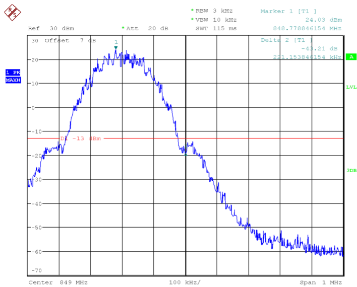
Channel 251- HIGH BAND EDGE BLOCK
