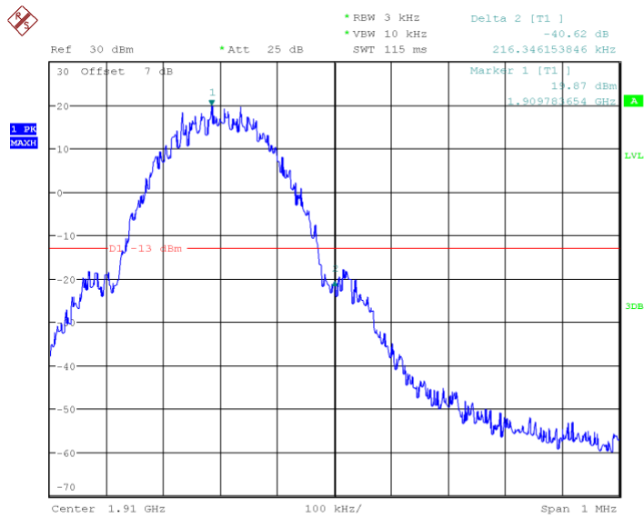
Channel 810- HIGH BAND EDGE BLOCK
