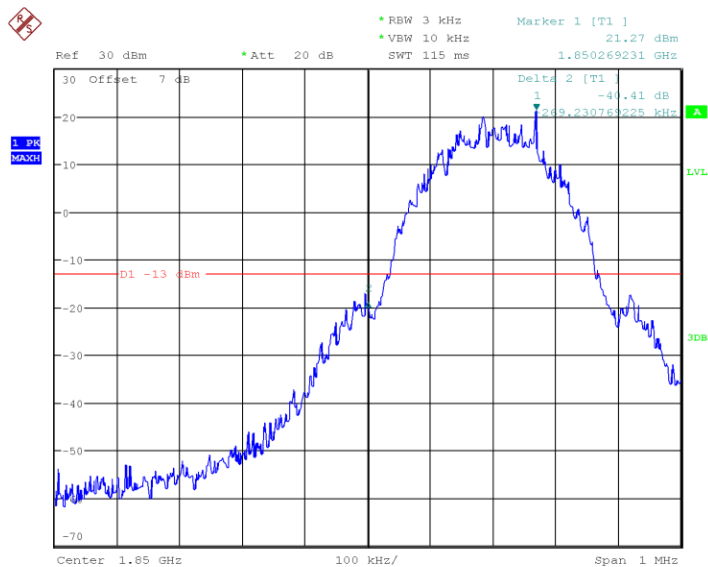
Channel 512- LOW BAND EDGE BLOCK
