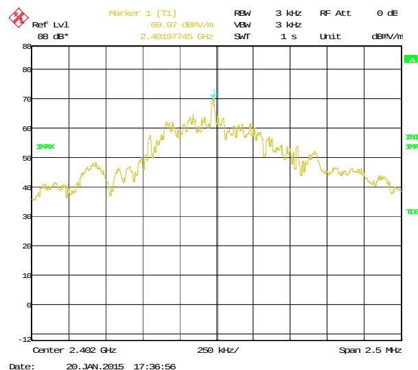
Figure 35 — Low Channel
