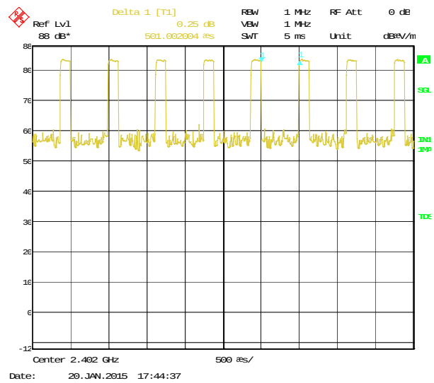
Figure 12. Number of bursts in 5msec=8 Number of bursts in 100msec=160
