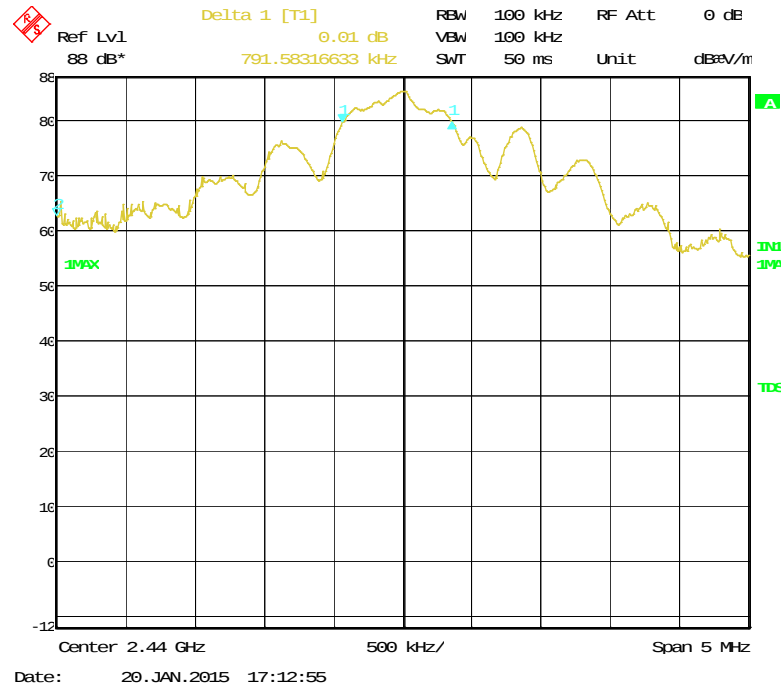
Figure 15. Mid Channel, BLE Modulation
