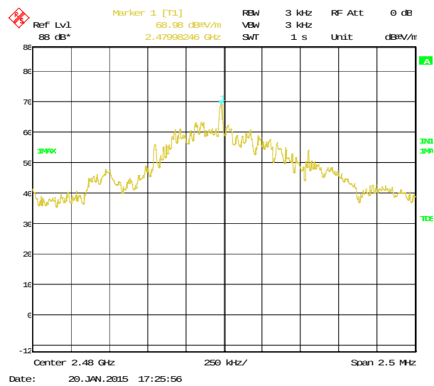
Figure 37 — High Channel
