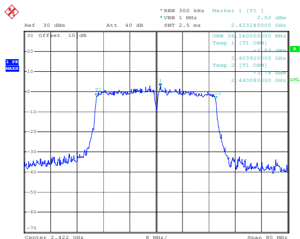
ANT 1(802.11n40)
