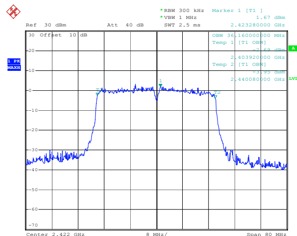
ANT 2(802.11n40)
