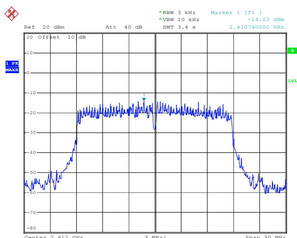
ANT 2(802.11 n20)
