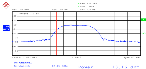
ANT 2(802.11b)
