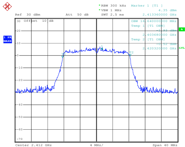
ANT 1(802.11g)
