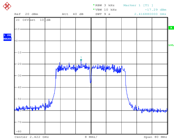
ANT 2(802.11n40)
