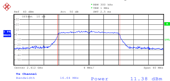
ANT 2(802.11g)
