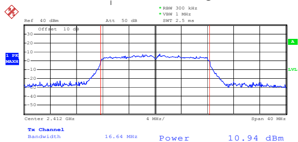
ANT 1(802.11g)
