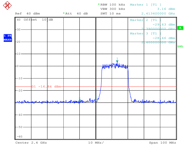
ANT 2(802.11g)
