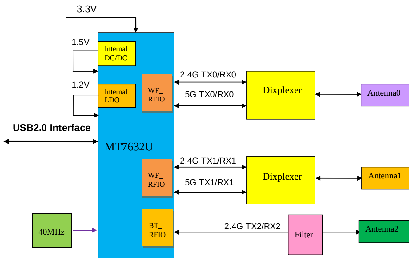
Figure 1 M632USA1 Block Diagram
