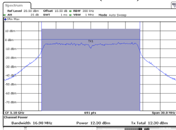
ANT 2(802.11A)
