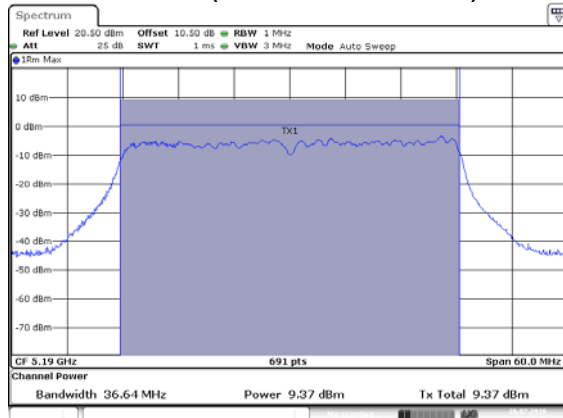
ANT 2(802.11 AC 40MHz)
