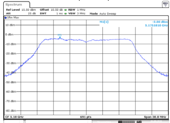
ANT 2(11N20)
