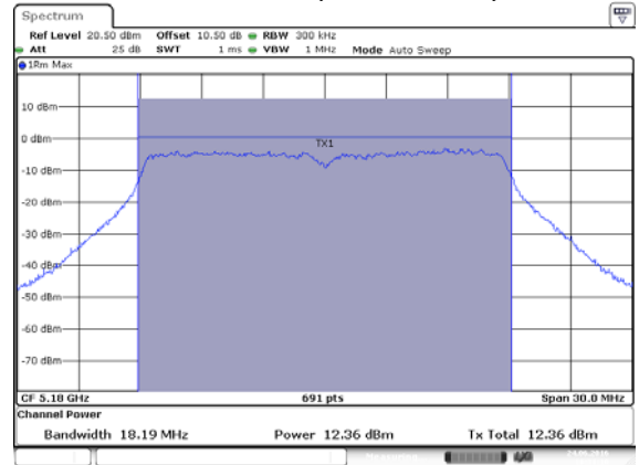
ANT 2(802.11 N20)
