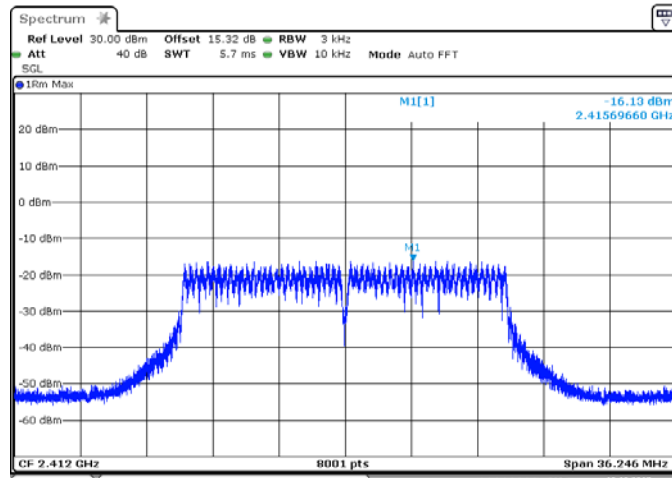
ANT 2(802.11 n20)
