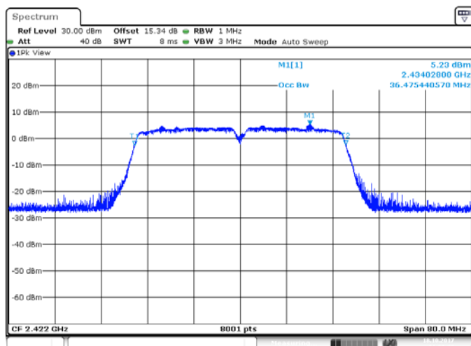
ANT 1(802.11n40)
