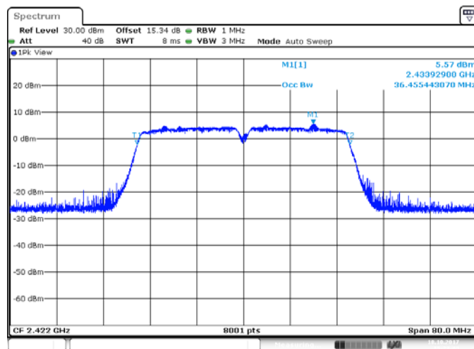
ANT 2(802.11n40)
