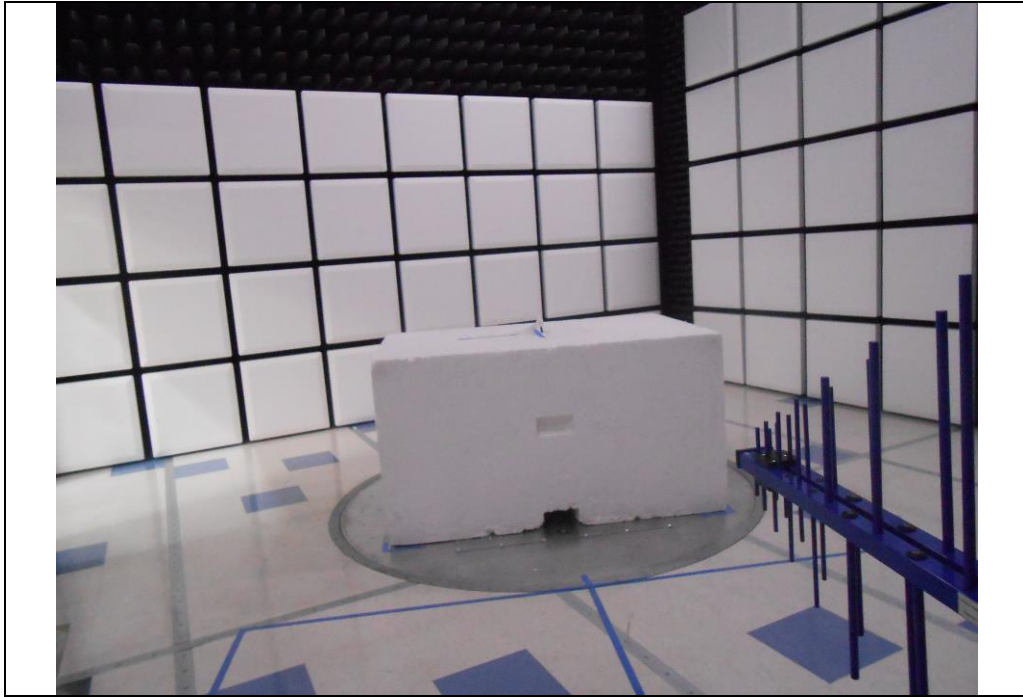
RF Radiated #2
