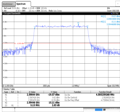
Band41-5MHz-QPSK-40620-25RB#0-PASS
