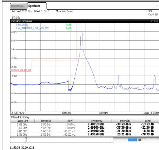
Band41-10MHz-QPSK-39700-50RB#0-PASS
