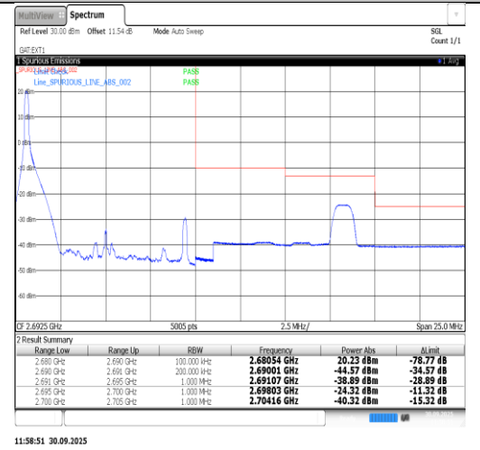
Band41-10MHz-QPSK-41540-50RB#0-PASS
