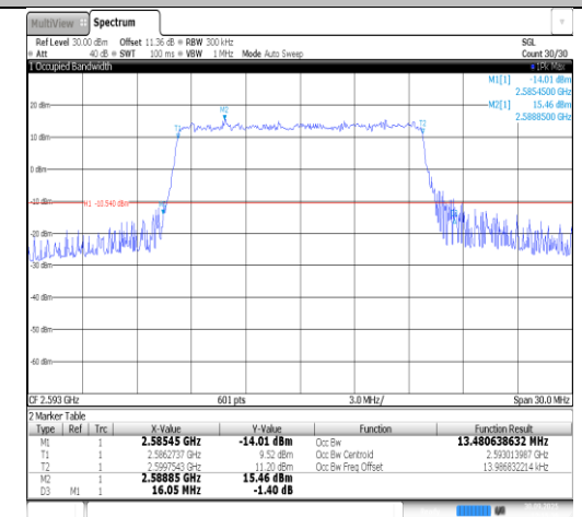
Band41-15MHz-16QAM-40620-75RB#0-PASS
