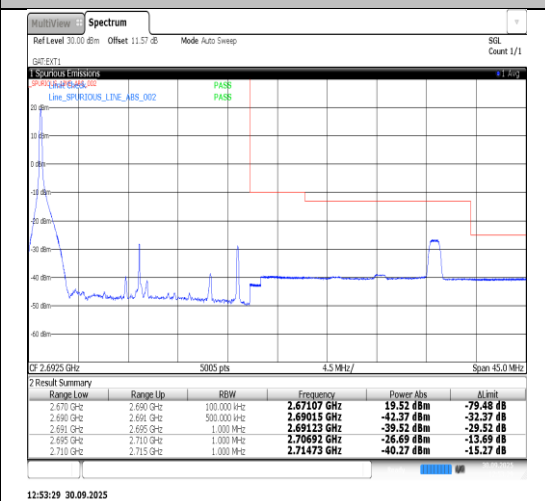
Band41-20MHz-16QAM-41490-100RB#0-PASS
