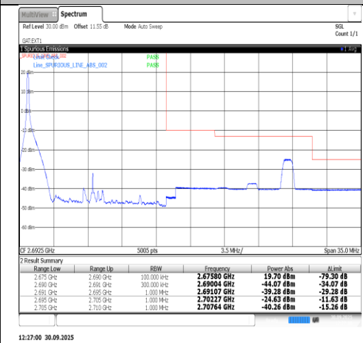
Band41-15MHz-16QAM-41515-75RB#0-PASS
