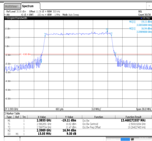
Band41-15MHz-QPSK-40620-75RB#0-PASS
