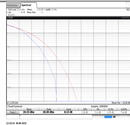
Band41-15MHz-16QAM-40620-75RB#0-PASS
