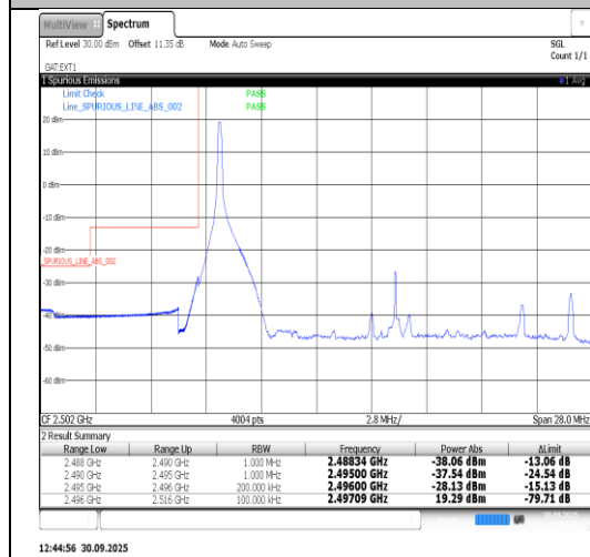
Band41-20MHz-16QAM-39750-100RB#0-PASS
