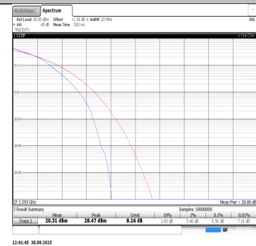
Band41-20MHz-16QAM-40620-100RB#0-PASS
