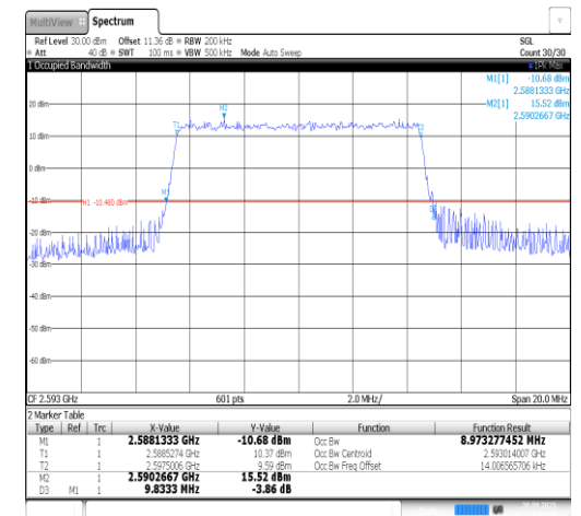
Band41-10MHz-16QAM-40620-50RB#0-PASS
