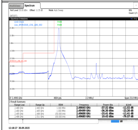
Band41-15MHz-16QAM-39725-75RB#0-PASS
