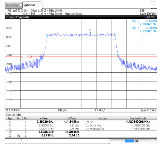
Band41-5MHz-16QAM-40620-25RB#0-PASS
