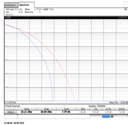
Band41-10MHz-16QAM-40620-50RB#0-PASS
