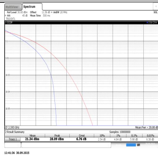
Band41-15MHz-QPSK-40620-75RB#0-PASS
