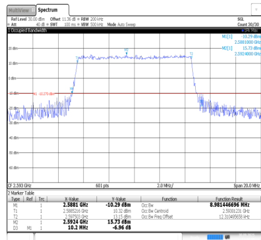
Band41-10MHz-QPSK-40620-50RB#0-PASS
