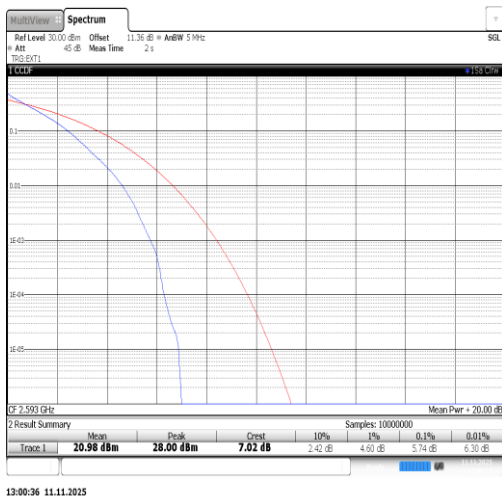
Band41-10MHz-QPSK-40620-50RB#0-PASS
