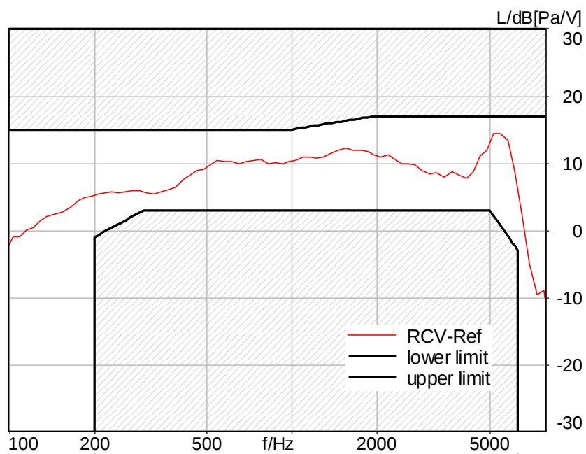
Figure C.3-16 – LTE Band 12 8N FF Wideband Frequency Response
