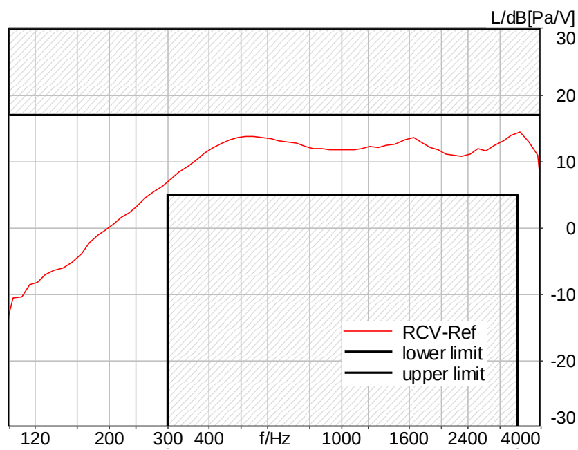
Figure C.3-34 – LTE Band 41 8N FF Narrowband Frequency Response
