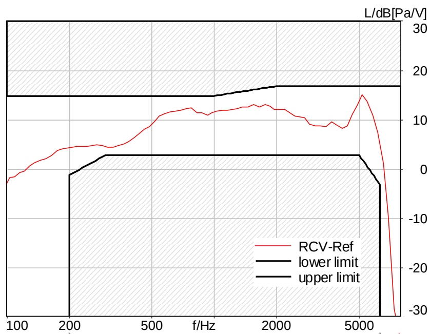
Figure C.2-12 – WCDMA Band V 8N FF Wideband Frequency Response
