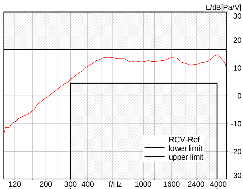
Figure C.3-22 – LTE Band 17 8N FF Narrowband Frequency Response
