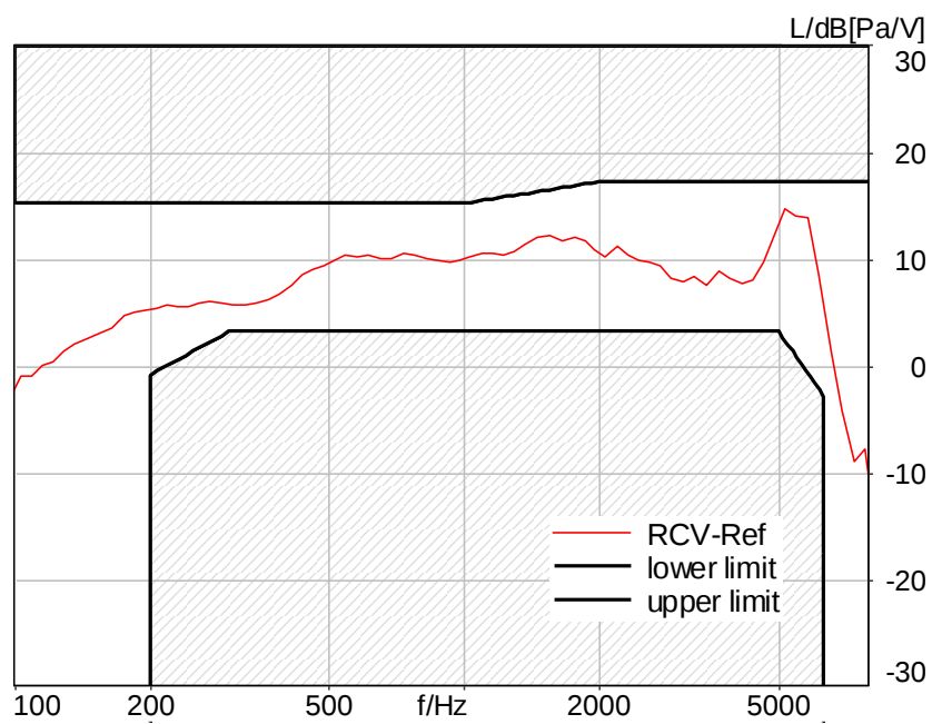
Figure C.3-8 – LTE Band 4 8N FF Wideband Frequency Response
