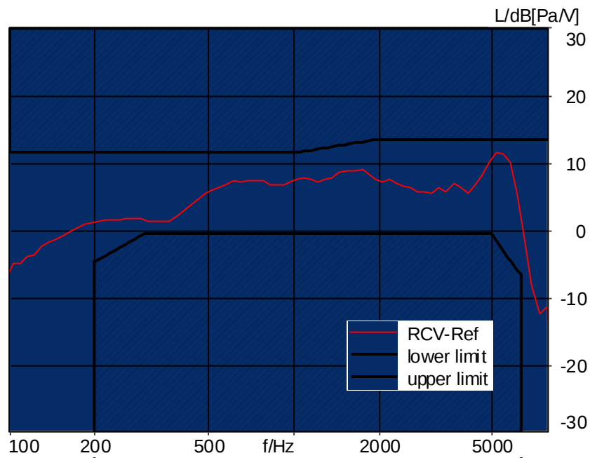
Figure C.4-15 – WLAN UNII-2C 2N FF Wideband Frequency Response
