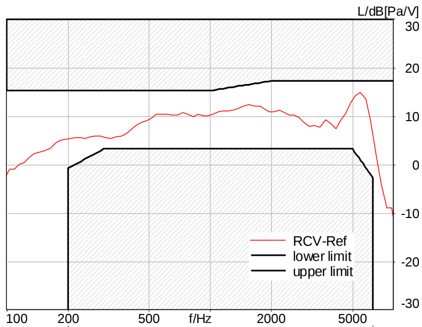
Figure C.3-32 – LTE Band 26 8N FF Wideband Frequency Response
