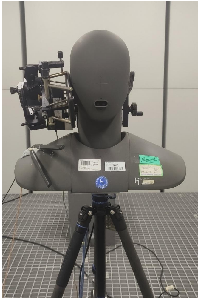
Figure E-1 – Test Layout (Handset)
