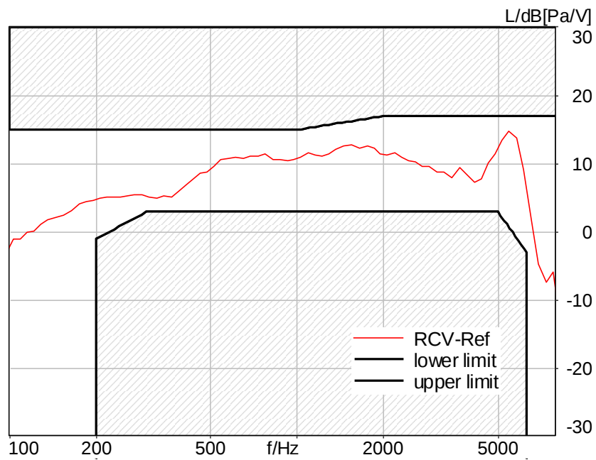
Figure C.3-44 – LTE Band 71 8N FF Wideband Frequency Response
