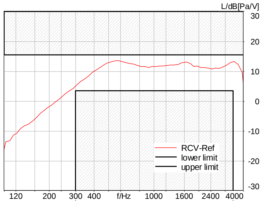
Figure C.4-2 – WLAN 2.4GHz 8N FF Narrowband Frequency Response
