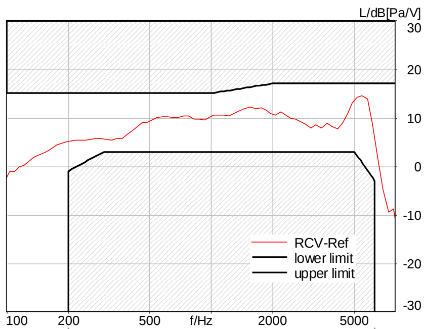
Figure C.3-24 – LTE Band 17 8N FF Wideband Frequency Response
