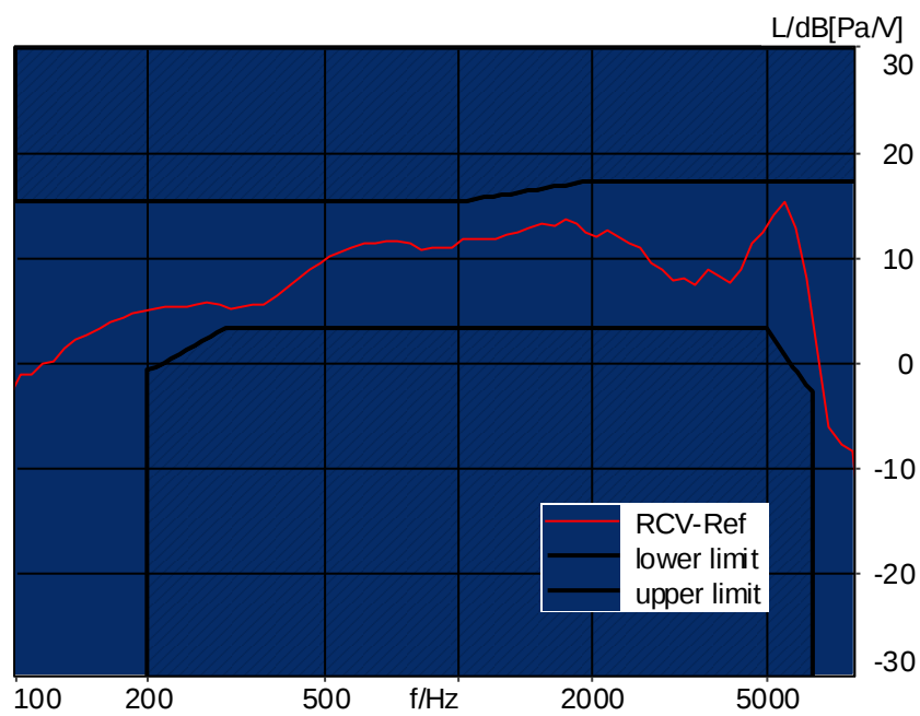
Figure C.4-16 – WLAN UNII-2C 8N FF Wideband Frequency Response
