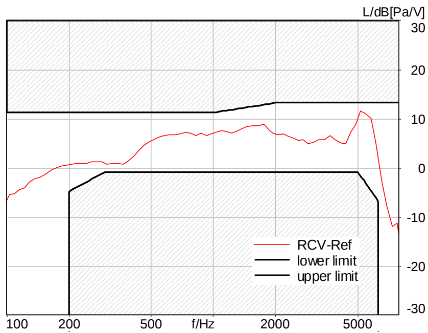
Figure C.4-19 – WLAN UNII-3 2N FF Wideband Frequency Response
