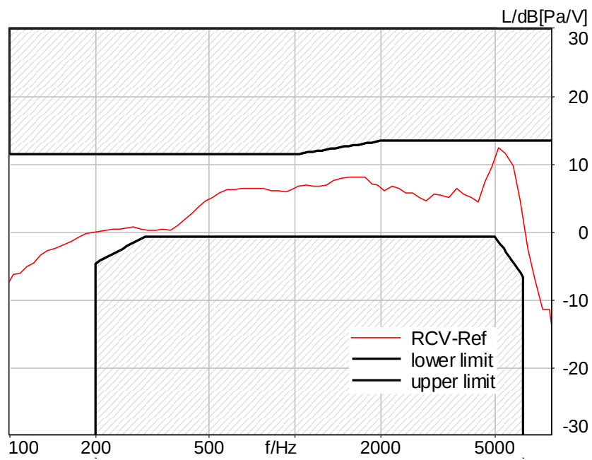
Figure C.4-7 – WLAN UNII-1 2N FF Wideband Frequency Response
