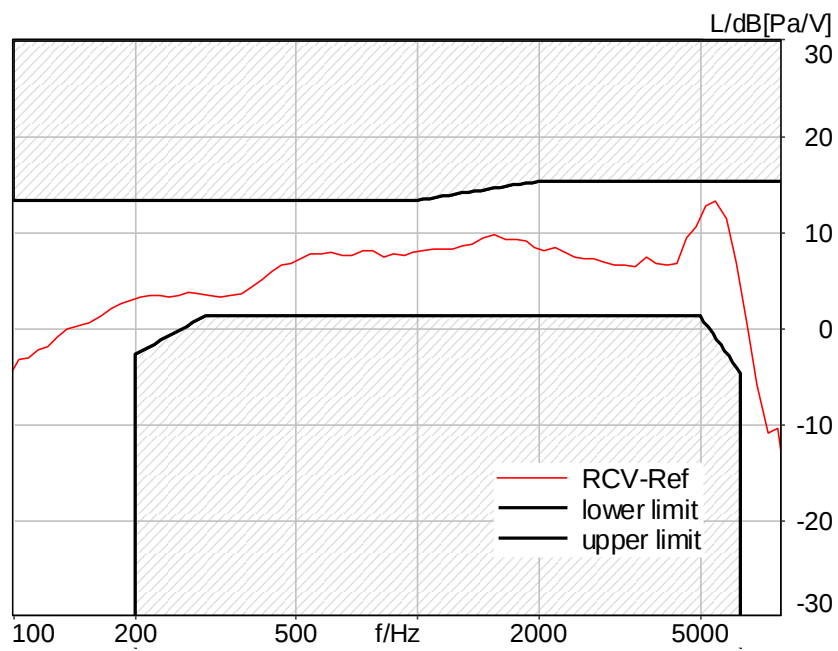
Figure C.3-3 – LTE Band 2 2N FF Wideband Frequency Response
