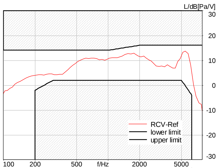
Figure C.4-12 – WLAN UNII-2A 8N FF Wideband Frequency Response
