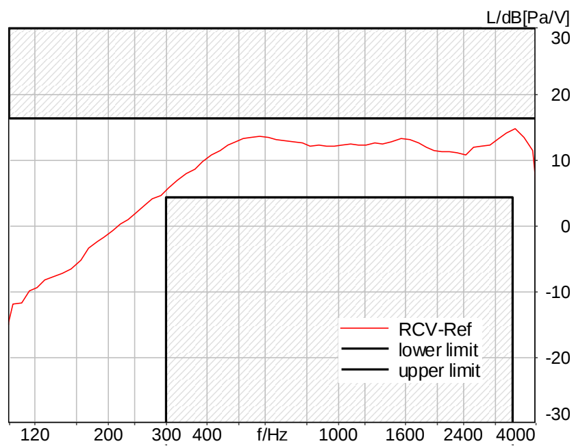
Figure C.3-14 – LTE Band 12 8N FF Narrowband Frequency Response
