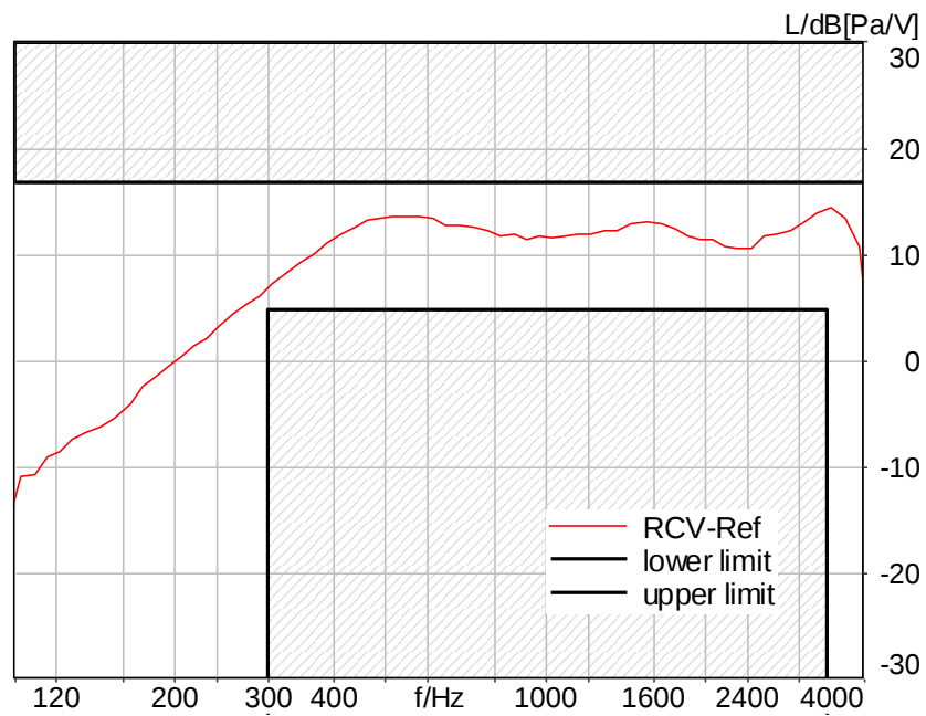
Figure C.3-42 – LTE Band 71 8N FF Narrowband Frequency Response
