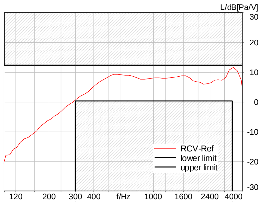
Figure C.4-5 – WLAN UNII-1 2N FF Narrowband Frequency Response
