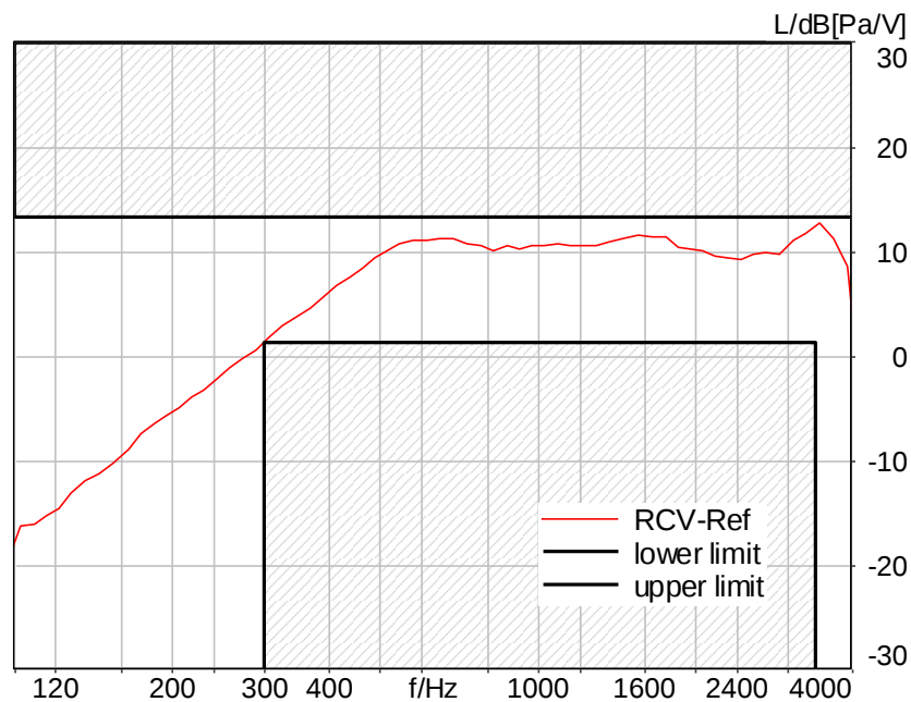
Figure C.1-2 – GSM850 8N FF Narrowband Frequency Response
