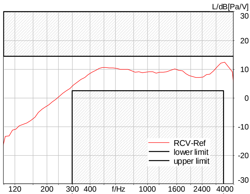
Figure C.3-33 – LTE Band 41 2N FF Narrowband Frequency Response
