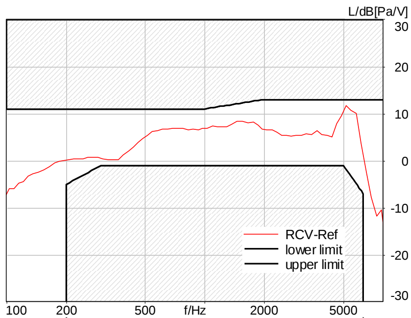
Figure C.4-11 – WLAN UNII-2A 2N FF Wideband Frequency Response
