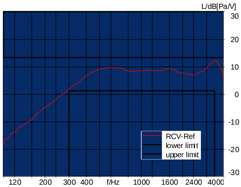
Figure C.4-13 – WLAN UNII-2C 2N FF Narrowband Frequency Response
