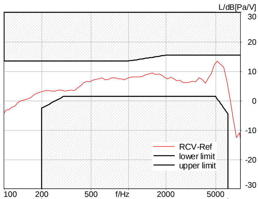
Figure C.3-27 – LTE Band 25 2N FF Wideband Frequency Response
