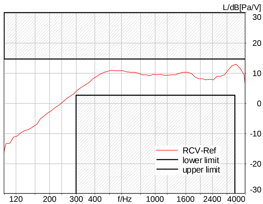
Figure C.3-37 – LTE Band 66 2N FF Narrowband Frequency Response
