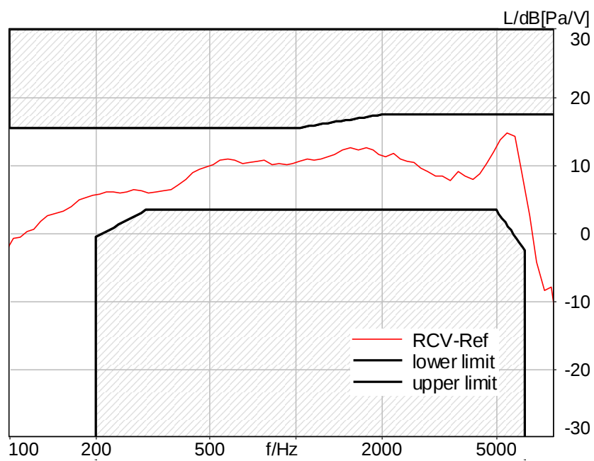
Figure C.3-4 – LTE Band 2 8N FF Wideband Frequency Response
