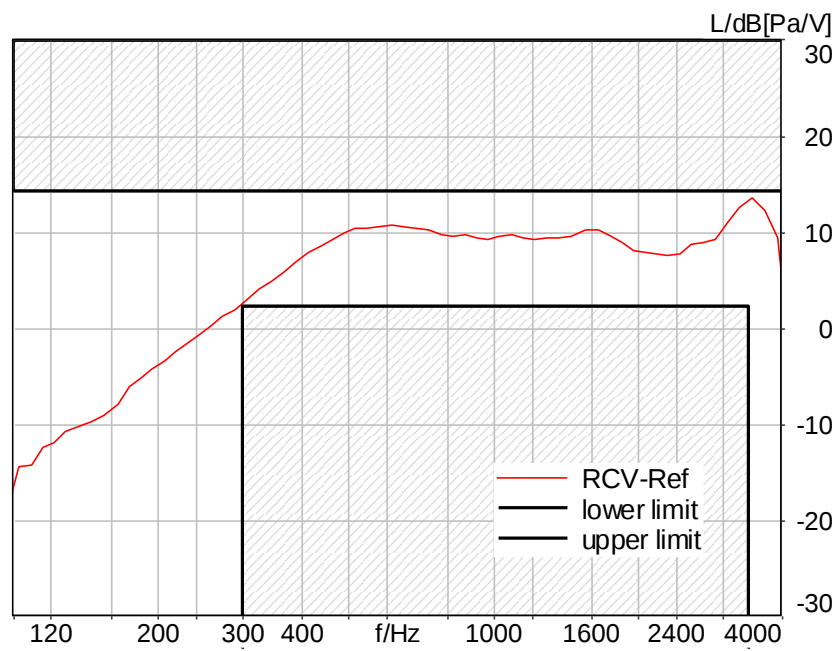
Figure C.3-13 – LTE Band 12 2N FF Narrowband Frequency Response
