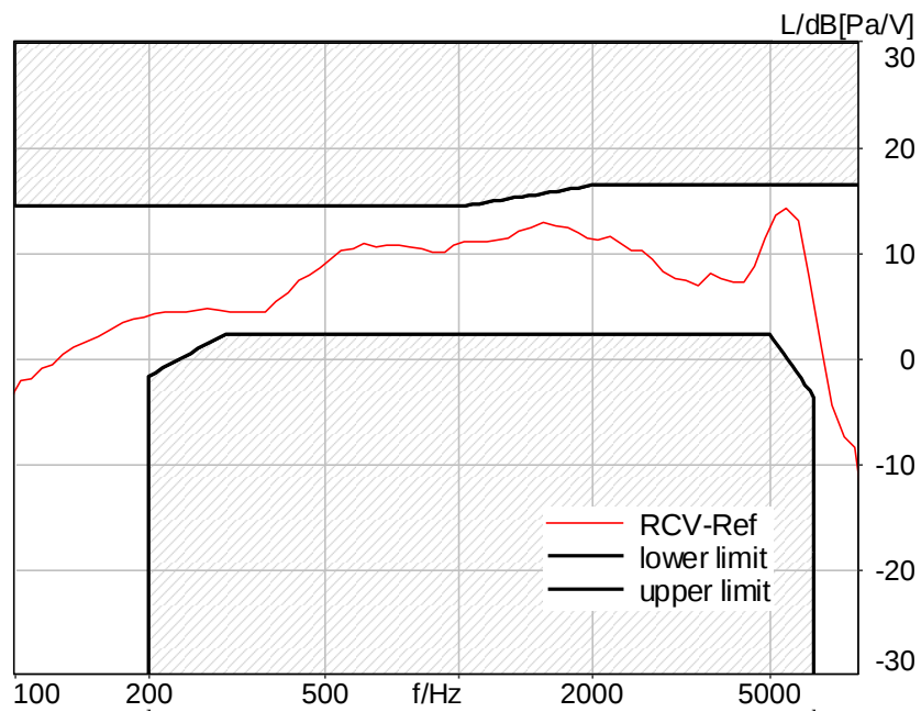
Figure C.4-8 – WLAN UNII-1 8N FF Wideband Frequency Response
