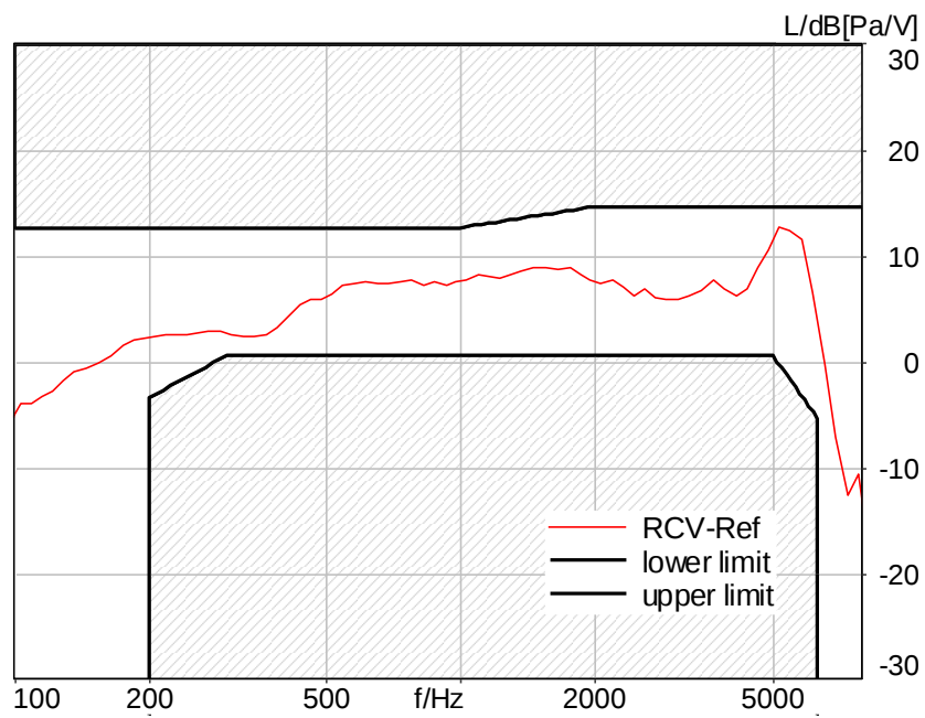
Figure C.3-19 – LTE Band 13 2N FF Wideband Frequency Response
