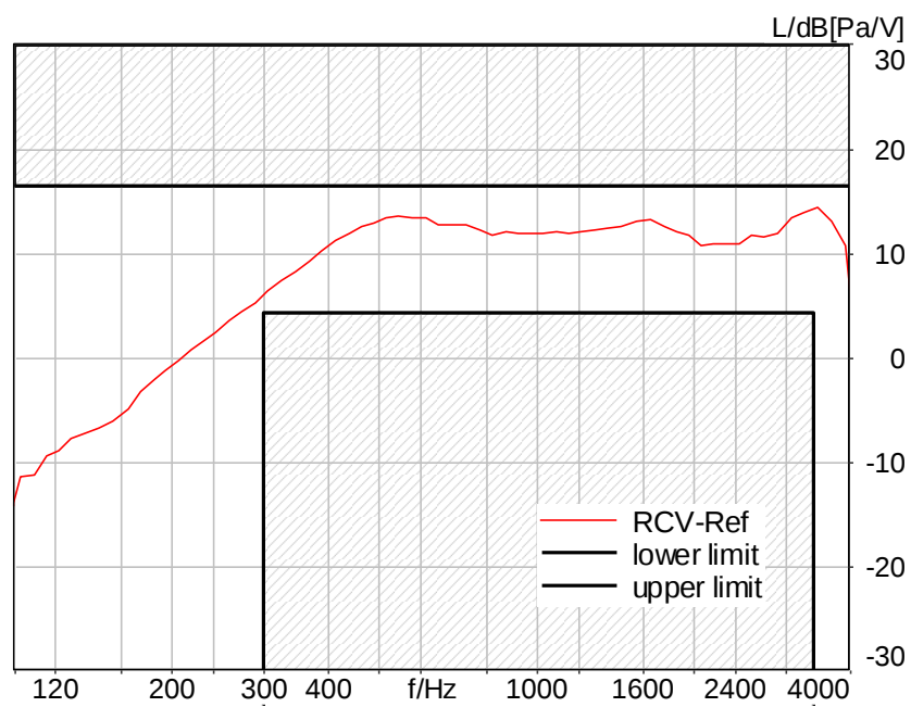
Figure C.3-30 – LTE Band 26 8N FF Narrowband Frequency Response
