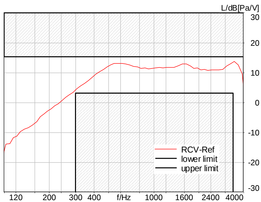
Figure C.4-10 – WLAN UNII-2A 8N FF Narrowband Frequency Response
