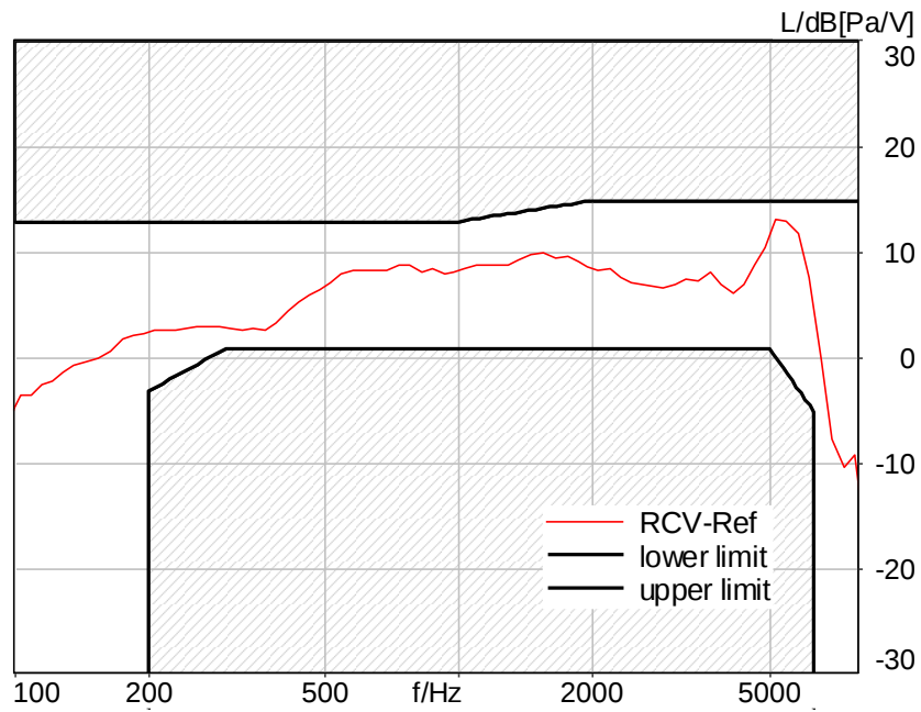
Figure C.3-35 – LTE Band 41 2N FF Wideband Frequency Response
