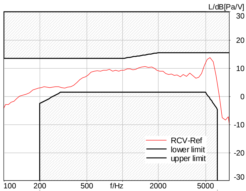
Figure C.3-39 – LTE Band 66 2N FF Wideband Frequency Response
