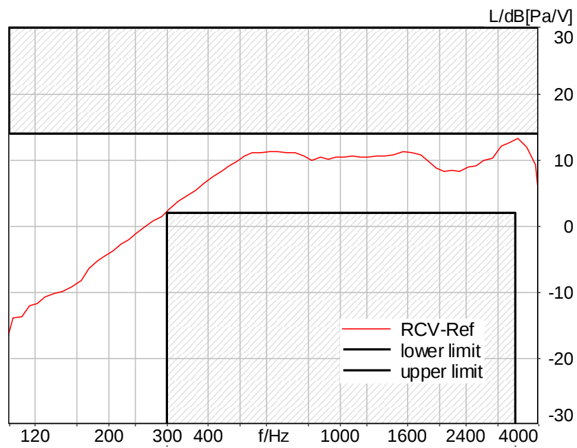
Figure C.2-5 – WCDMA Band IV 2N FF Narrowband Frequency Response
