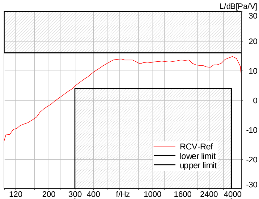
Figure C.2-2 – WCDMA Band II 8N FF Narrowband Frequency Response
