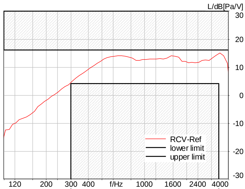
Figure C.2-10 – WCDMA Band V 8N FF Narrowband Frequency Response
