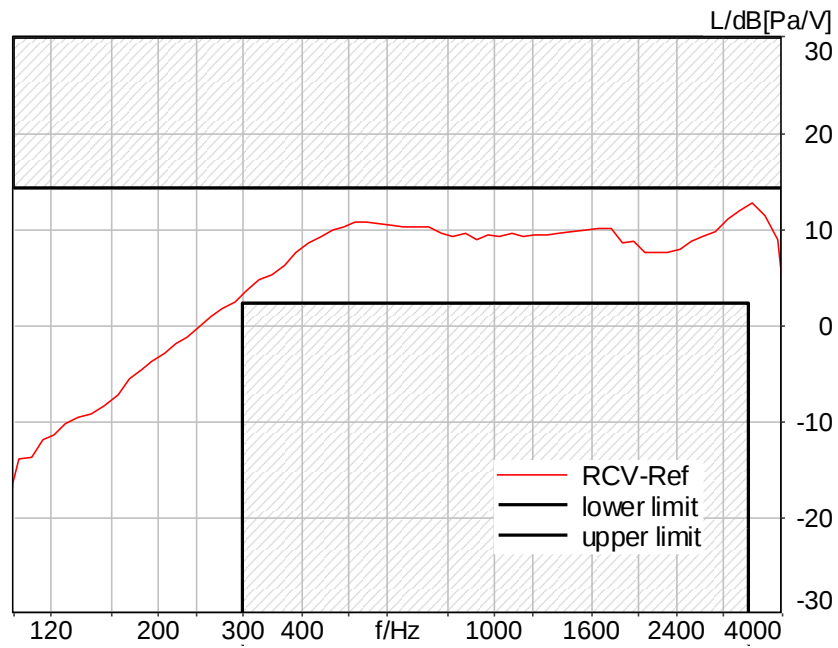
Figure C.3-9 – LTE Band 5 2N FF Narrowband Frequency Response
