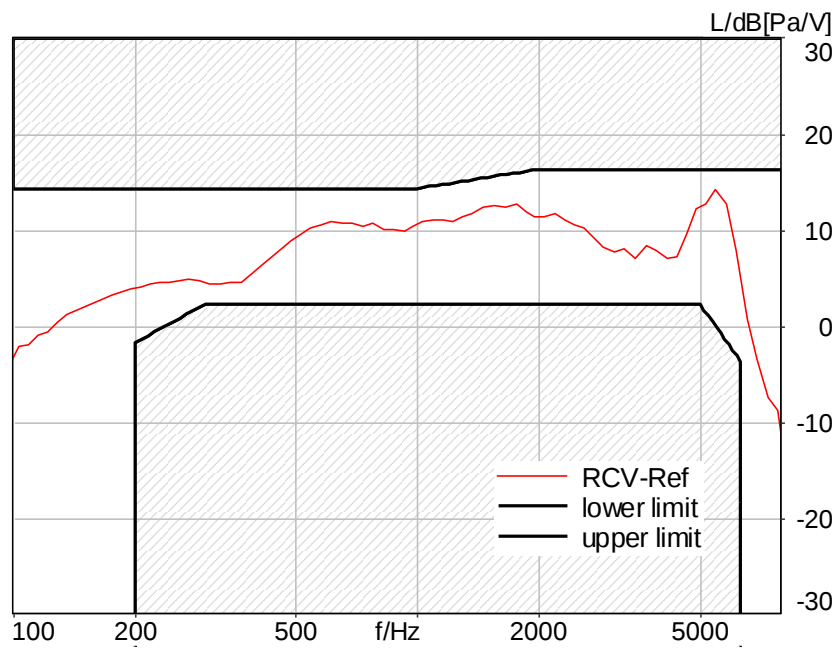
Figure C.4-4 – WLAN 2.4GHz 8N FF Wideband Frequency Response
