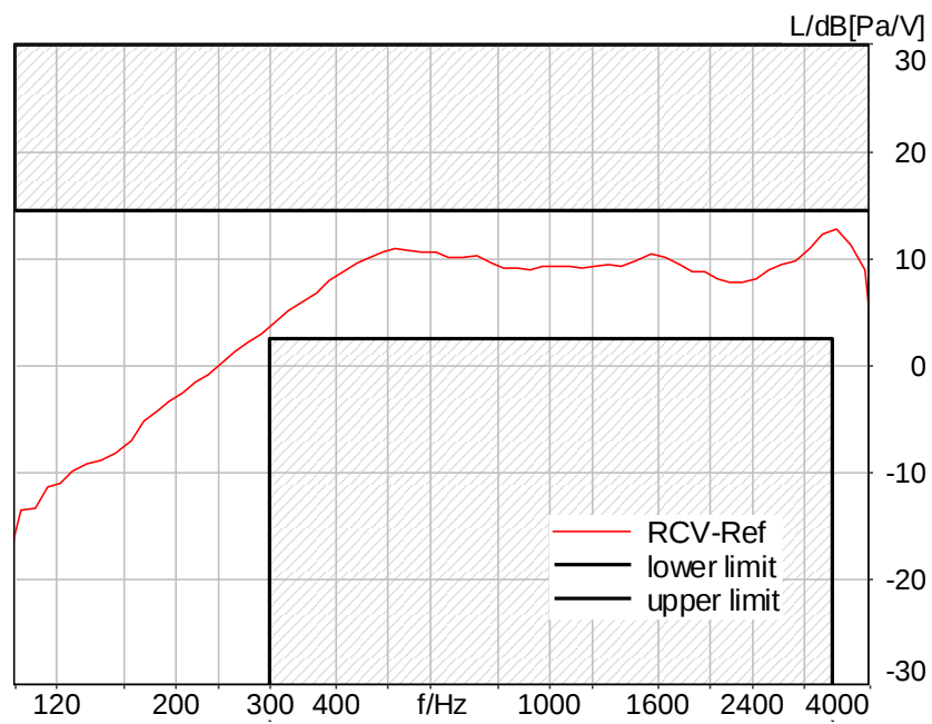
Figure C.3-5 – LTE Band 4 2N FF Narrowband Frequency Response
