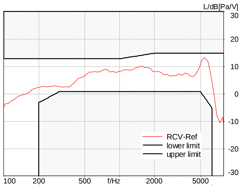
Figure C.3-43 – LTE Band 71 2N FF Wideband Frequency Response
