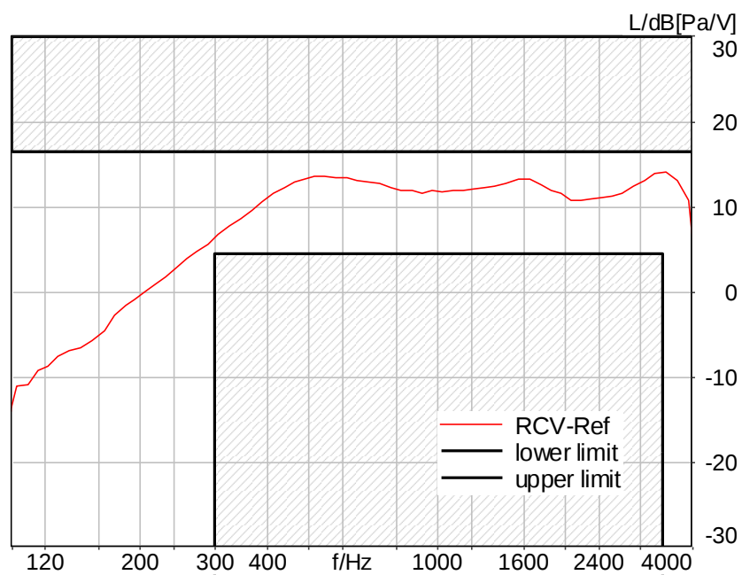
Figure C.3-38 – LTE Band 66 8N FF Narrowband Frequency Response
