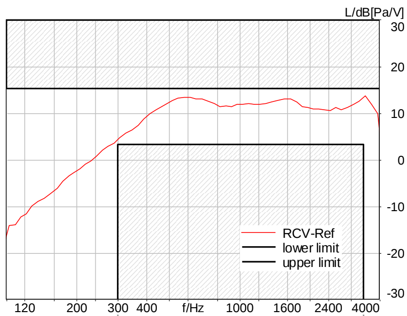
Figure C.4-6 – WLAN 2 UNII-1 8N FF Narrowband Frequency Response
