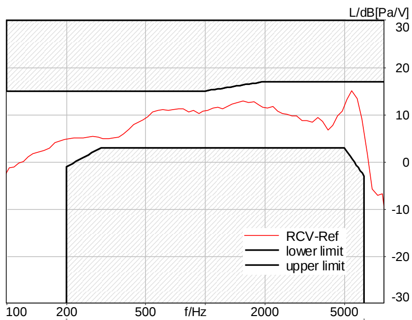
Figure C.3-40 – LTE Band 66 8N FF Wideband Frequency Response
