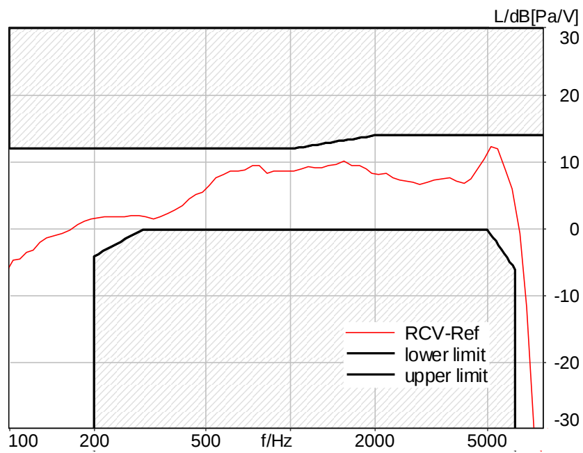
Figure C.2-11 – WCDMA Band V 2N FF Wideband Frequency Response
