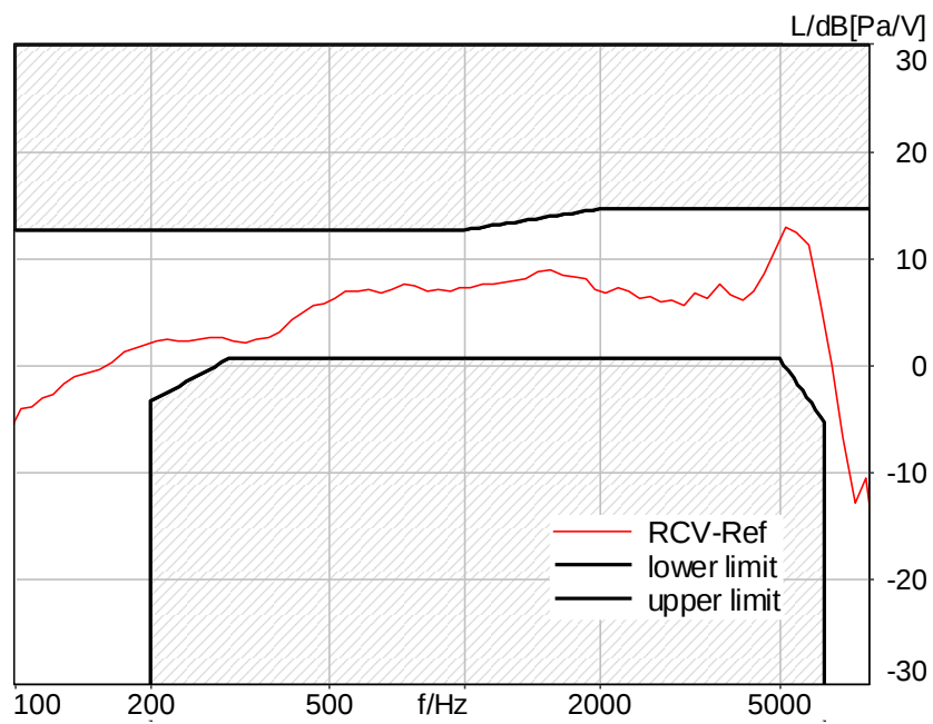
Figure C.3-15 – LTE Band 12 2N FF Wideband Frequency Response
