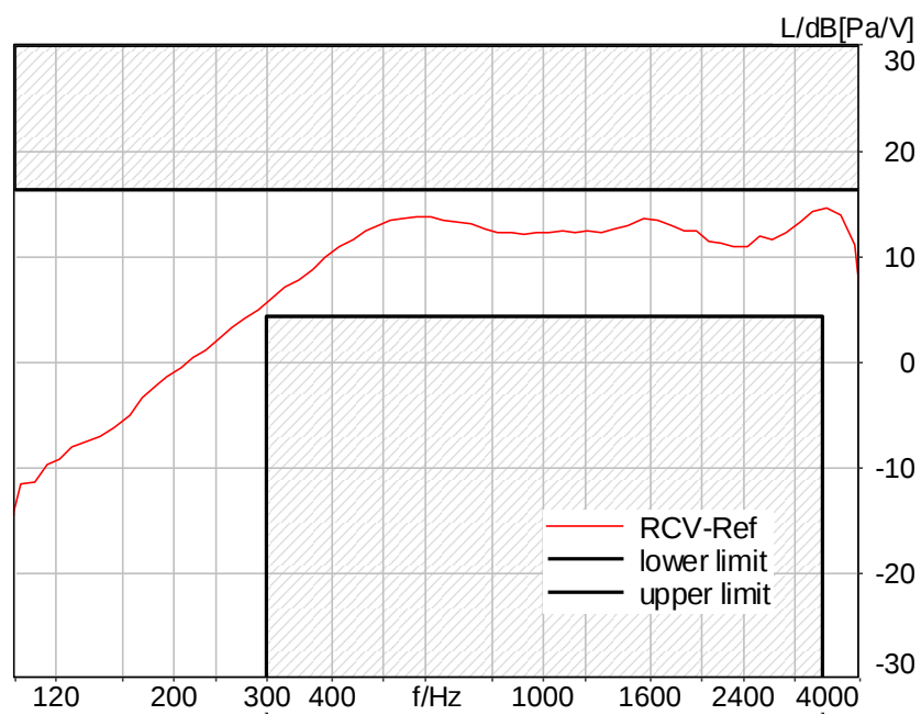
Figure C.3-18 – LTE Band 13 8N FF Narrowband Frequency Response
