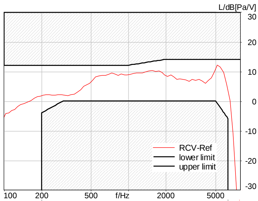
Figure C.2-3 – WCDMA Band II 2N FF Wideband Frequency Response
