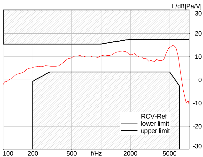
Figure C.3-28 – LTE Band 25 8N FF Wideband Frequency Response
