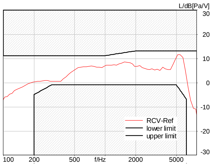
Figure C.4-3 – WLAN 2.4GHz 2N FF Wideband Frequency Response
