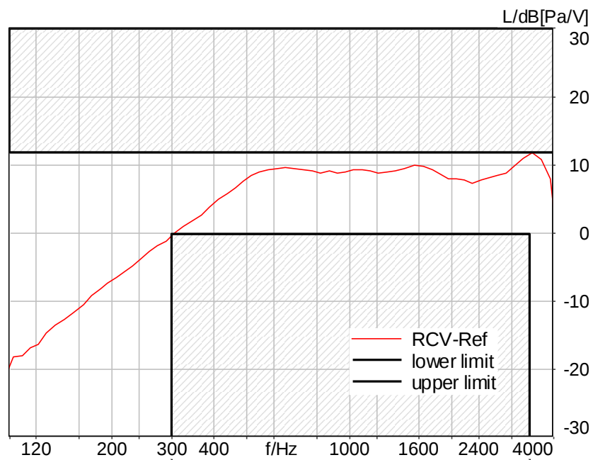
Figure C.1-3 – GSM1900 2N FF Narrowband Frequency Response
