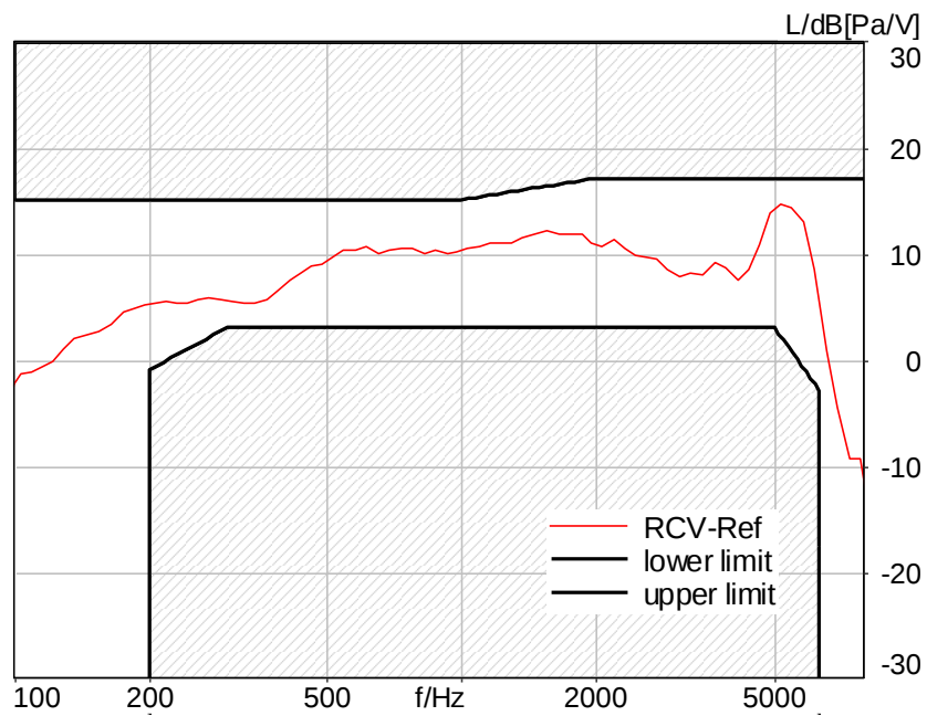
Figure C.3-20 – LTE Band 13 8N FF Wideband Frequency Response
