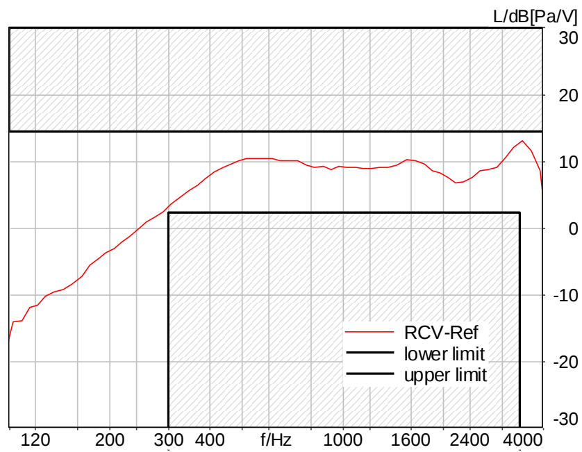
Figure C.3-29 – LTE Band 26 2N FF Narrowband Frequency Response
