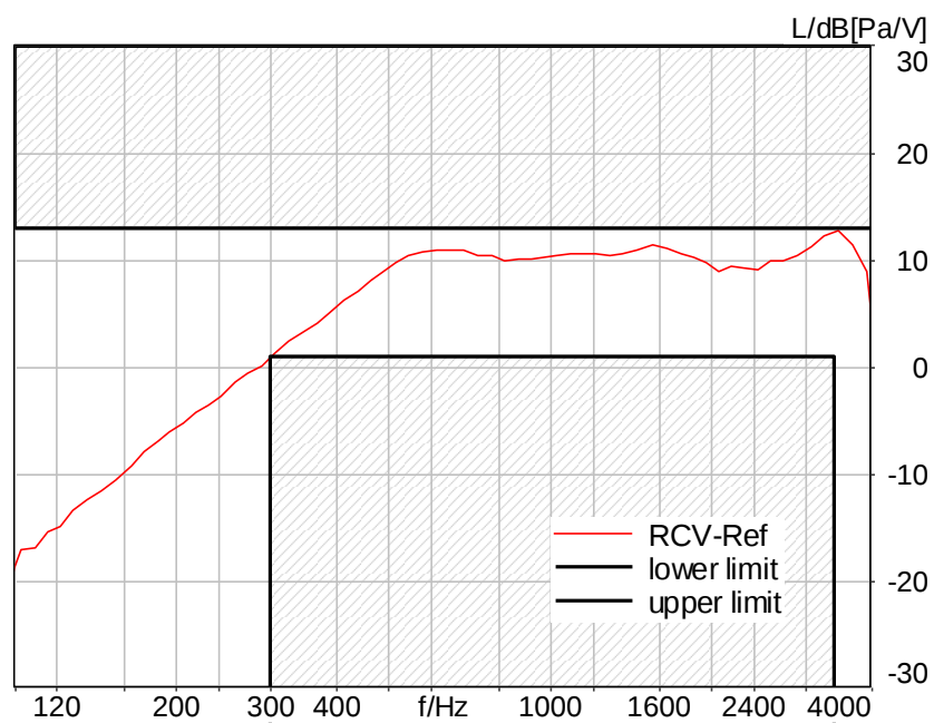
Figure C.1-4 – GSM1900 8N FF Narrowband Frequency Response
