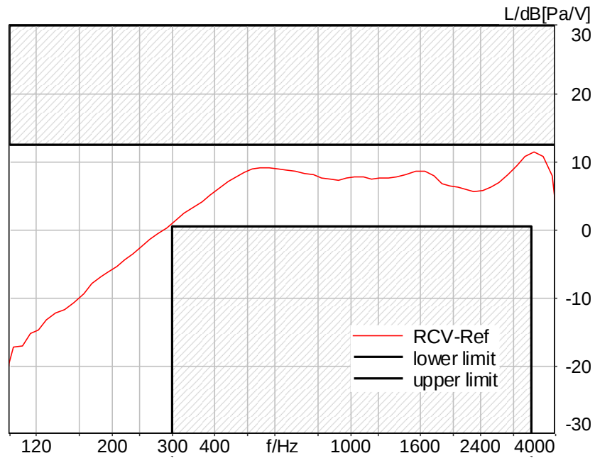
Figure C.4-1 – WLAN 2.4GHz 2N FF Narrowband Frequency Response
