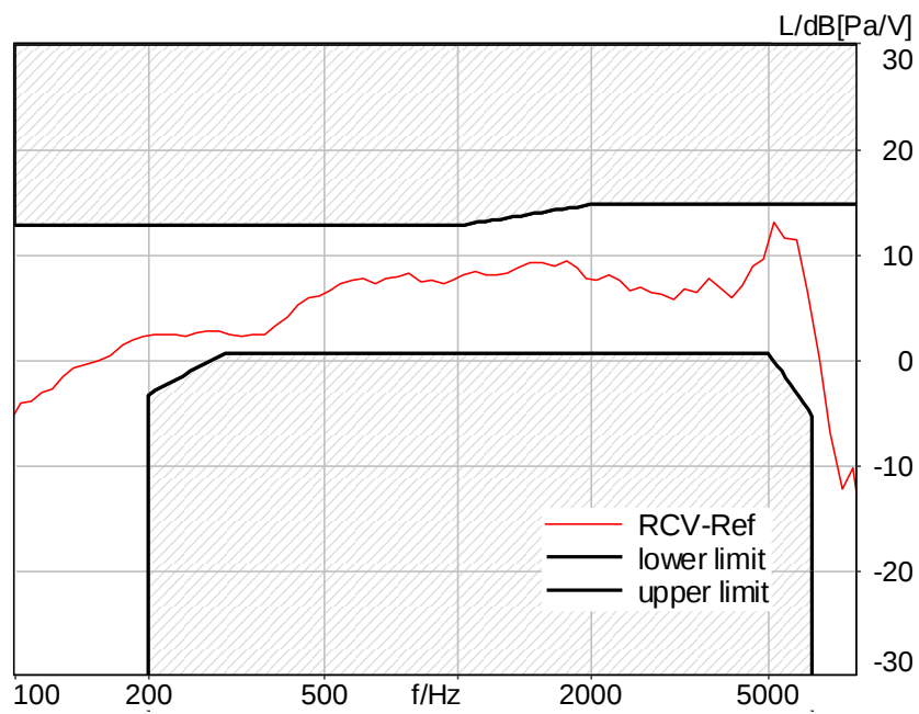
Figure C.3-11 – LTE Band 5 2N FF Wideband Frequency Response
