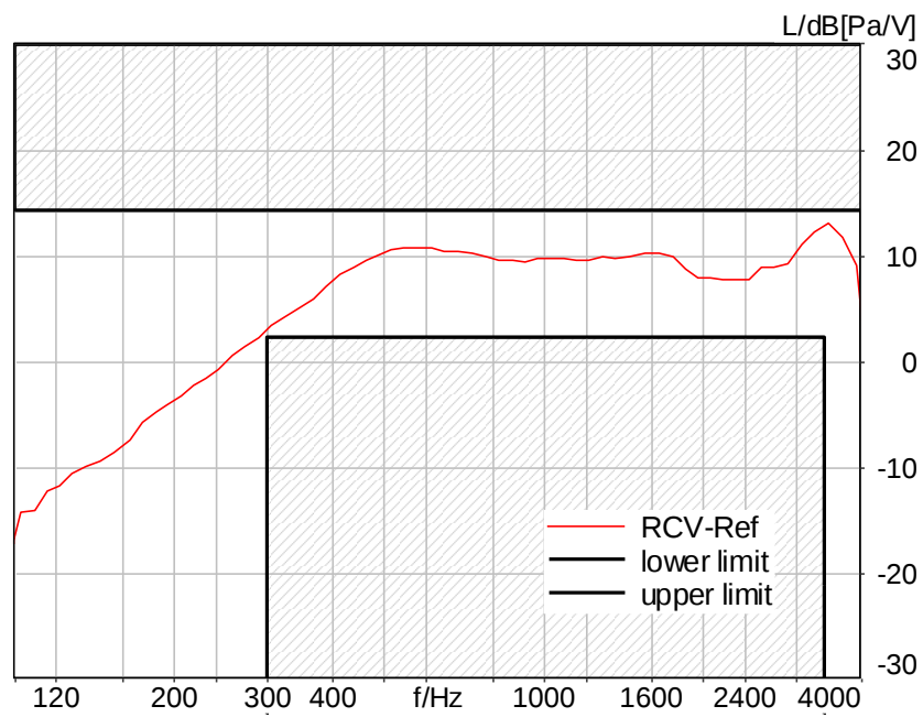
Figure C.3-21 – LTE Band 17 2N FF Narrowband Frequency Response
