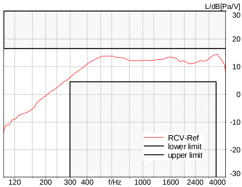
Figure C.3-26 – LTE Band 25 8N FF Narrowband Frequency Response
