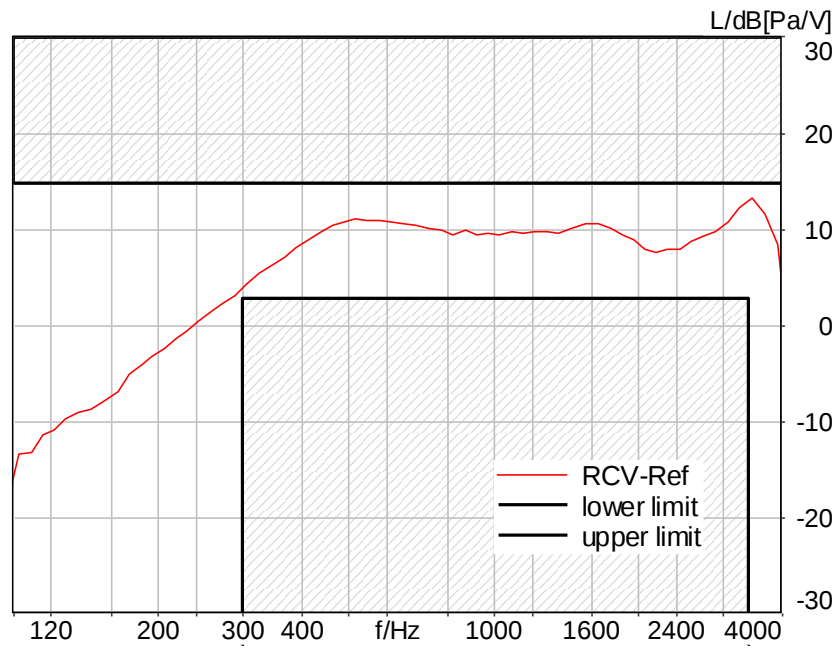
Figure C.3-25 – LTE Band 25 2N FF Narrowband Frequency Response
