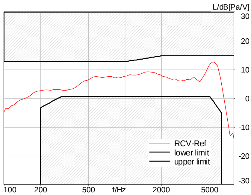
Figure C.3-31 – LTE Band 26 2N FF Wideband Frequency Response
