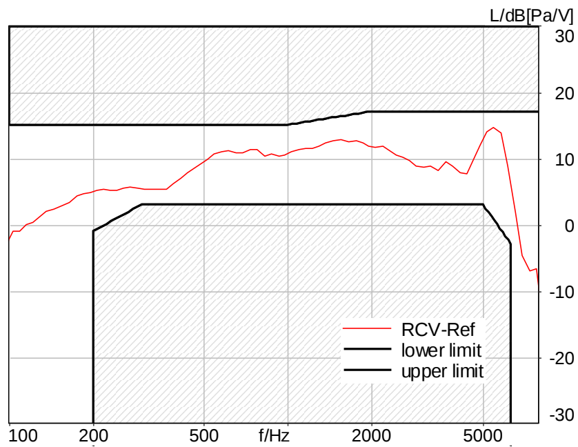
Figure C.3-36 – LTE Band 41 8N FF Wideband Frequency Response
