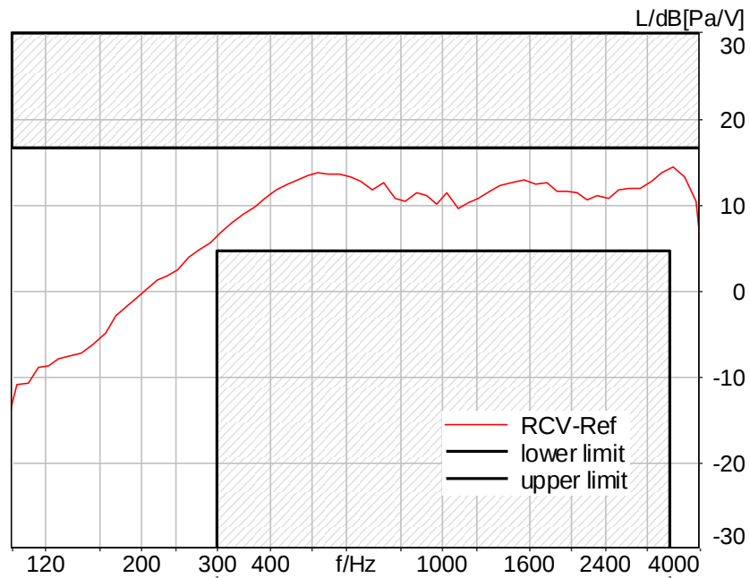
Figure C.3-2 – LTE Band 2 8N FF Narrowband Frequency Response
