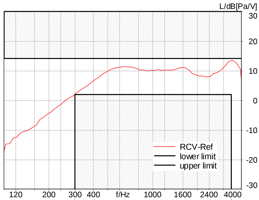
Figure C.2-9 – WCDMA Band V 2N FF Narrowband Frequency Response
