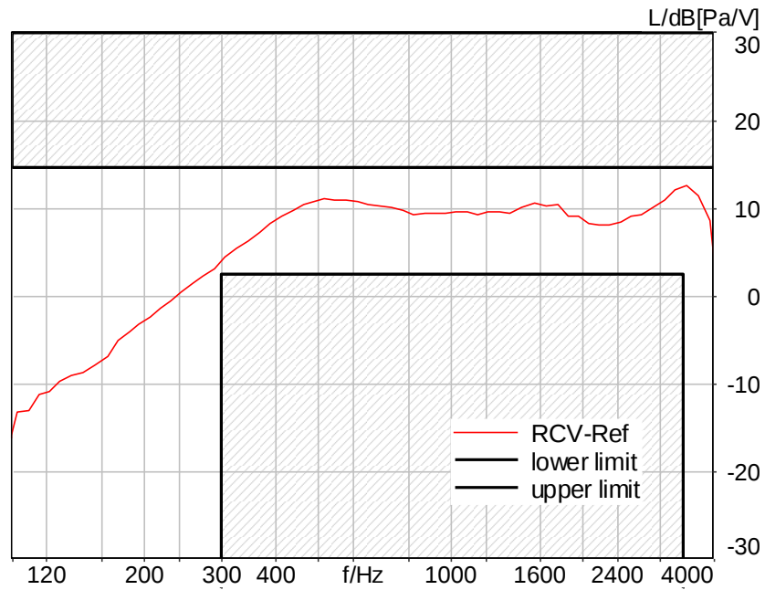
Figure C.3-1 – LTE Band 2 2N FF Narrowband Frequency Response
