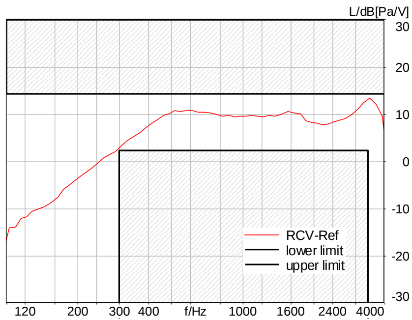
Figure C.3-17 – LTE Band 13 2N FF Narrowband Frequency Response
