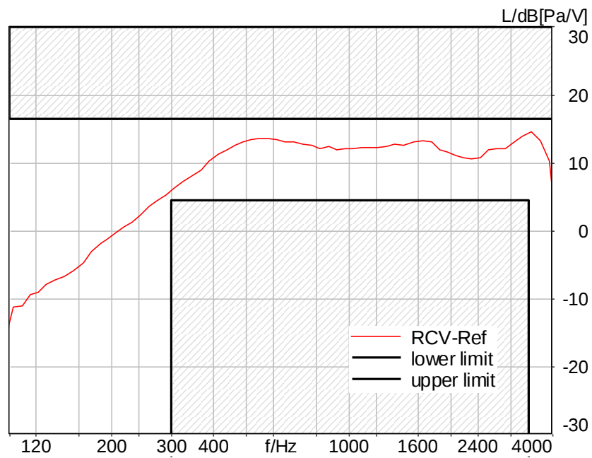
Figure C.3-10 – LTE Band 5 8N FF Narrowband Frequency Response
