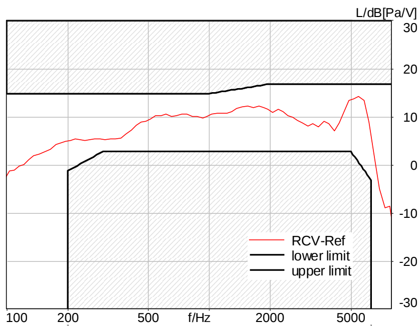
Figure C.3-12 – LTE Band 5 8N FF Wideband Frequency Response
