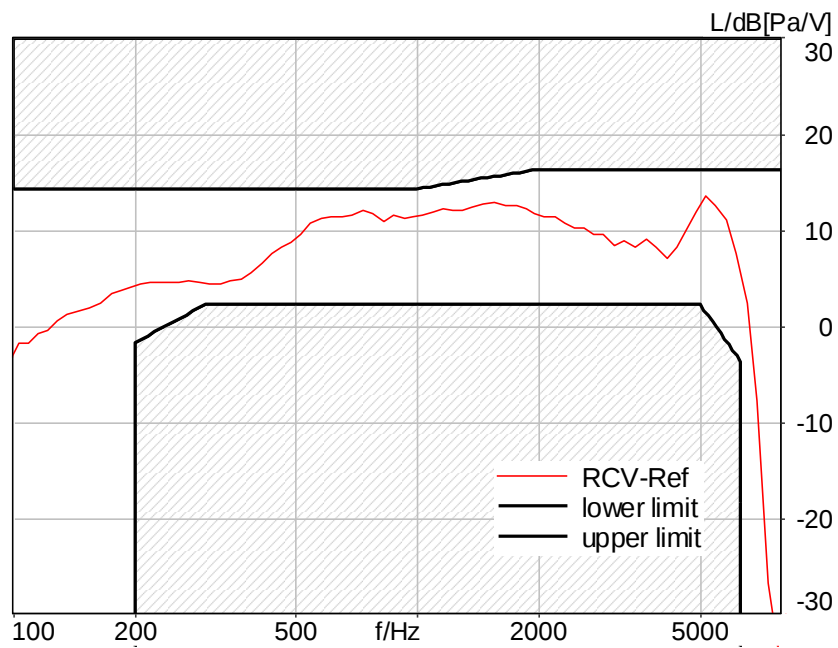
Figure C.2-4 – WCDMA Band II 8N FF Wideband Frequency Response
