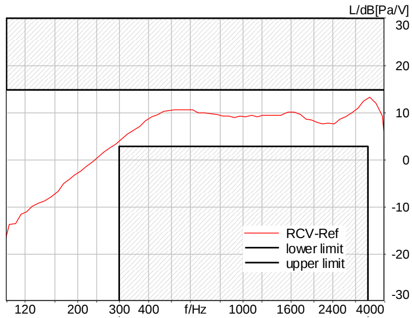
Figure C.3-41 – LTE Band 71 2N FF Narrowband Frequency Response
