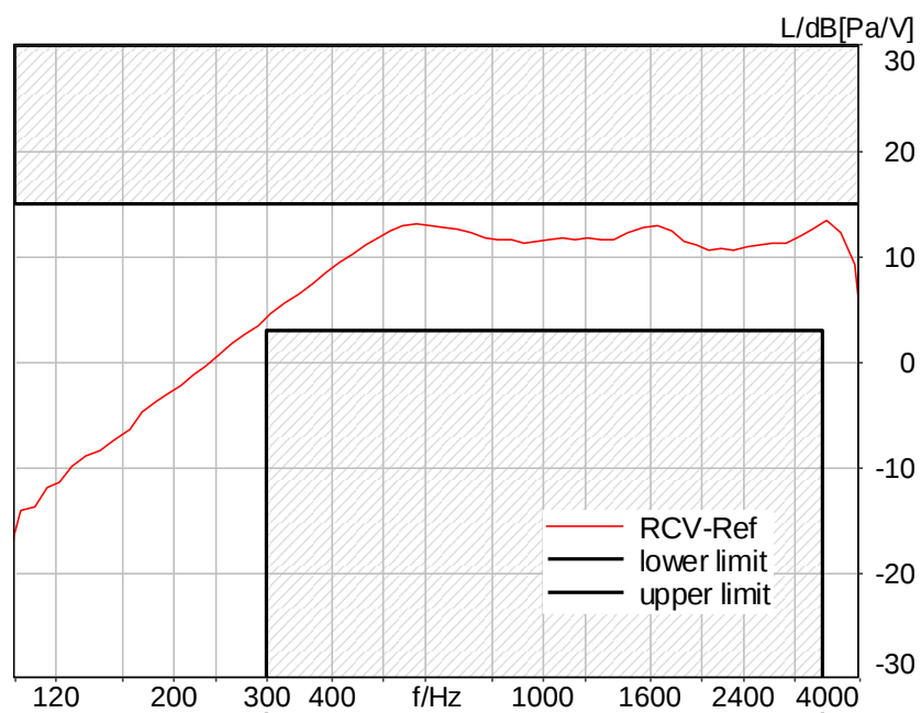
Figure C.4-18 – WLAN UNII-3 8N FF Narrowband Frequency Response
