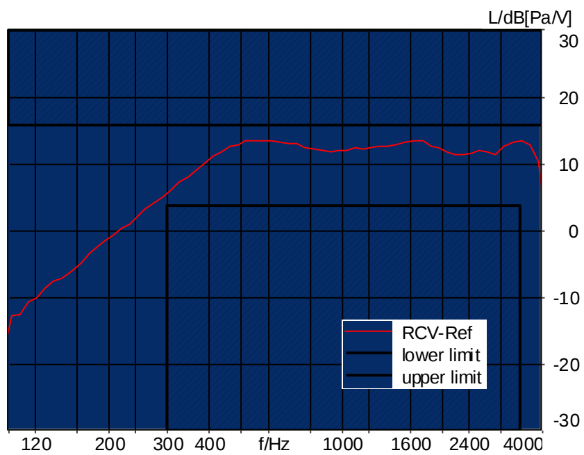
Figure C.4-14 – WLAN UNII-2C 8N FF Narrowband Frequency Response
