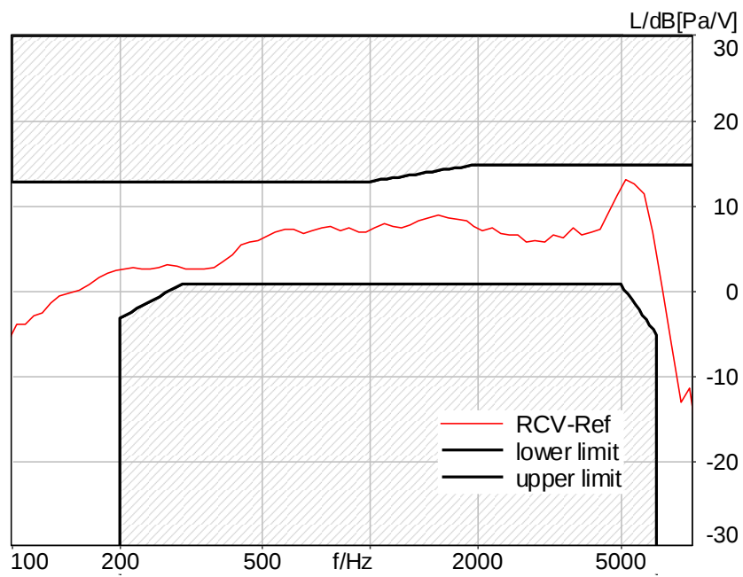
Figure C.3-23 – LTE Band 17 2N FF Wideband Frequency Response
