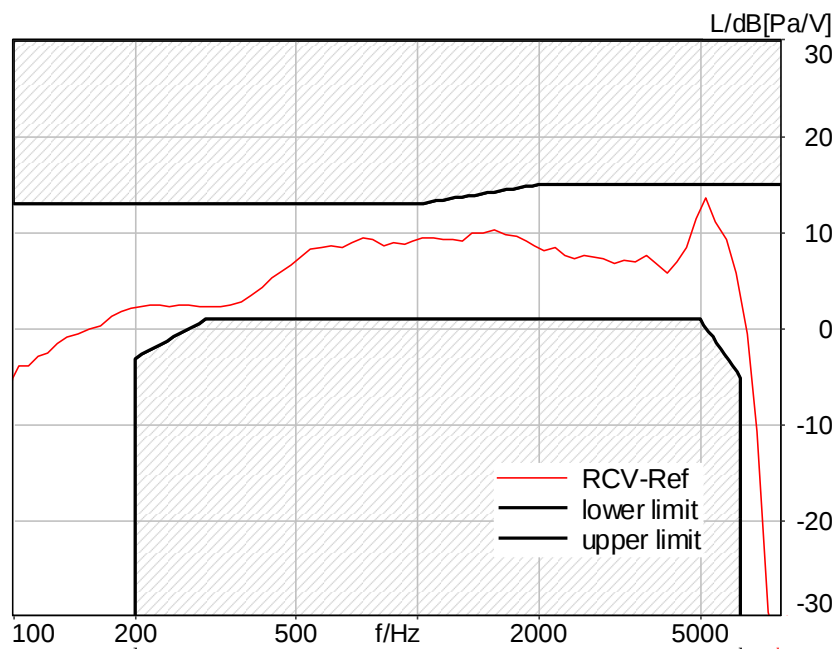
Figure C.2-7 – WCDMA Band IV 2N FF Wideband Frequency Response
