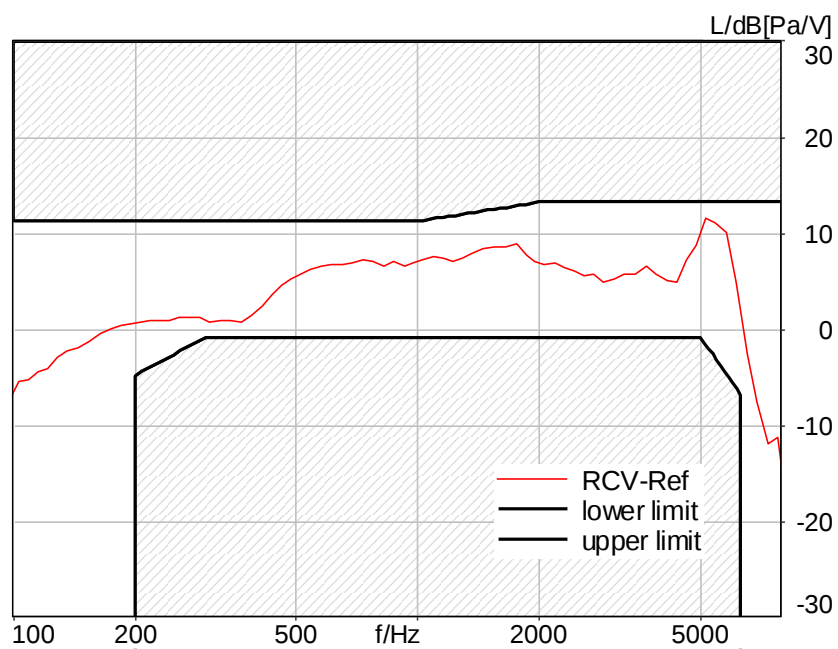
Figure C.4-20 – WLAN UNII-3 8N FF Wideband Frequency Response
