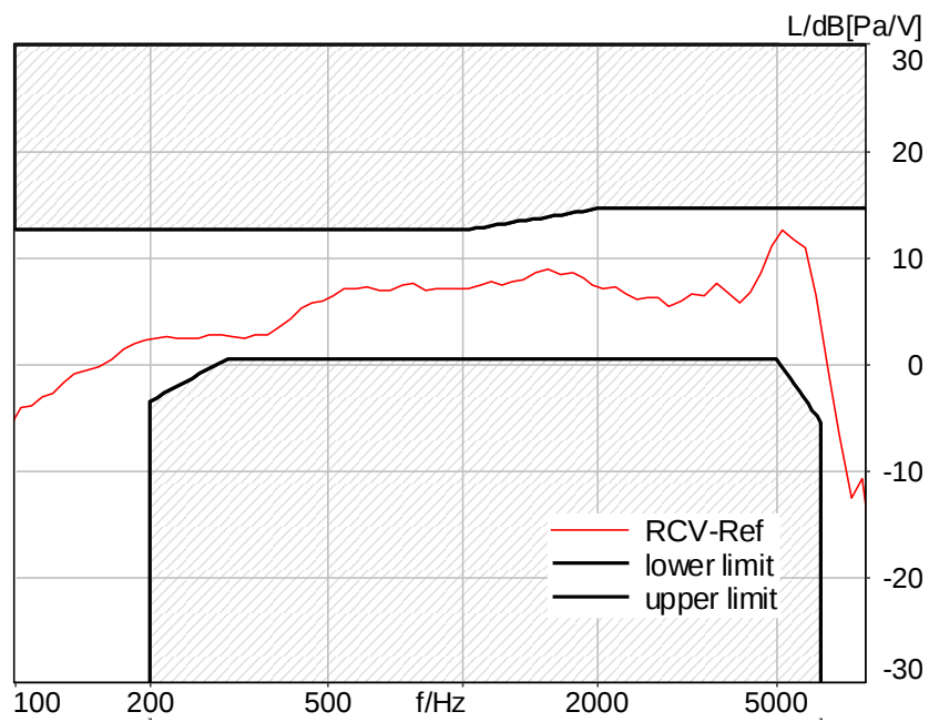
Figure C.3-7 – LTE Band 4 2N FF Wideband Frequency Response
