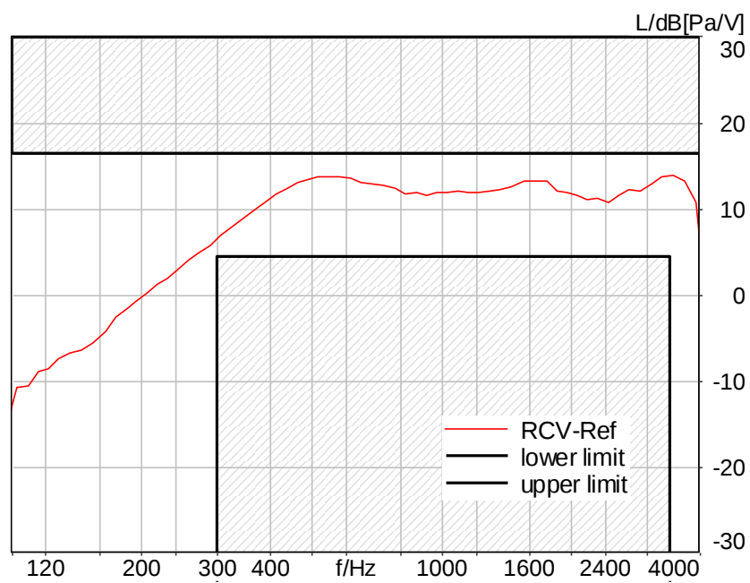
Figure C.3-6 – LTE Band 4 8N FF Narrowband Frequency Response
