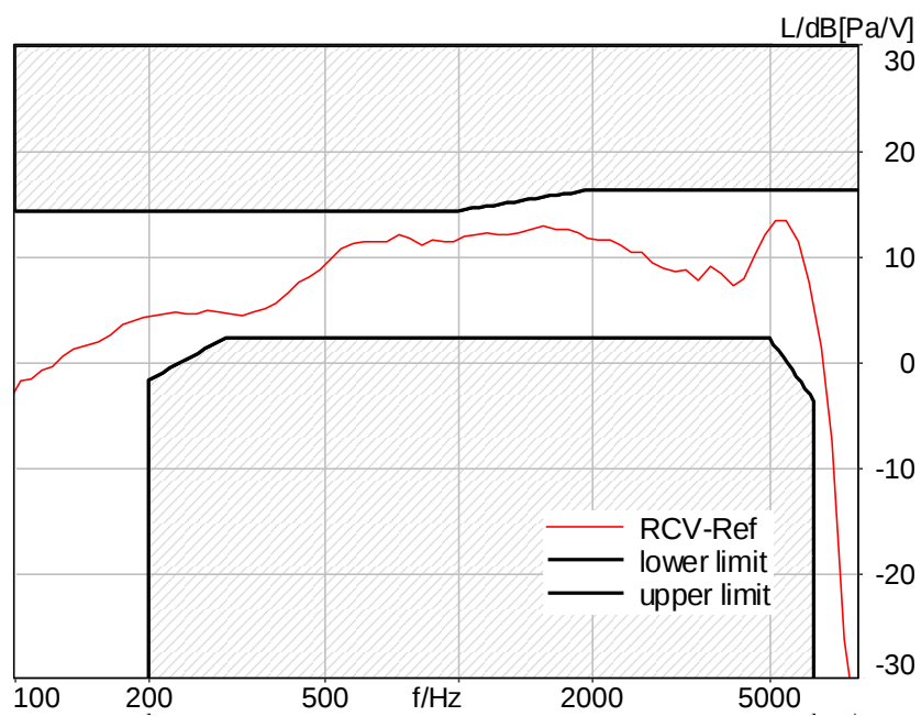
Figure C.2-8 – WCDMA Band IV 8N FF Wideband Frequency Response
