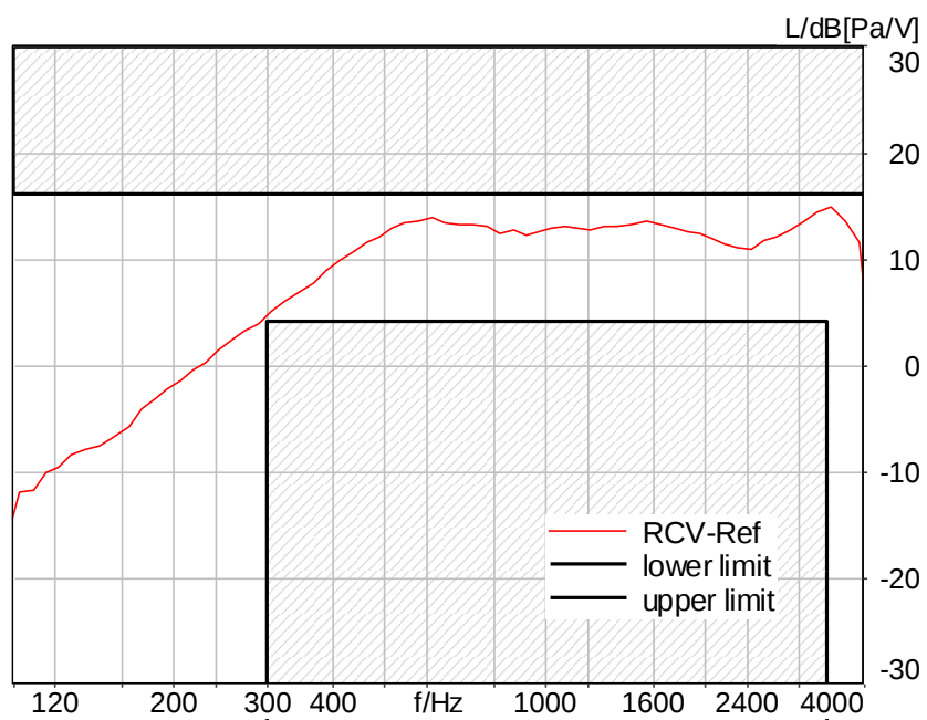
Figure C.2-6 – WCDMA Band IV 8N FF Narrowband Frequency Response
