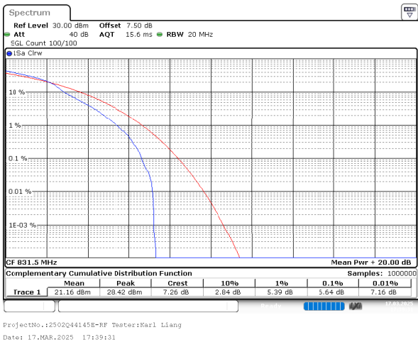
2_15MHz_Middle_QPSK_1@0
