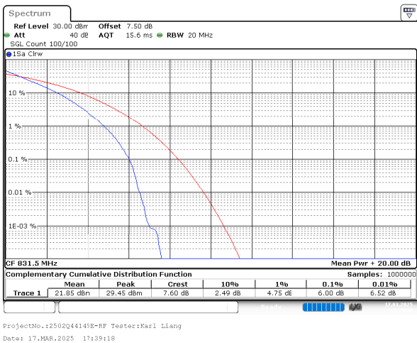
2_15MHz_Low_16QAM_75@0
