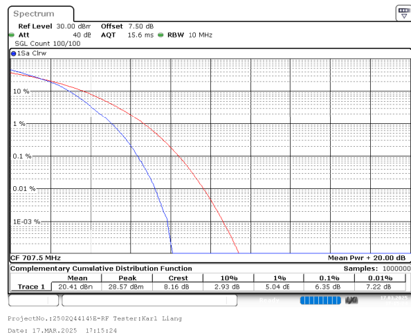
10MHz_High_QPSK_50@0
