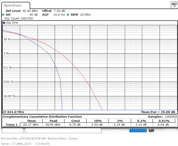
10MHz_High_16QAM_1@0
