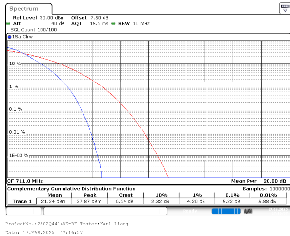
10MHz_High_16QAM_50@0
