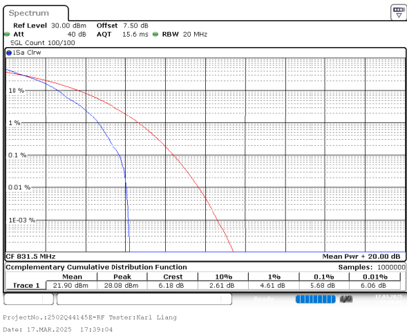
2_15MHz_Low_16QAM_1@0
