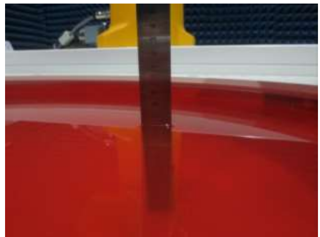
Fig. 9.6 Photo of Liquid Height for Body SAR of
