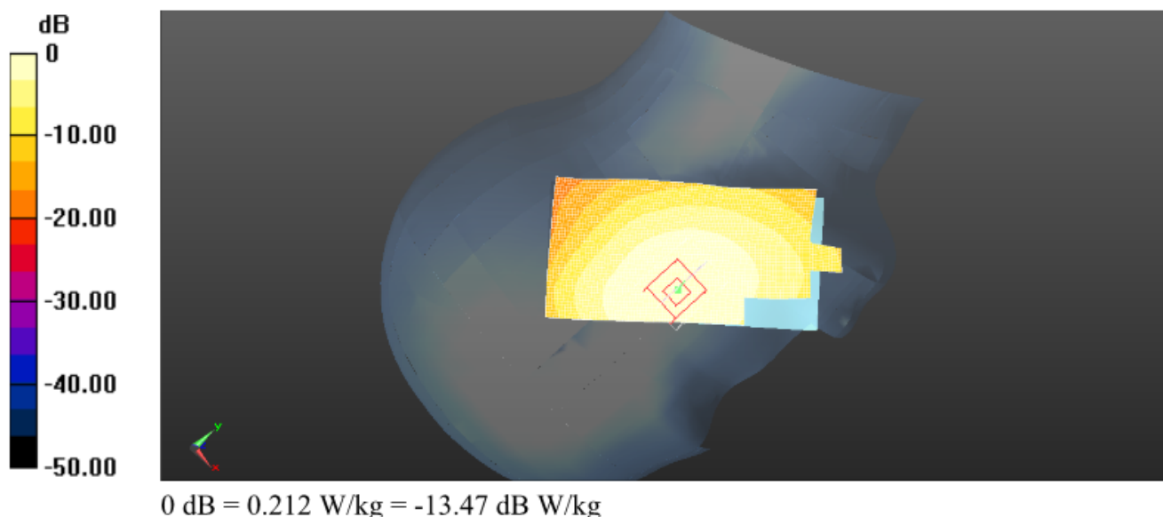
Plot 7: Right Head Touch (WCDMA Band V RMC Middle Channel)
