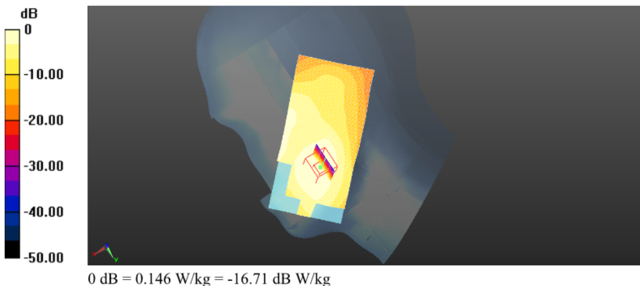
Plot 3: Right Head Touch (GSM1900 Middle Channel)
