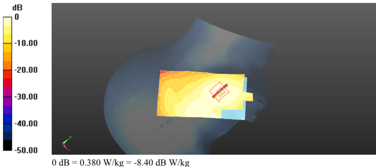
Plot 5: Right Head Touch (WCDMA Band II RMC Middle Channel)
