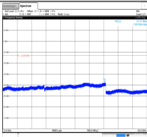
Band5-1.4MHz-16QAM-20525-1RB#0-3000~10000-PASS
