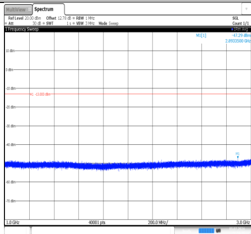
Band5-1.4MHz-16QAM-20643-1RB#0-1000~3000-PASS
