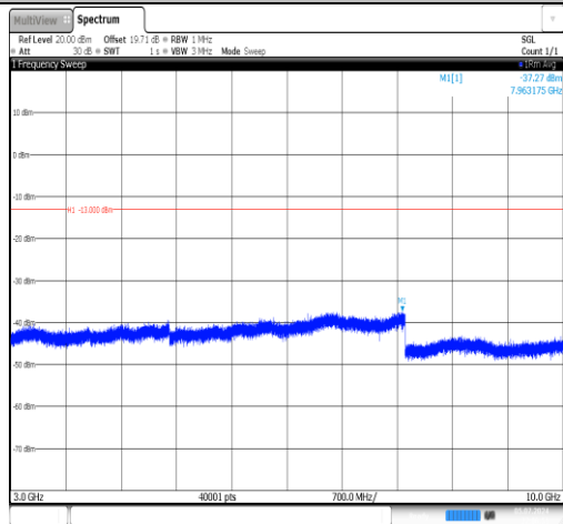
Band5-5MHz-16QAM-20525-1RB#0-3000~10000-PASS
