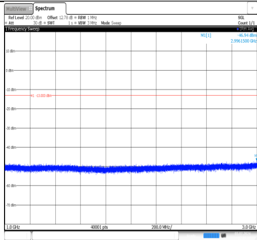
Band5-5MHz-16QAM-20625-1RB#0-1000~3000-PASS
