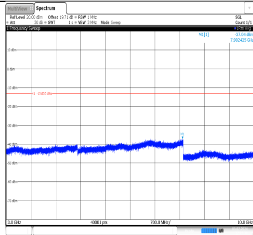
Band5-5MHz-16QAM-20625-1RB#0-3000~10000-PASS
