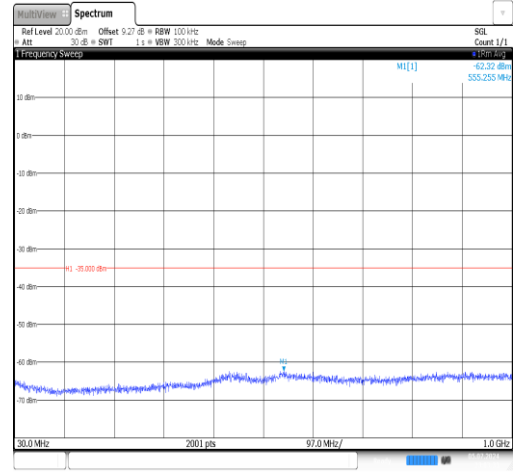
Band7-10MHz-16QAM-20800-1RB#0-30~1000-PASS
