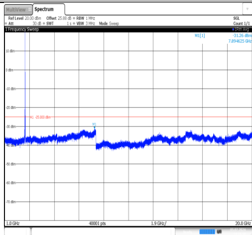
Band7-20MHz-16QAM-21350-1RB#0-1000~20000-PASS
