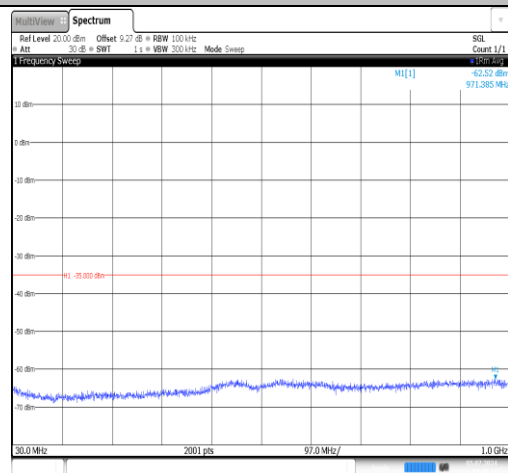
Band7-20MHz-16QAM-21350-1RB#0-30~1000-PASS
