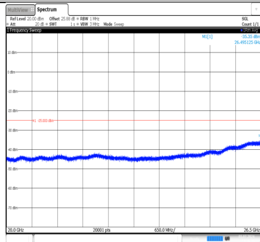
Band7-20MHz-16QAM-21350-1RB#0-20000~26500-PASS
