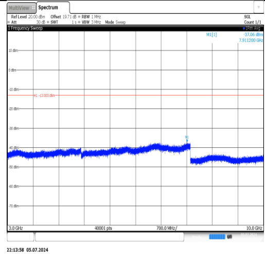
Band7-5MHz-QPSK-20775-1RB#0-1000~20000-PASS
