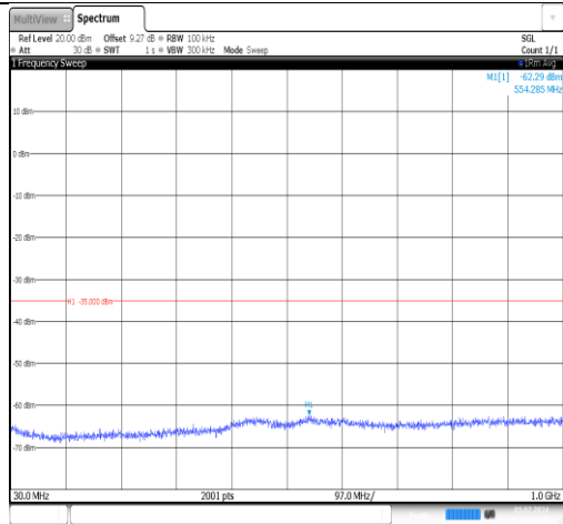
Band7-5MHz-QPSK-20775-1RB#0-20000-PASS
