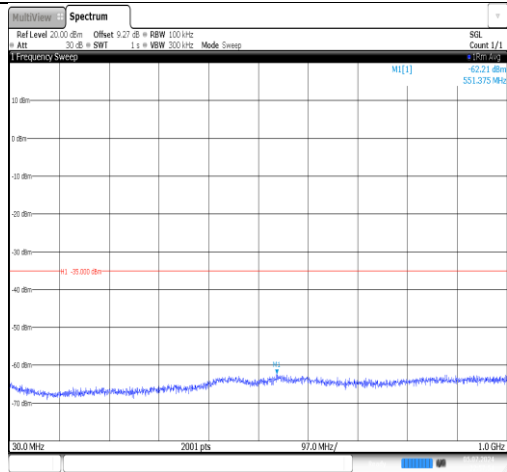
Band7-5MHz-QPSK-21425-1RB#0-20000-PASS
