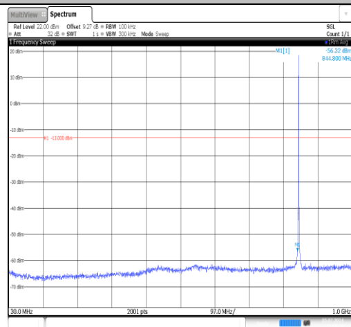
Band5-1.4MHz-16QAM-20643-1RB#0-30~1000-PASS
