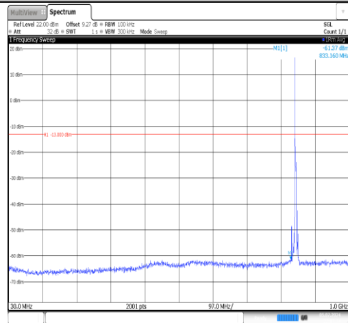
Band5-5MHz-16QAM-20625-1RB#0-30~1000-PASS
