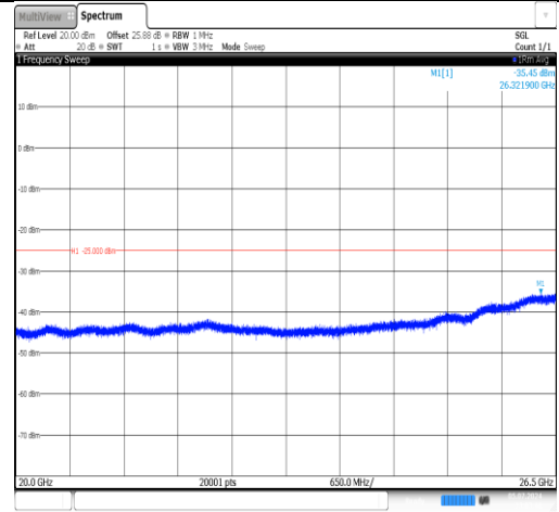
Band7-10MHz-16QAM-20800-1RB#0-20000~26500-PASS
