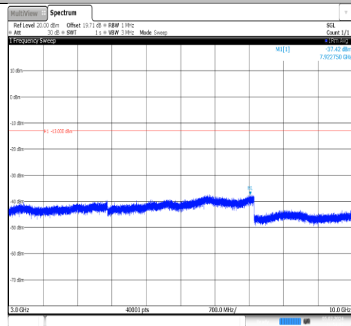
Band5-1.4MHz-16QAM-20643-1RB#0-3000~10000-PASS
