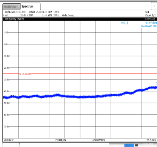
Band7-20MHz-16QAM-21100-1RB#0-20000-PASS
