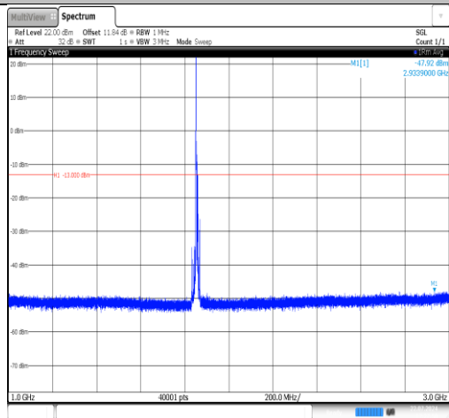
Band25-10MHz-16QAM-26090-1RB#0-1000~3000-PASS
