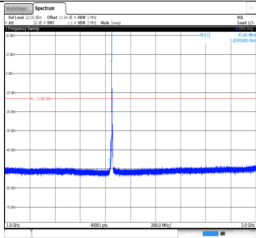
Band25-5MHz-16QAM-26065-1RB#0-1000~3000-PASS
