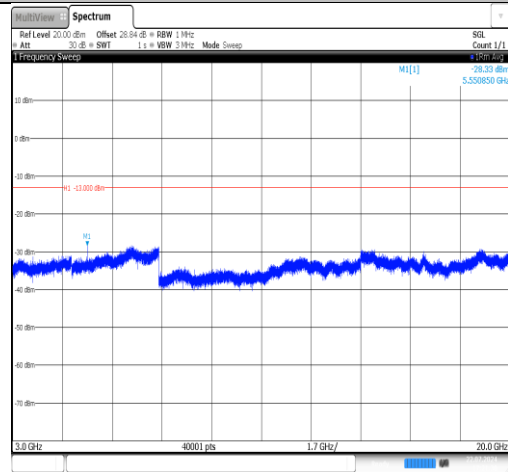
Band25-5MHz-16QAM-26065-1RB#0-3000~20000-PASS
