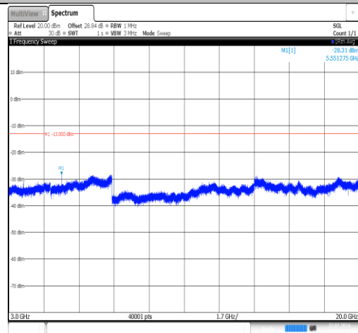
Band25-10MHz-16QAM-26090-1RB#0-3000~20000-PASS
