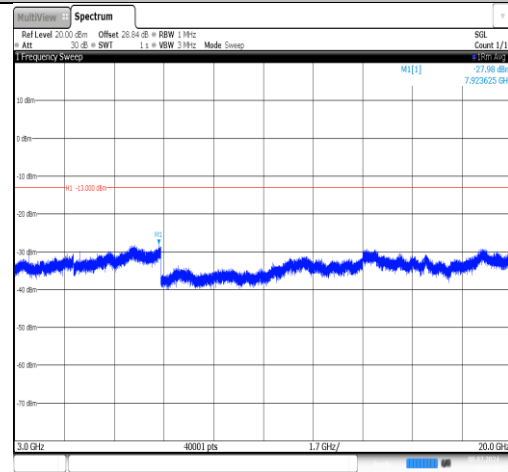
Band66-1.4MHz-QPSK-132322-1RB#0-3000~20000-PASS
