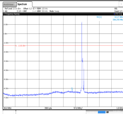
Band71-10MHz-16QAM-133172-1RB#0-30~1000-PASS
