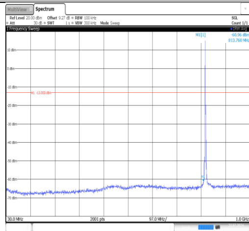
Band26(814-824)-3MHz-16QAM-26775-1RB#0-30~1000-PASS
