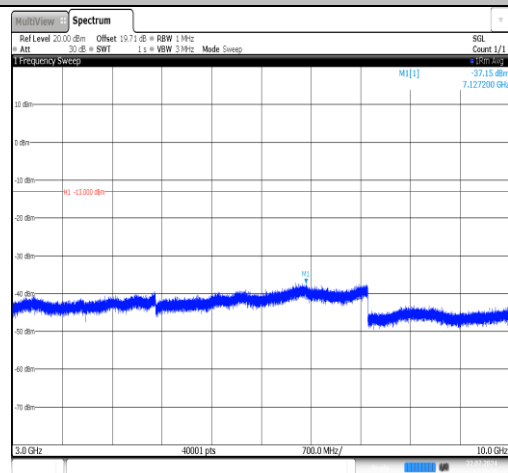
Band26(814-824)-3MHz-16QAM-26775-1RB#0-3000~10000-PASS
