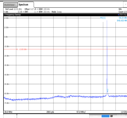
Band26(824-849)-1.4MHz-QPSK-26915-1RB#0-30~1000-PASS
