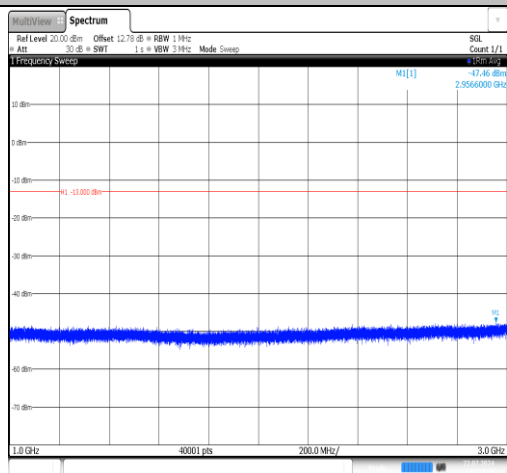
Band26(814-824)-1.4MHz-16QAM-26783-1RB#0-1000~3000-PASS
