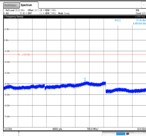
Band26(824-849)-1.4MHz-16QAM-27033-1RB#0-3000~10000-PASS
