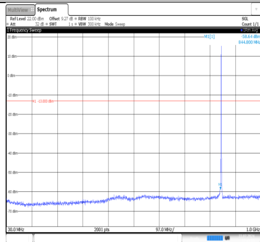
Band26(824-849)-1.4MHz-16QAM-27033-1RB#0-30~1000-PASS
