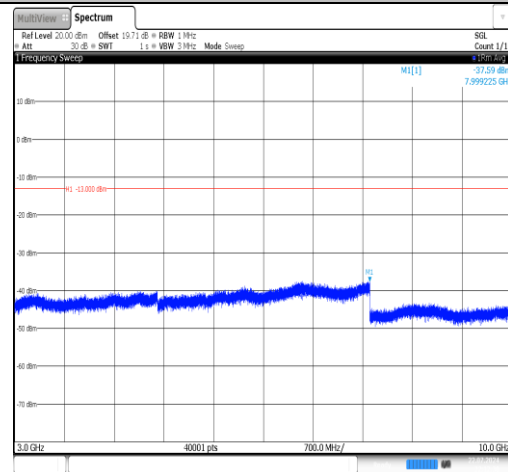
Band26(814-824)-1.4MHz-QPSK-26740-1RB#0-3000~10000-PASS
