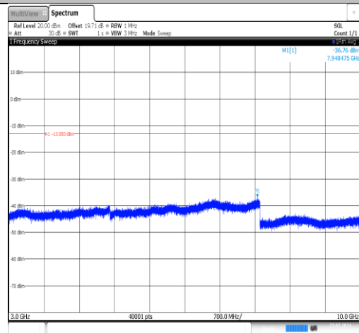
Band71-20MHz-QPSK-133322-1RB#0-3000~10000-PASS
