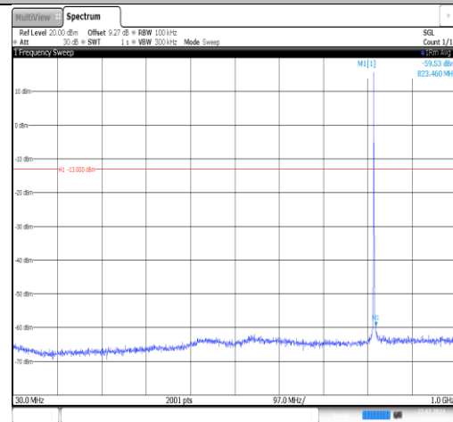
Band26(814-824)-1.4MHz-QPSK-26740-1RB#0-30~1000-PASS
