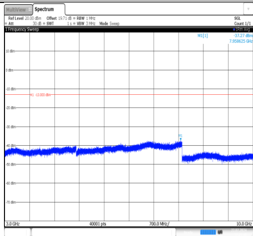
Band26(814-824)-3MHz-16QAM-26740-1RB#0-3000~10000-PASS
