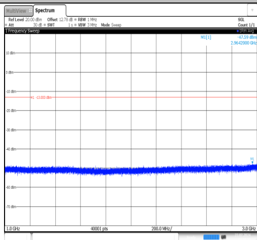
Band26(814-824)-10MHz-16QAM-26740-1RB#0-1000~3000-PASS
