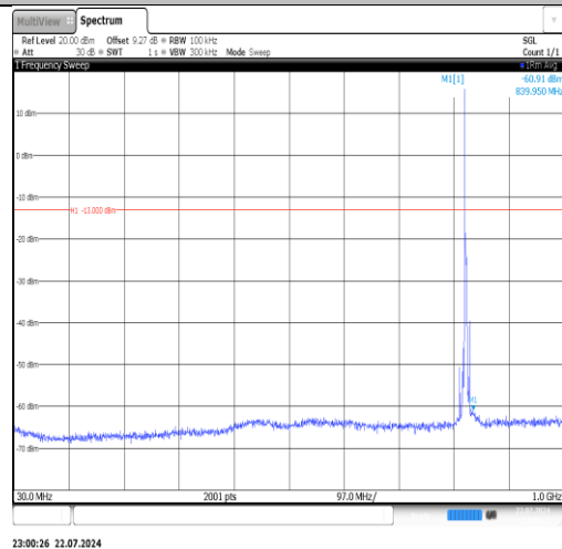
Band26(824-849)-5MHz-16QAM-26815-1RB#0-3000~10000-PASS
