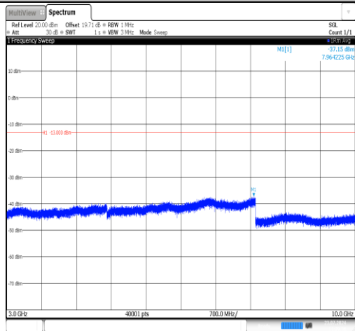
Band71-15MHz-QPSK-133397-1RB#0-3000~10000-PASS
