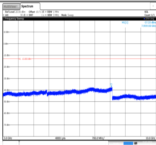
Band71-20MHz-QPSK-133222-1RB#0-3000~10000-PASS
