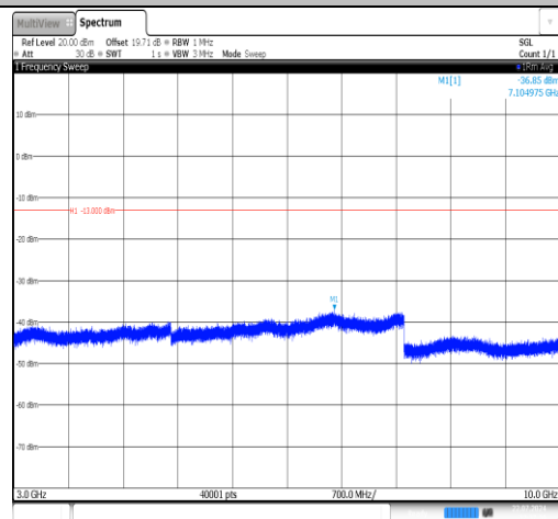
Band26(814-824)-10MHz-16QAM-26740-1RB#0-3000~10000-PASS
