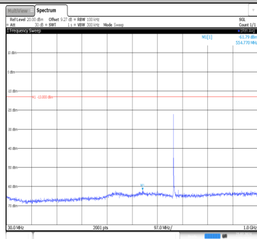
Band71-20MHz-QPSK-133322-1RB#0-30~1000-PASS
