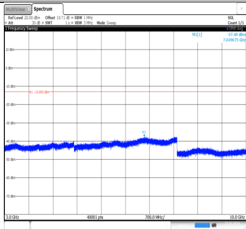
Band26(814-824)-10MHz-QPSK-26740-1RB#0-3000~10000-PASS
