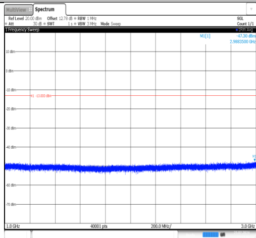
Band71-20MHz-QPSK-133322-1RB#0-1000~3000-PASS
