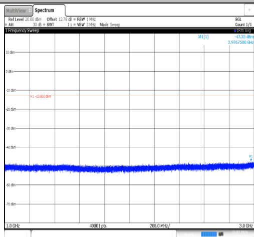
Band26(824-849)-1.4MHz-QPSK-26915-1RB#0-1000~3000-PASS
