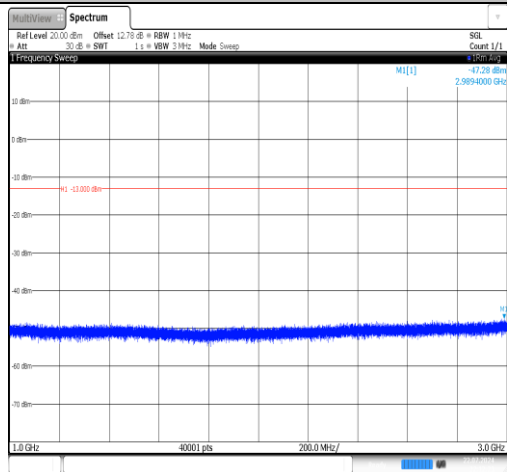
Band26(814-824)-1.4MHz-QPSK-26740-1RB#0-1000~3000-PASS
