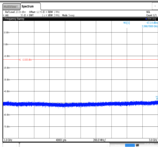
Band26(814-824)-3MHz-16QAM-26775-1RB#0-1000~3000-PASS
