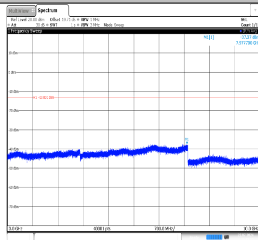
Band26(814-824)-1.4MHz-16QAM-26783-1RB#0-3000~10000-PASS
