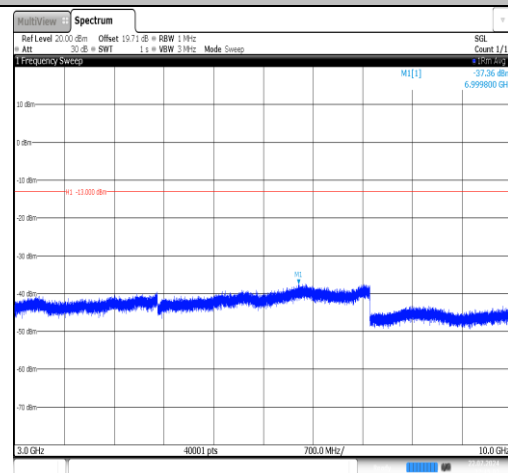
Band26(824-849)-1.4MHz-QPSK-26915-1RB#0-3000~10000-PASS
