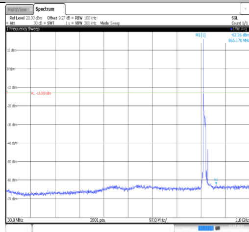
Band26(814-824)-10MHz-16QAM-26740-1RB#0-30~1000-PASS
