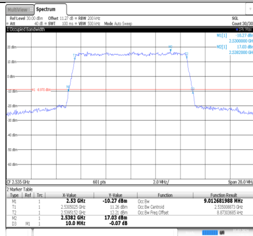
Band7-10MHz-16QAM-21100-50RB#0-PASS
