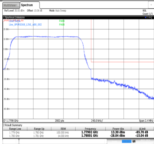
Band66-1.4MHz-16QAM-131979-1RB#0-PASS
