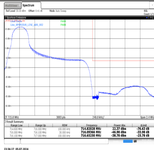
Band12-1.4MHz-QPSK-23173-1RB#5-PASS
