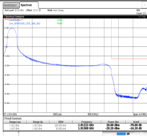
Band25-3MHz-16QAM-26675-1RB#14-PASS
