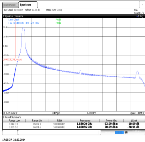
Band25-10MHz-16QAM-26090-1RB#49-PASS
