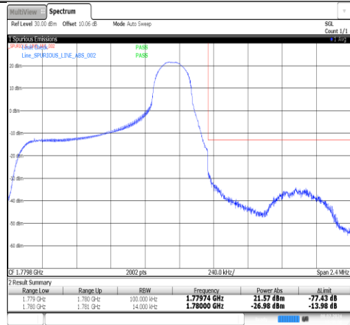
Band66-1.4MHz-16QAM-131979-6RB#0-PASS
