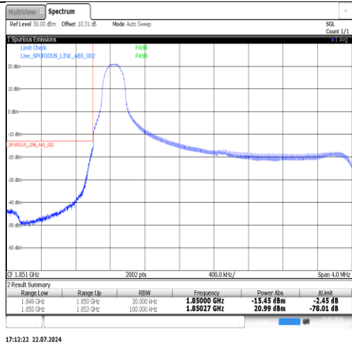
Band25-3MHz-QPSK-26055-1RB#14-PASS
