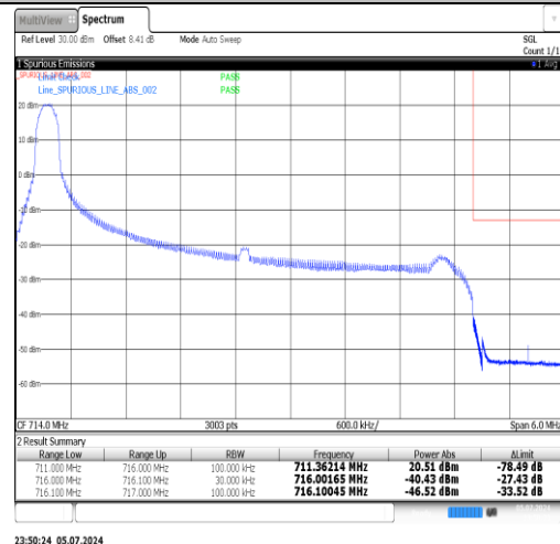
Band12-5MHz-16QAM-23155-1RB#24-PASS
