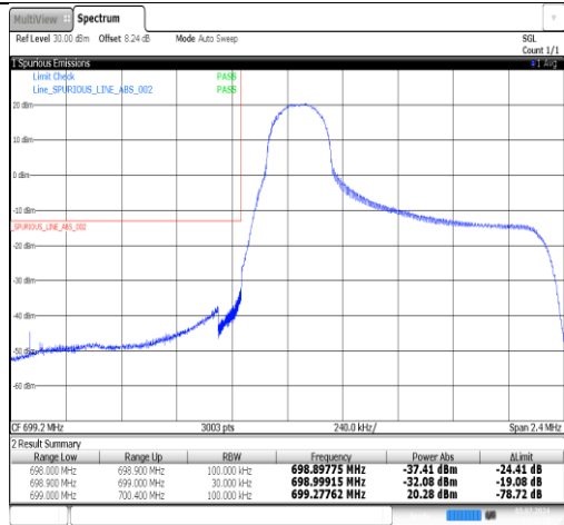
Band12-1.4MHz-QPSK-23017-1RB#5-PASS
