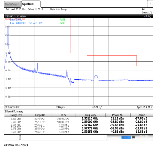
Band7-20MHz-16QAM-21350-1RB#99-PASS
