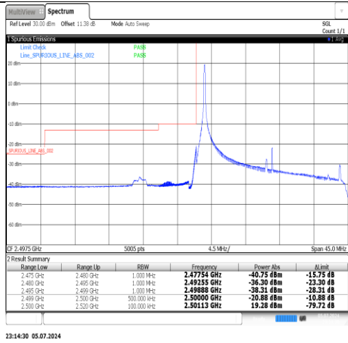
Band7-20MHz-16QAM-20850-1RB#99-PASS
