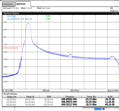
Band12-5MHz-16QAM-23035-1RB#24-PASS
