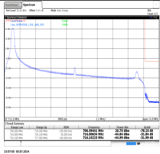
Band12-10MHz-16QAM-23130-1RB#49-PASS
