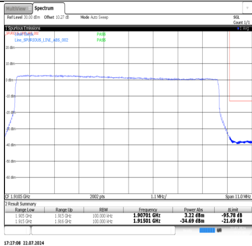
Band25-15MHz-QPSK-26115-1RB#0-PASS
