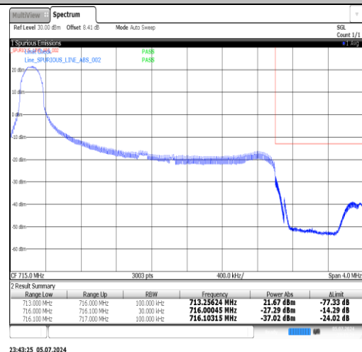
Band12-3MHz-16QAM-23165-1RB#14-PASS
