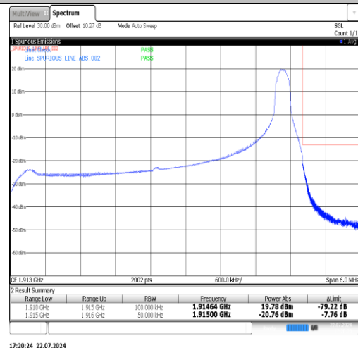
Band25-10MHz-QPSK-26090-50RB#0-PASS
