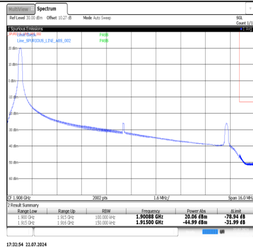
Band25-15MHz-16QAM-26615-1RB#74-PASS
