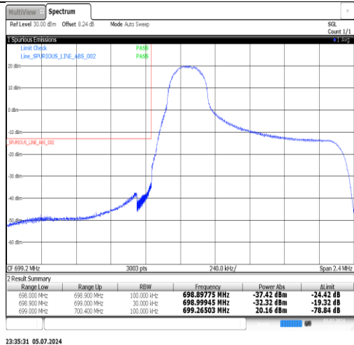
Band12-1.4MHz-16QAM-23017-1RB#5-PASS
