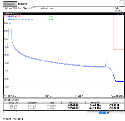
Band25-10MHz-16QAM-26640-1RB#49-PASS
