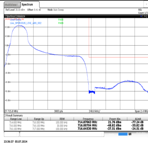
Band12-1.4MHz-16QAM-23173-1RB#5-PASS
