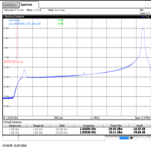
Band25-10MHz-16QAM-26640-50RB#0-PASS
