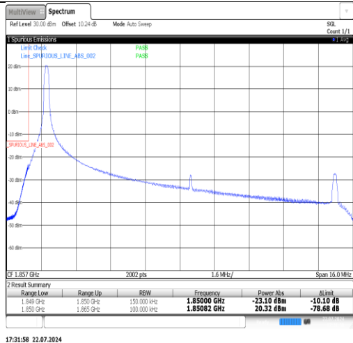
Band25-15MHz-16QAM-26115-1RB#74-PASS
