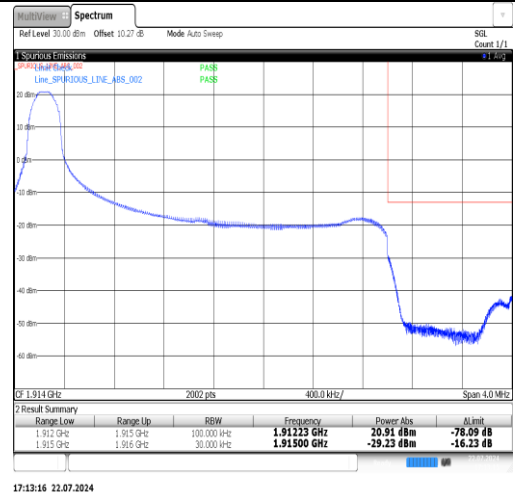
Band25-3MHz-QPSK-26675-1RB#14-PASS
