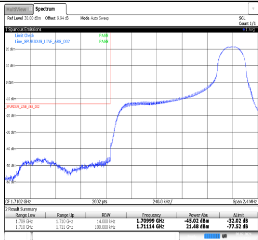
Band66-1.4MHz-QPSK-132665-6RB#0-PASS
