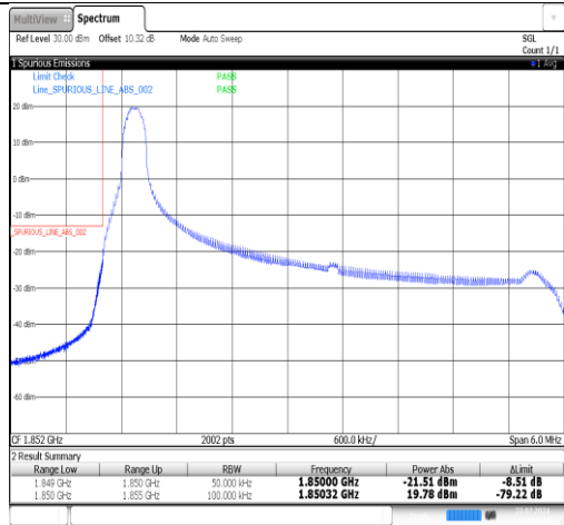
Band25-5MHz-16QAM-26065-1RB#24-PASS
