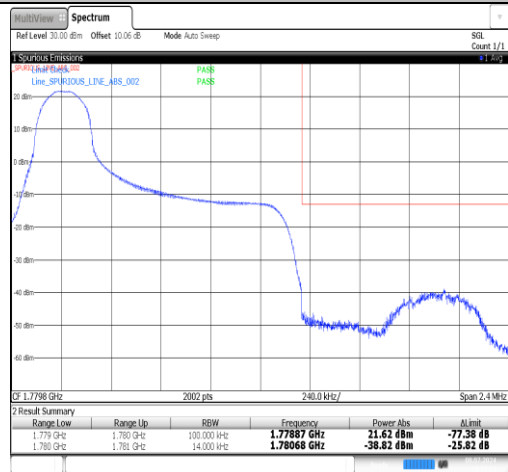
Band66-1.4MHz-QPSK-132665-1RB#5-PASS
