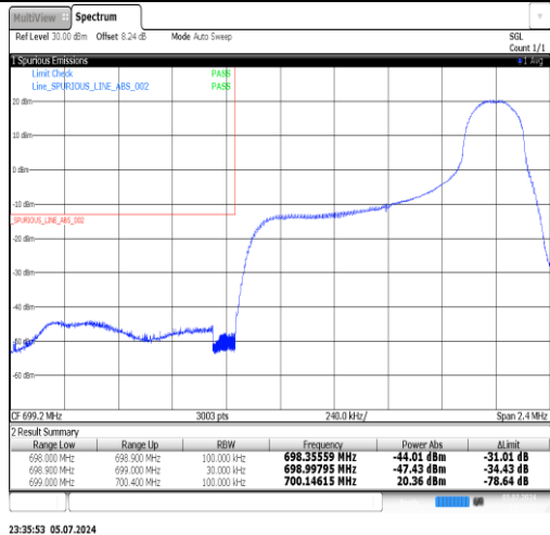
Band12-1.4MHz-16QAM-23173-6RB#0-PASS
