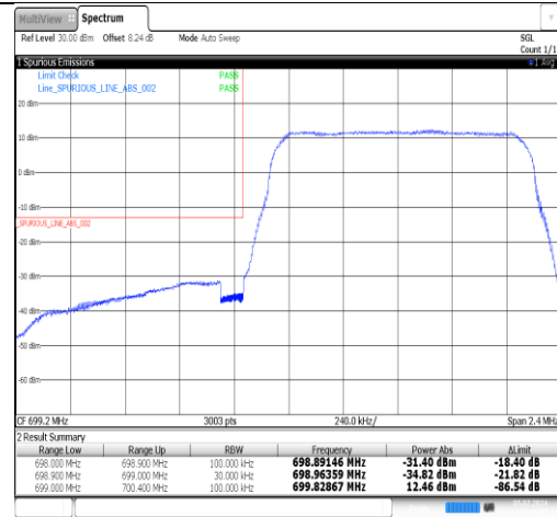
Band12-1.4MHz-QPSK-23173-1RB#0-PASS
