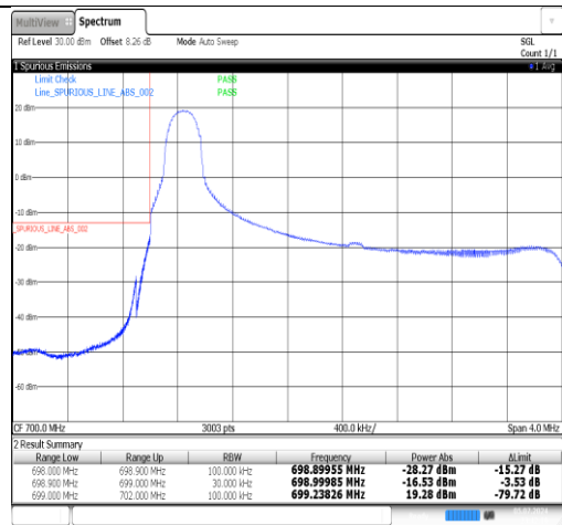
Band12-3MHz-16QAM-23025-1RB#14-PASS
