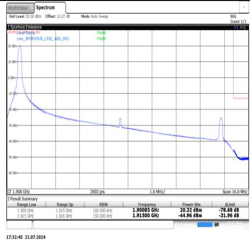
Band25-15MHz-QPSK-26615-1RB#74-PASS
