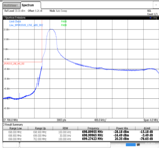
Band12-3MHz-QPSK-23025-1RB#14-PASS
