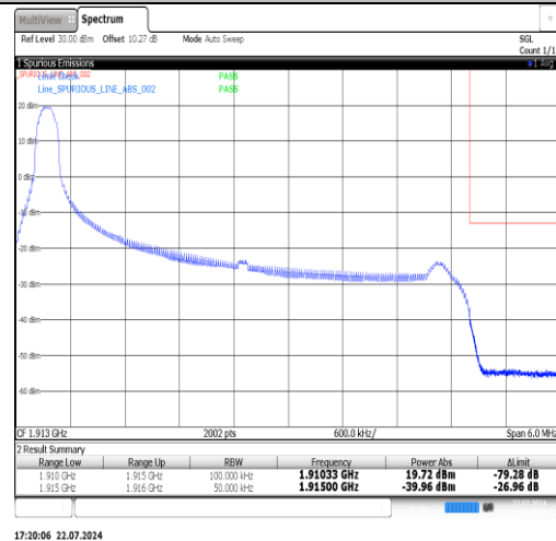
Band25-5MHz-16QAM-26665-1RB#24-PASS
