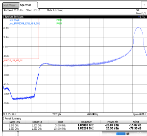
Band25-3MHz-16QAM-26675-15RB#0-PASS
