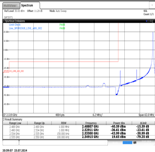
Band41(2535-2655)-15MHz-16QAM-41165-75RB#0-PASS
