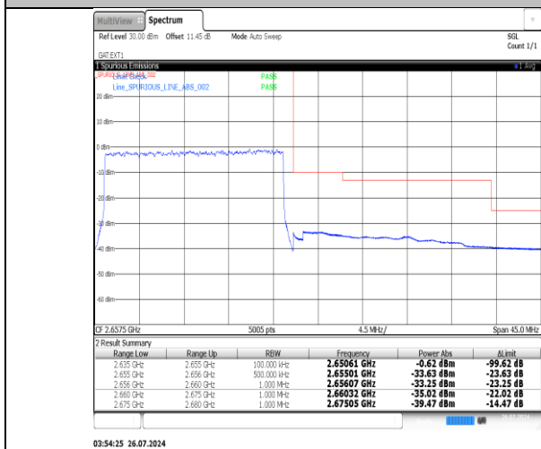
Band41(2535-2655)-20MHz-16QAM-41140-100RB#0-PASS
