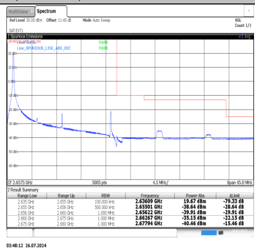
Band41(2535-2655)-20MHz-16QAM-41140-1RB#0-PASS
