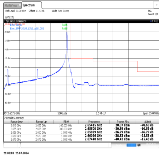
Band41(2535-2655)-20MHz-QPSK-40140-100RB#0-PASS
