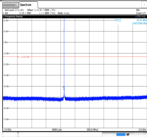
Band2-1.4MHz-16QAM-18607-1RB#0-1000~3000-PASS
