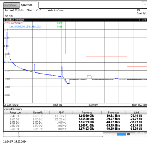
Band41(2535-2655)-15MHz-16QAM-41165-1RB#74-PASS
