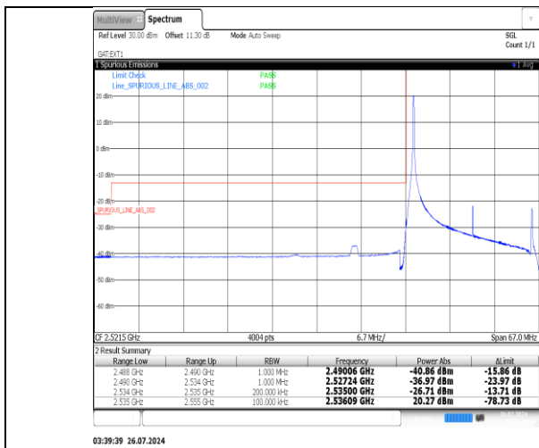
Band41(2535-2655)-20MHz-16QAM-40140-1RB#99-PASS
