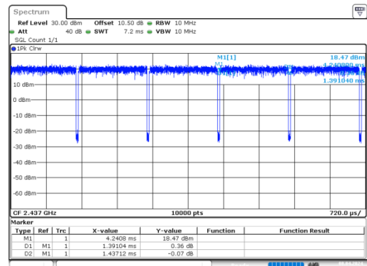
g_2437MHz_Chain 0
