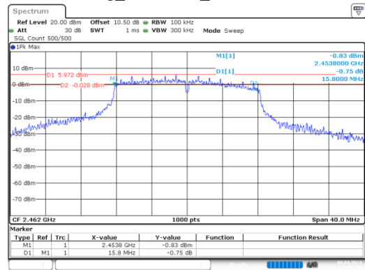
g_2462MHz_Chain 0
