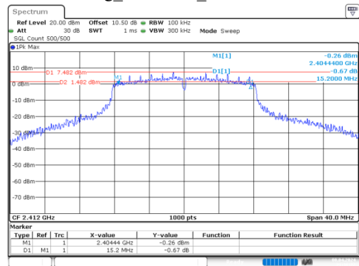
g_2412MHz_Chain 0
