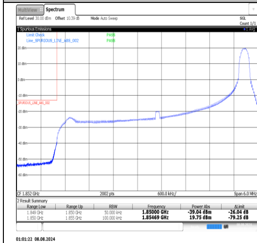
Band25-5MHz-16QAM-26665-25RB#0-PASS
