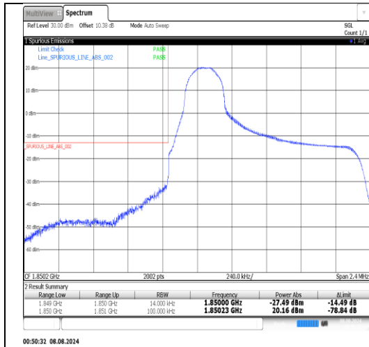
Band25-1.4MHz-QPSK-26047-1RB#5-PASS
