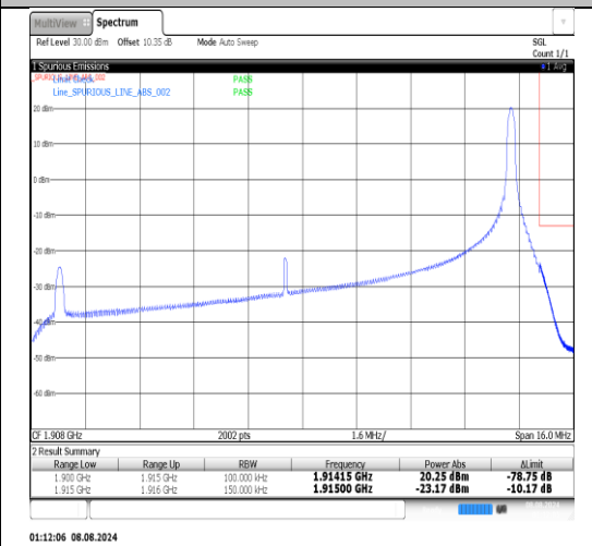
Band25-15MHz-16QAM-26115-75RB#0-PASS
