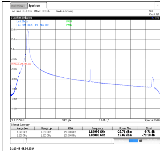
Band25-15MHz-QPSK-26115-1RB#74-PASS
