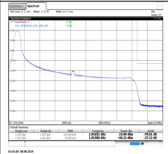
Band25-5MHz-QPSK-26665-1RB#24-PASS
