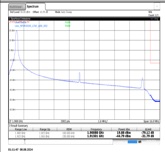
Band25-15MHz-QPSK-26615-1RB#74-PASS
