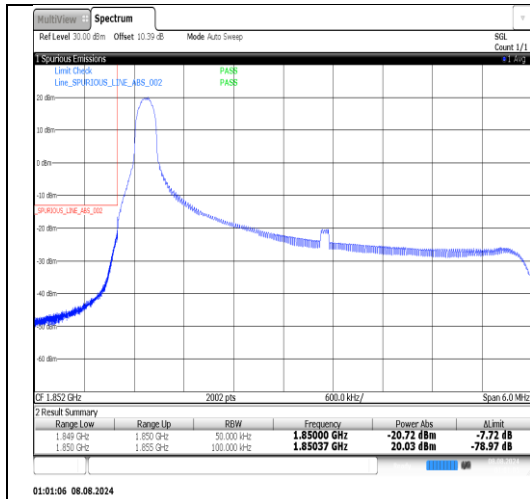
Band25-5MHz-16QAM-26065-1RB#24-PASS
