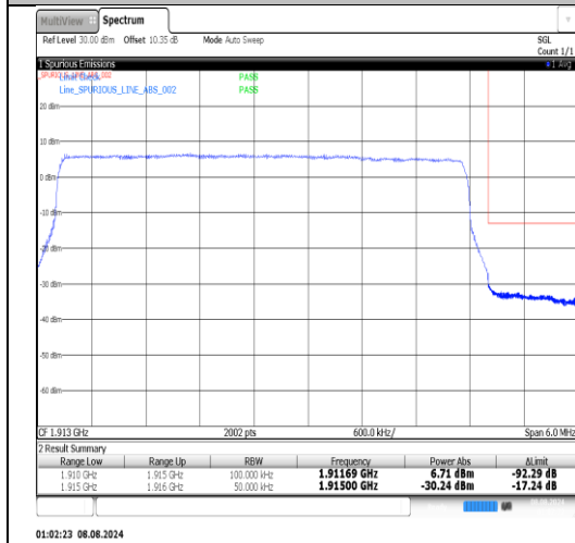
Band25-5MHz-16QAM-26065-1RB#0-PASS
