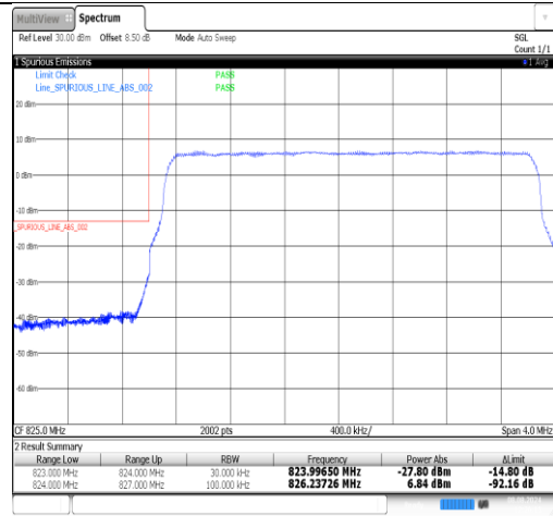
Band26(824-849)-3MHz-16QAM-27025-1RB#0-PASS
