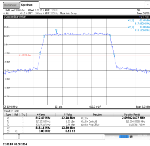
Band26(814-824)-5MHz-16QAM-26740-25RB#0-PASS
