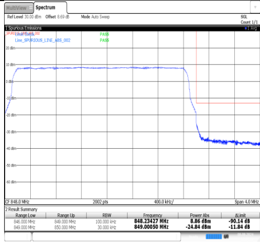
Band26(824-849)-3MHz-16QAM-27025-15RB#0-PASS
