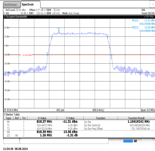
Band26(814-824)-3MHz-16QAM-26740-15RB#0-PASS
