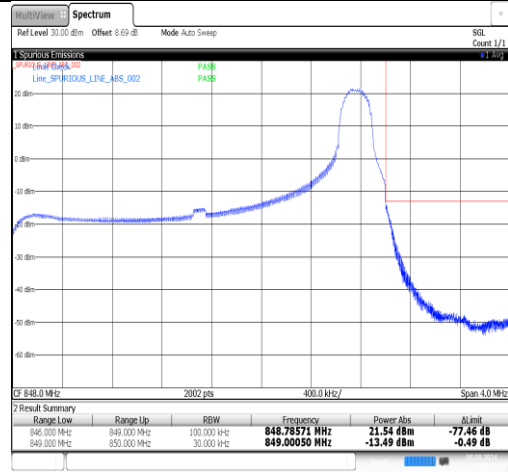
Band26(824-849)-3MHz-16QAM-27025-1RB#14-PASS
