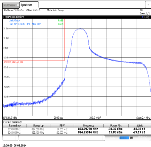
Band26(824-849)-1.4MHz-QPSK-26797-1RB#5-PASS
