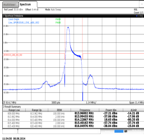
Band26(814-824)-1.4MHz-QPSK-26697-1RB#5-PASS
