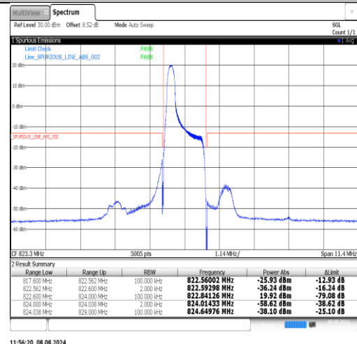
Band26(814-824)-1.4MHz-QPSK-26783-1RB#5-PASS
