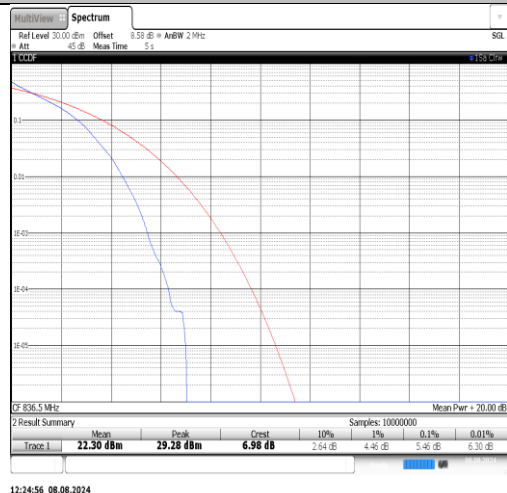
Band26(824-849)-5MHz-QPSK-26915-25RB#0-PASS
