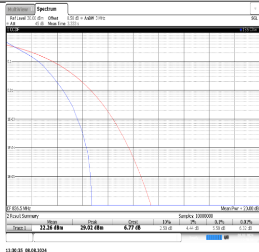
Band26(824-849)-10MHz-QPSK-26915-50RB#0-PASS
