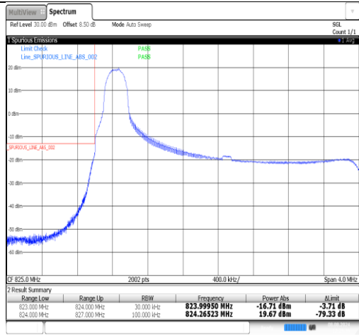
Band26(824-849)-3MHz-16QAM-26805-1RB#14-PASS
