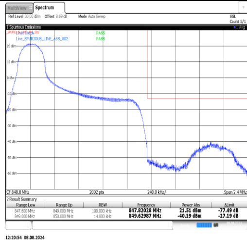
Band26(824-849)-1.4MHz-QPSK-27033-1RB#5-PASS
