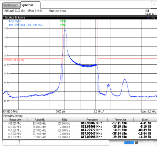
Band26(814-824)-3MHz-QPSK-26705-1RB#14-PASS
