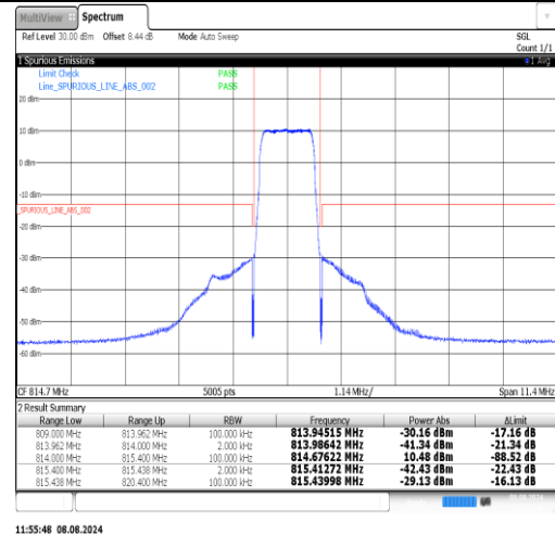
Band26(814-824)-1.4MHz-QPSK-26783-1RB#0-PASS
