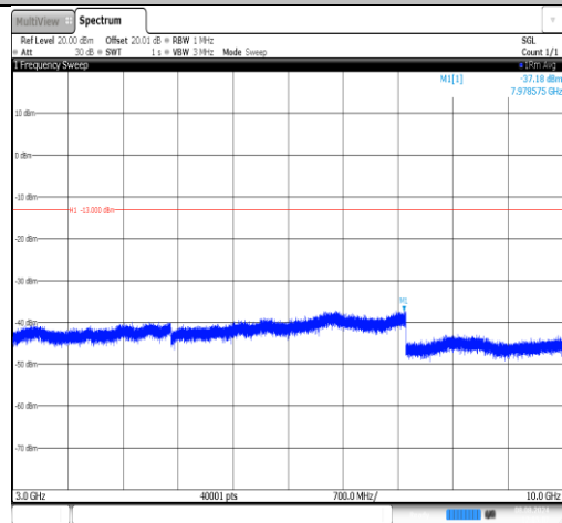
Band26(814-824)-3MHz-16QAM-26705-1RB#0-3000~10000-PASS
