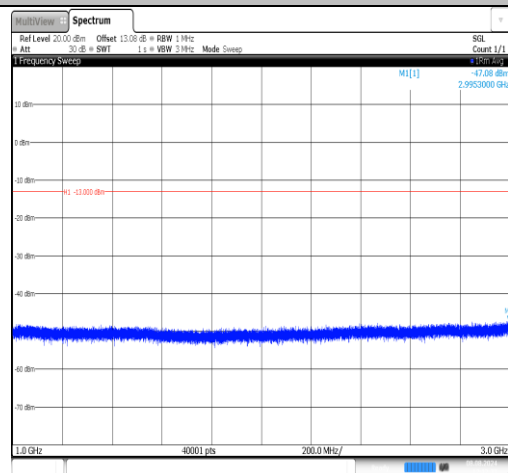
Band26(814-824)-5MHz-16QAM-26740-1RB#0- 1000~3000-PASS
