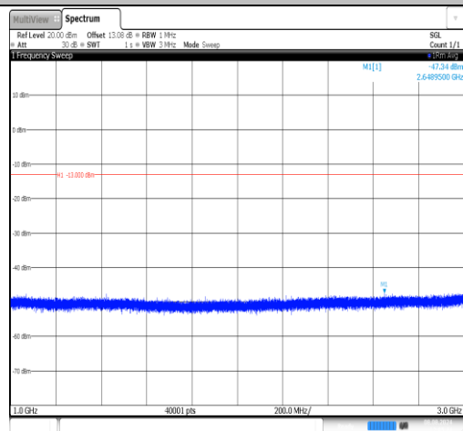
Band26(814-824)-3MHz-16QAM-26740-1RB#0-1000~3000-PASS
