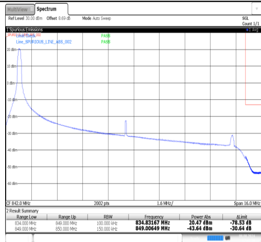
Band26(824-849)-15MHz-QPSK-26965-1RB#74-PASS
