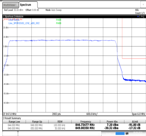
Band26(824-849)-5MHz-QPSK-27015-25RB#0-PASS
