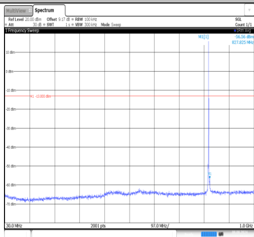
Band26(814-824)-1.4MHz-QPSK-26783-1RB#0-30~1000-PASS
