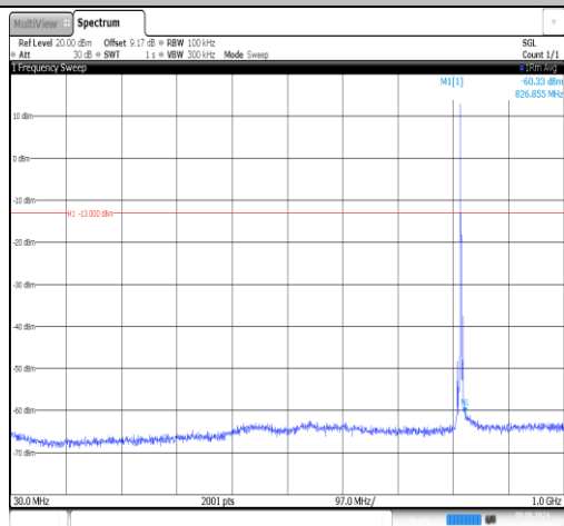
Band26(814-824)-3MHz-16QAM-26740-1RB#0-30~1000-PASS
