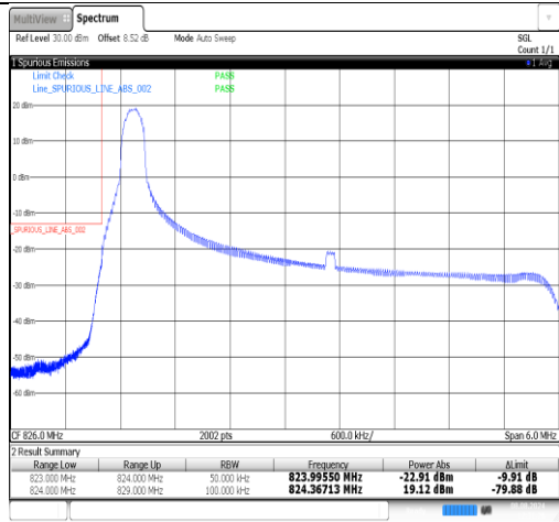
Band26(824-849)-5MHz-16QAM-26815-1RB#24-PASS
