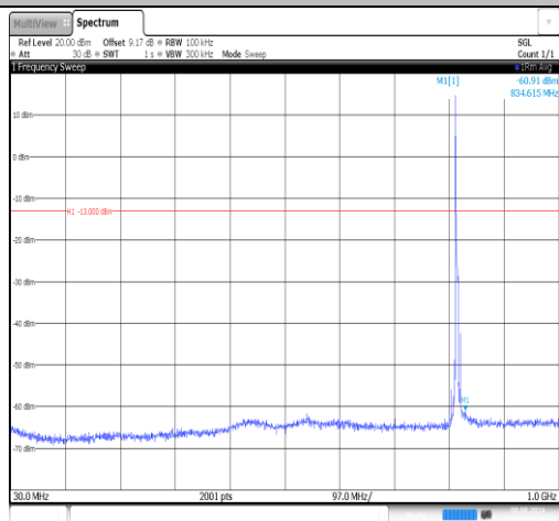
Band26(814-824)-5MHz-16QAM-26740-1RB#0-30~1000- PASS
