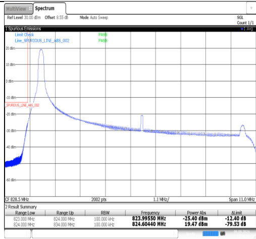
Band26(824-849)-10MHz-16QAM-26840-1RB#49-PASS
