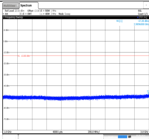
Band26(814-824)-5MHz-16QAM-26715-1RB#0- 1000~3000-PASS
