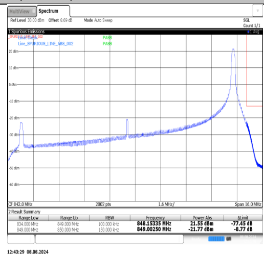
Band26(824-849)-15MHz-16QAM-26965-1RB#74-PASS
