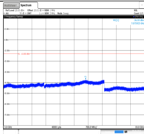
Band26(814-824)-5MHz-16QAM-26715-1RB#0- 3000~10000-PASS
