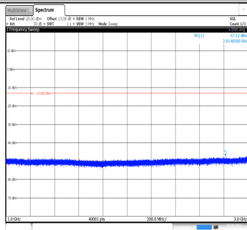
Band26(814-824)-1.4MHz-QPSK-26783-1RB#0-1000~3000-PASS
