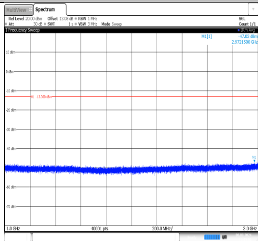
Band26(814-824)-3MHz-16QAM-26705-1RB#0-1000~3000-PASS
