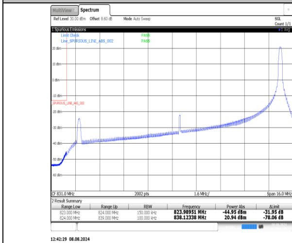
Band26(824-849)-15MHz-16QAM-26965-75RB#0-PASS
