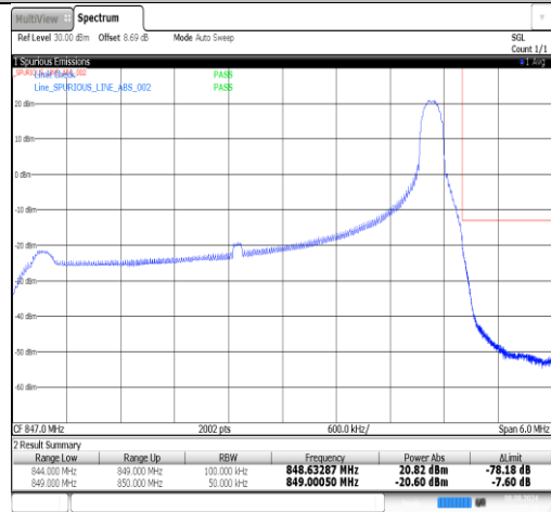
Band26(824-849)-5MHz-QPSK-27015-1RB#24-PASS
