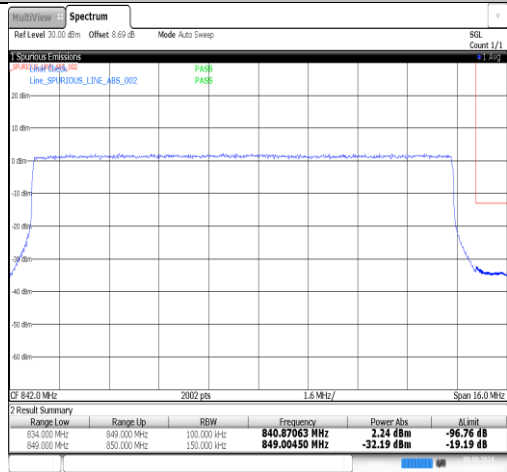
Band26(824-849)-15MHz-QPSK-26965-75RB#0-PASS
