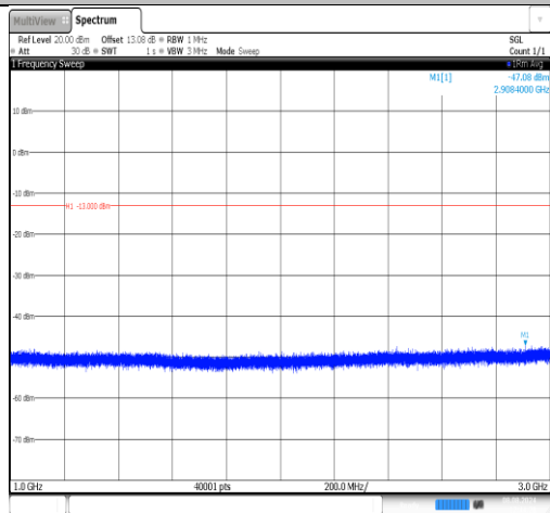
Band26(824-849)-15MHz-16QAM-26865-1RB#0- 1000~3000-PASS
