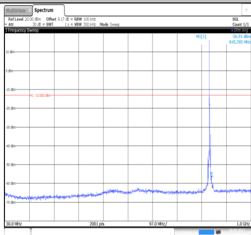
Band26(824-849)-3MHz-16QAM-26915-1RB#0-30~1000- PASS
