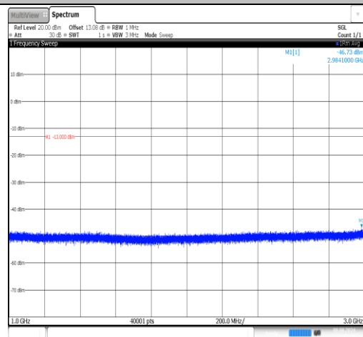
Band26(824-849)-15MHz-QPSK-26965-1RB#0- 1000~3000-PASS
