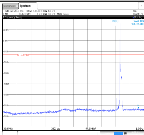
Band26(824-849)-15MHz-QPSK-26965-1RB#0-30~1000- PASS
