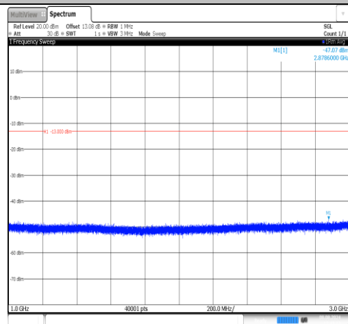
Band26(824-849)-15MHz-16QAM-26915-1RB#0- 1000~3000-PASS
