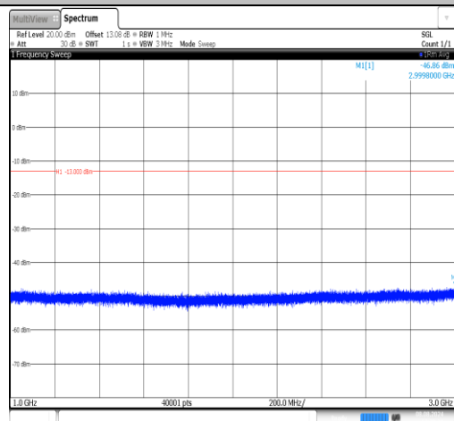
Band26(824-849)-10MHz-16QAM-26915-1RB#0-1000~3000-PASS
