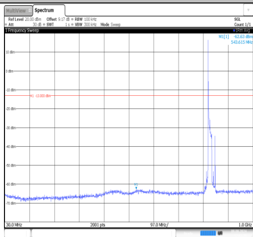
Band26(824-849)-15MHz-QPSK-26865-1RB#0-30~1000- PASS
