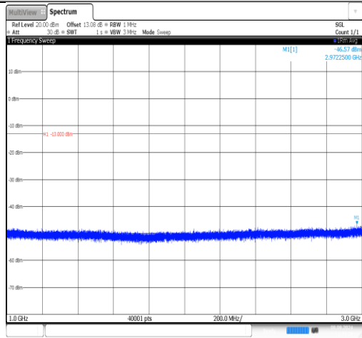
Band26(824-849)-15MHz-16QAM-26965-1RB#0- 1000~3000-PASS
