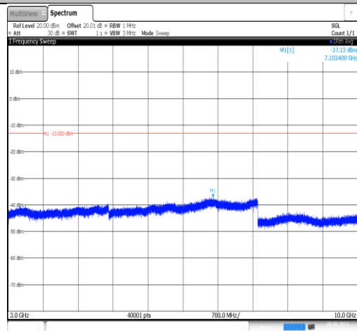
Band26(824-849)-10MHz-16QAM-26840-1RB#0-3000~10000-PASS
