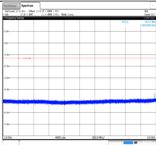
Band26(824-849)-15MHz-QPSK-26915-1RB#0- 1000~3000-PASS
