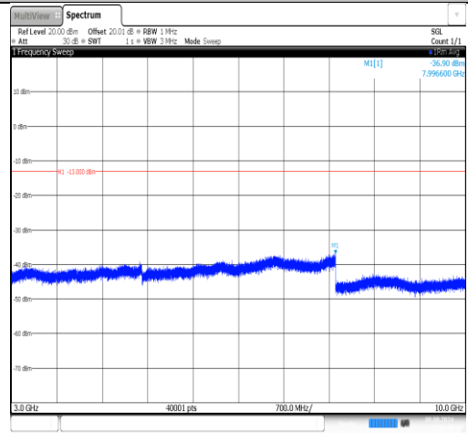
Band26(824-849)-15MHz-16QAM-26965-1RB#0- 3000~10000-PASS
