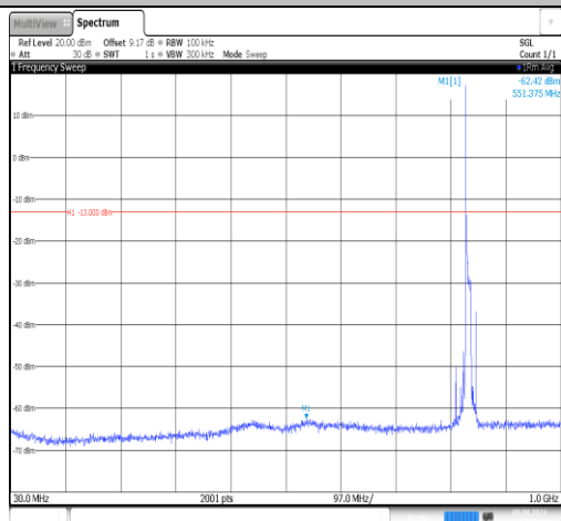
Band26(824-849)-10MHz-16QAM-26915-1RB#0-30~1000-PASS
