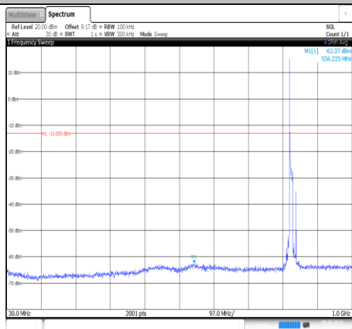
Band26(824-849)-10MHz-QPSK-26840-1RB#0-30~1000- PASS
