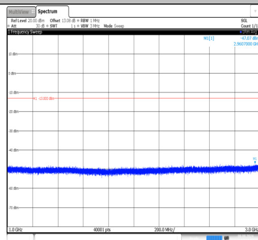
Band26(824-849)-5MHz-16QAM-26915-1RB#0- 1000~3000-PASS
