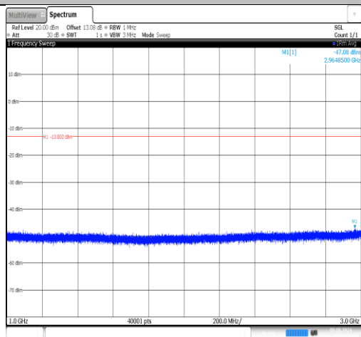
Band26(824-849)-5MHz-16QAM-26815-1RB#0- 1000~3000-PASS
