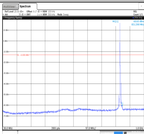
Band26(824-849)-5MHz-16QAM-26915-1RB#0-30~1000- PASS
