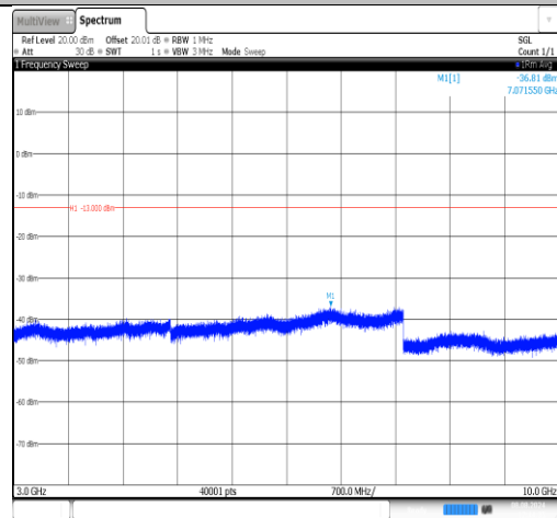
Band26(824-849)-15MHz-16QAM-26865-1RB#0- 3000~10000-PASS
