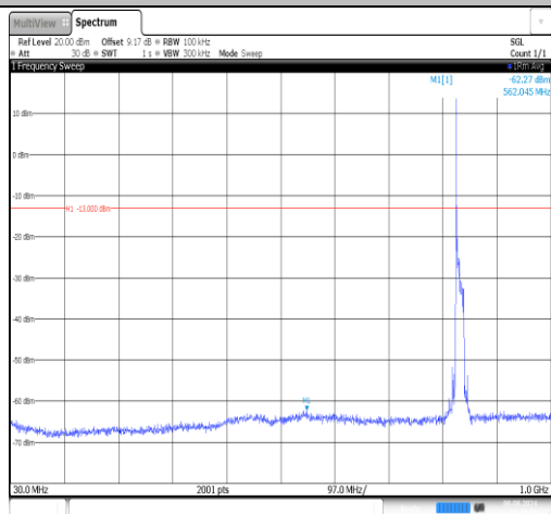
Band26(824-849)-15MHz-16QAM-26915-1RB#0-30~1000- PASS
