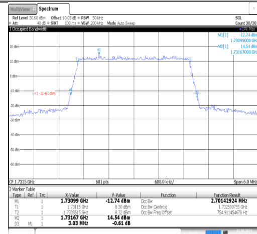
Band4-3MHz-16QAM-20175-15RB#0-PASS
