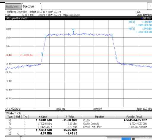
Band4-5MHz-16QAM-20175-25RB#0-PASS
