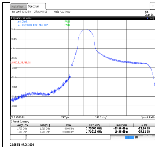
Band4-1.4MHz-16QAM-19957-1RB#5-PASS
