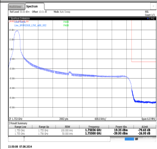
Band4-5MHz-16QAM-20375-1RB#24-PASS
