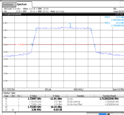
Band4-3MHz-QPSK-20175-15RB#0-PASS
