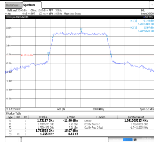
Band4-1.4MHz-16QAM-20175-6RB#0-PASS
