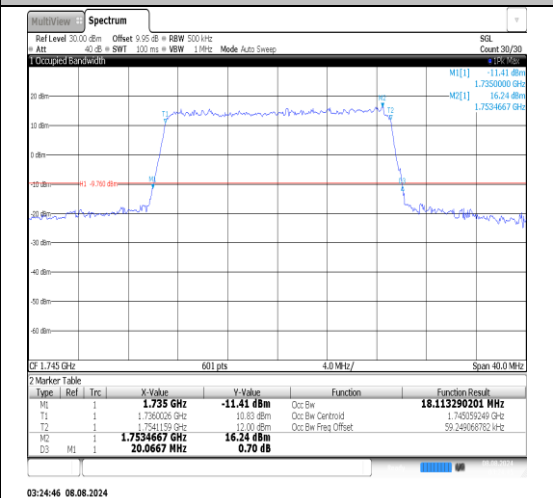
Band66-20MHz-16QAM-132322-100RB#0- PASS
