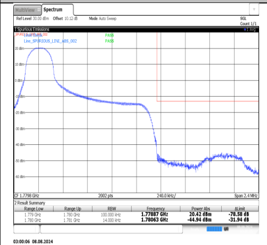
Band66-1.4MHz-16QAM-132665-1RB#5- PASS
