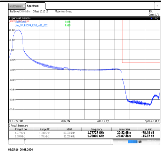
Band66-3MHz-16QAM-132657-1RB#14-PASS
