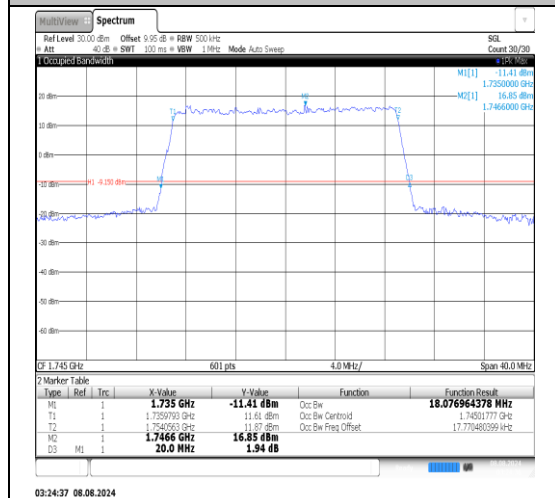
Band66-20MHz-QPSK-132322-100RB#0- PASS
