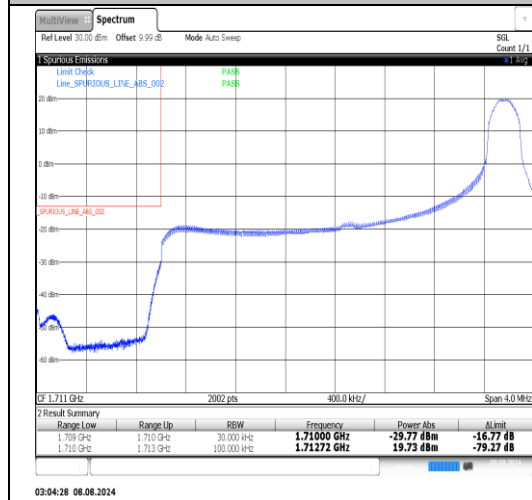
Band66-3MHz-QPSK-132657-15RB#0-PASS
