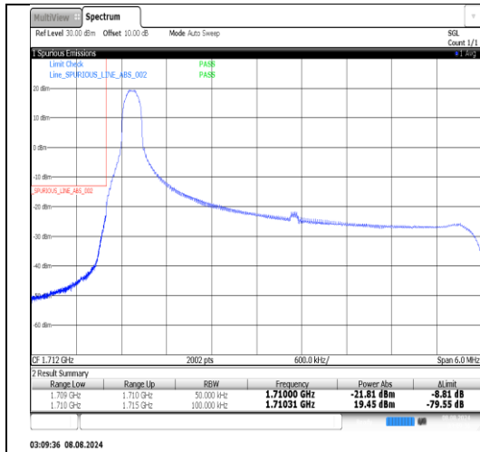
Band66-5MHz-QPSK-131997-1RB#24-PASS
