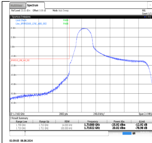
Band66-1.4MHz-QPSK-131979-1RB#5-PASS
