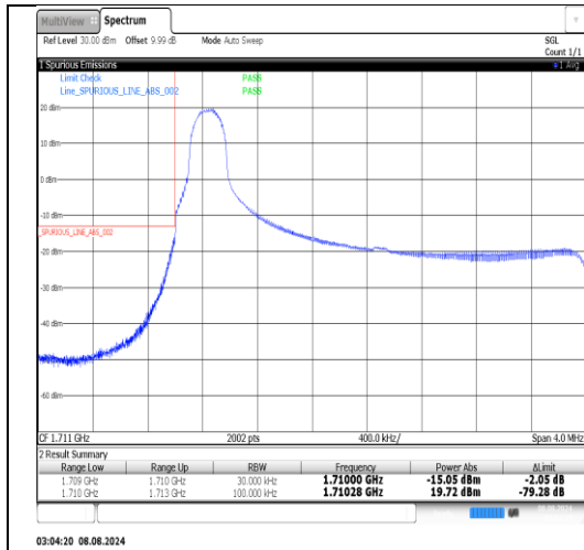
Band66-3MHz-16QAM-131987-1RB#14-PASS
