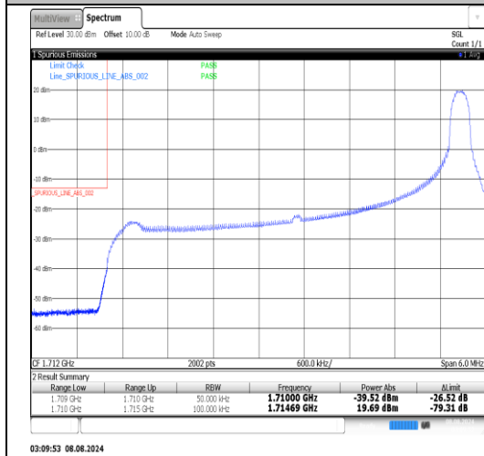
Band66-5MHz-QPSK-132647-25RB#0-PASS
