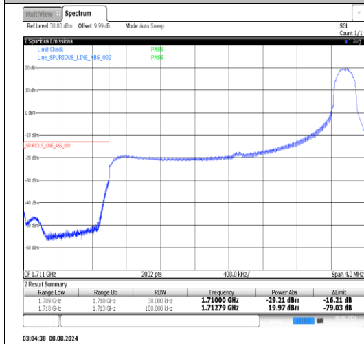
Band66-3MHz-16QAM-132657-15RB#0-PASS
