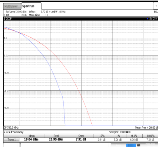
Band13-10MHz-16QAM-23230-50RB#0-PASS
