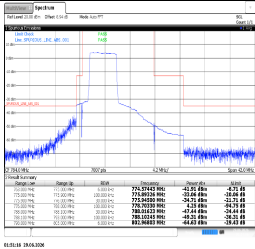
Band13-5MHz-16QAM-23255-1RB#24-PASS
