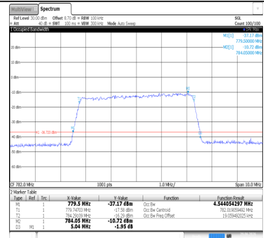
Band13-5MHz-16QAM-23230-25RB#0-PASS
