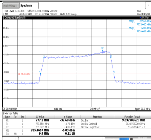
Band13-10MHz-QPSK-23230-50RB#0-PASS
