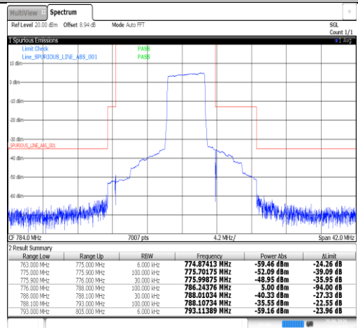
Band13-5MHz-QPSK-23255-25RB#0-PASS
