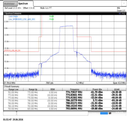
Band13-10MHz-QPSK-23230-1RB#49-PASS
