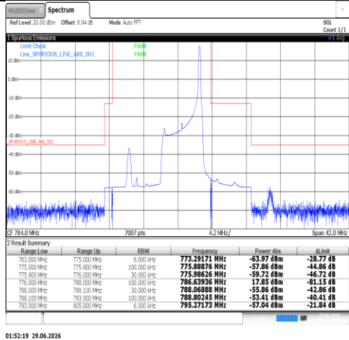
Band13-10MHz-QPSK-23230-1RB#0-PASS
