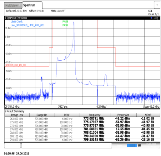
Band13-5MHz-16QAM-23255-1RB#0-PASS
