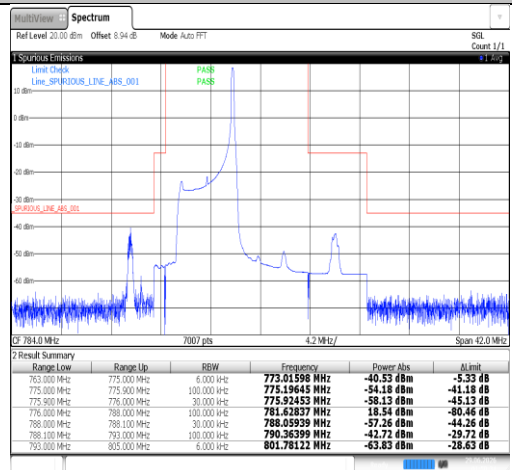
Band13-5MHz-QPSK-23205-1RB#24-PASS
