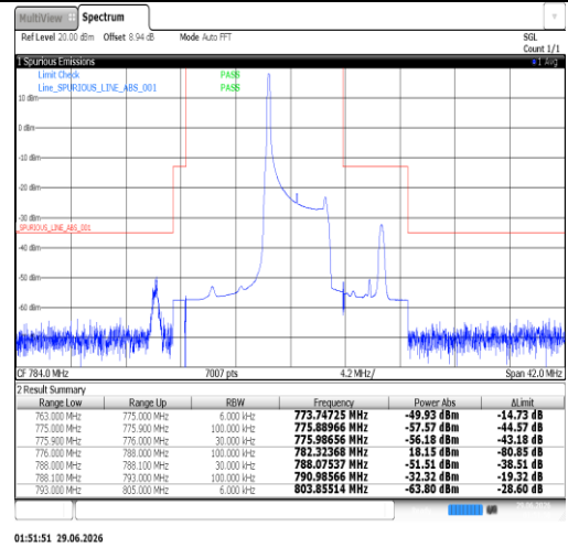
Band13-5MHz-16QAM-23255-25RB#0-PASS
