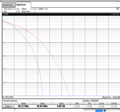
Band13-10MHz-QPSK-23230-50RB#0-PASS
