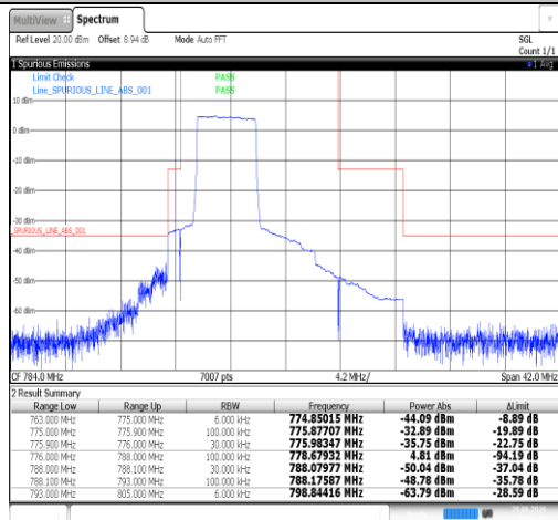
Band13-5MHz-QPSK-23205-25RB#0-PASS
