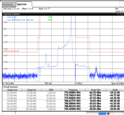
Band13-5MHz-QPSK-23255-1RB#24-PASS
