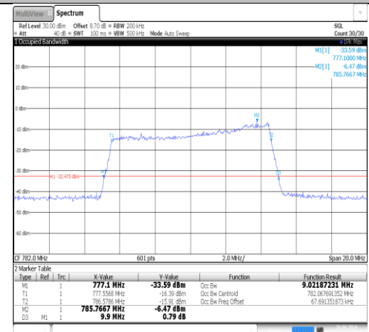
Band13-10MHz-16QAM-23230-50RB#0-PASS
