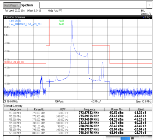
Band13-5MHz-QPSK-23255-1RB#0-PASS
