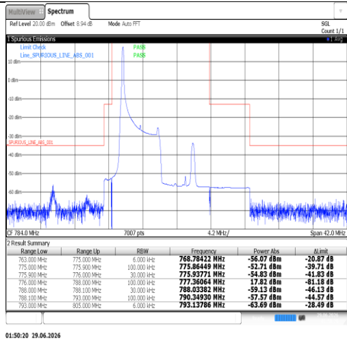
Band13-5MHz-16QAM-23205-25RB#0-PASS
