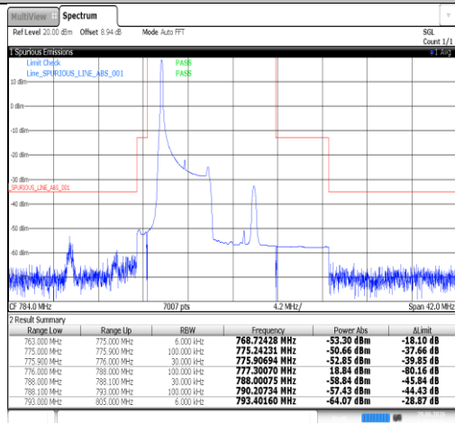
Band13-5MHz-QPSK-23205-1RB#0-PASS
