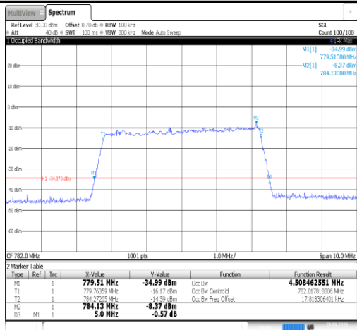
Band13-5MHz-QPSK-23230-25RB#0-PASS
