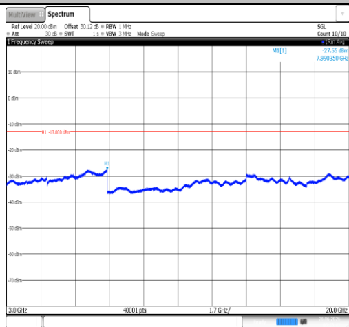
Band2-3MHz-16QAM-19185-1RB#0-3000~20000-PASS
