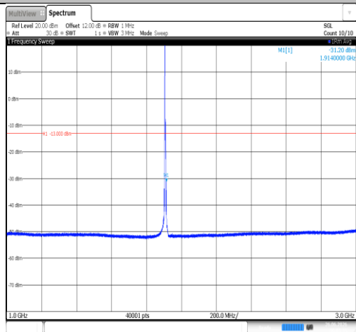
Band2-5MHz-QPSK-19175-1RB#0-1000~3000-PASS
