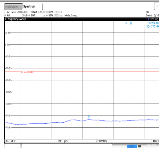
Band2-5MHz-QPSK-19175-1RB#0-30~1000-PASS
