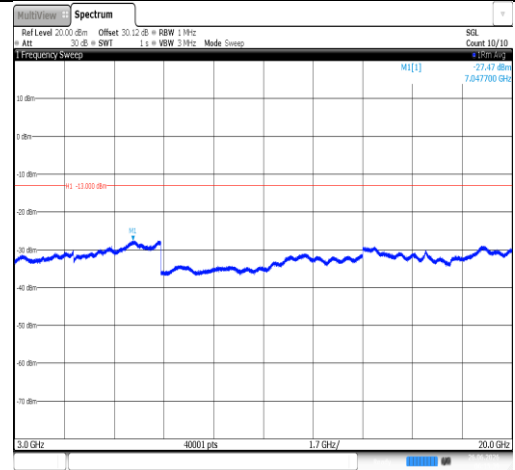
Band2-10MHz-16QAM-18900-1RB#0-3000~20000-PASS
