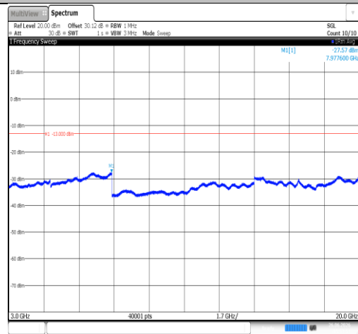
Band2-3MHz-16QAM-18900-1RB#0-3000~20000-PASS
