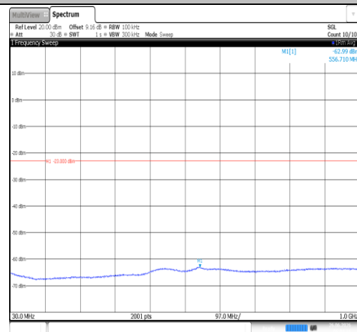
Band2-5MHz-16QAM-18900-1RB#0-30~1000-PASS
