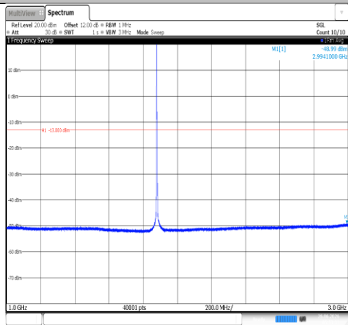
Band2-3MHz-16QAM-18900-1RB#0-1000~3000-PASS
