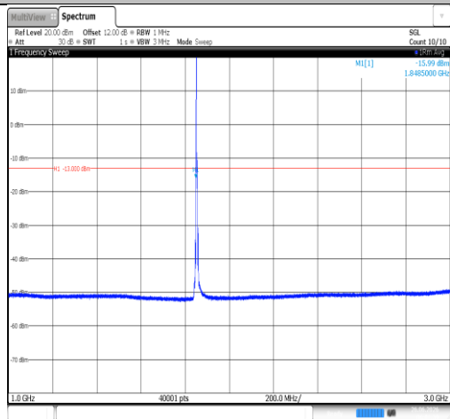
Band2-5MHz-QPSK-18625-1RB#0-1000~3000-PASS
