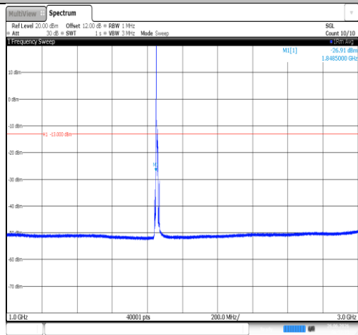
Band2-10MHz-QPSK-18650-1RB#0-1000~3000-PASS
