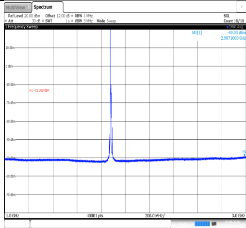
Band2-10MHz-16QAM-18900-1RB#0-1000~3000-PASS
