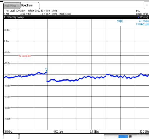
Band2-10MHz-QPSK-18650-1RB#0-3000~20000-PASS
