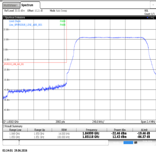
Band25-1.4MHz-QPSK-26683-1RB#5-PASS
