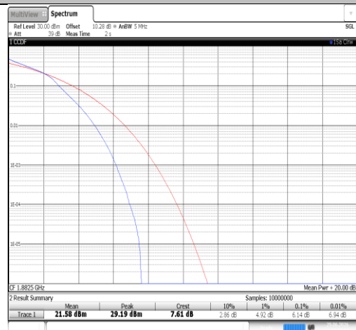
Band25-5MHz-16QAM-26365-25RB#0-PASS
