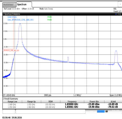
Band25-10MHz-16QAM-26090-50RB#0-PASS
