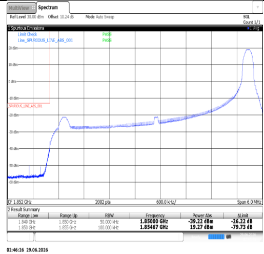
Band25-5MHz-16QAM-26665-1RB#0-PASS
