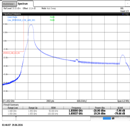
Band25-5MHz-16QAM-26065-25RB#0-PASS
