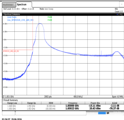
Band25-3MHz-QPSK-26055-15RB#0-PASS
