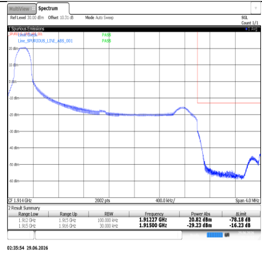
Band25-3MHz-16QAM-26675-15RB#0-PASS
