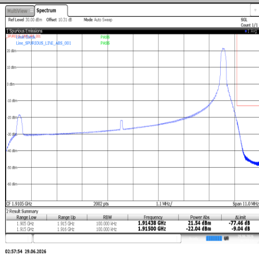
Band25-10MHz-16QAM-26090-1RB#0-PASS
