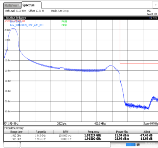
Band25-3MHz-QPSK-26675-15RB#0-PASS
