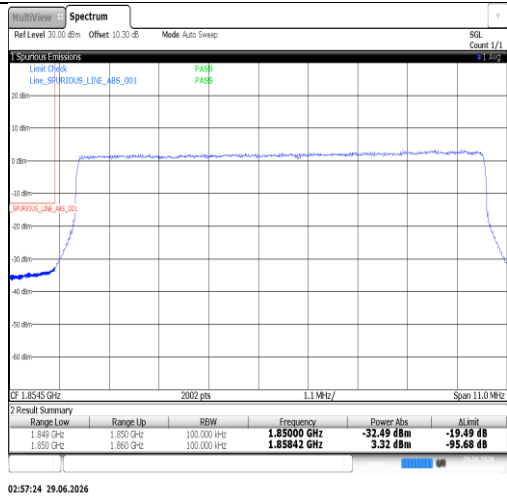
Band25-10MHz-16QAM-26640-1RB#49-PASS
