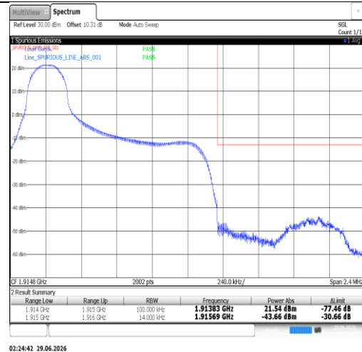
Band25-1.4MHz-16QAM-26683-6RB#0-PASS
