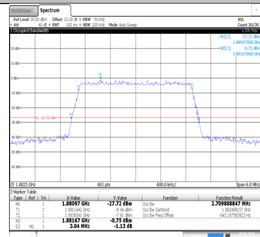
Band25-3MHz-16QAM-26365-15RB#0-PASS
