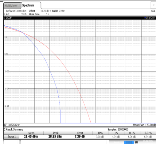
Band25-1.4MHz-16QAM-26365-6RB#0-PASS
