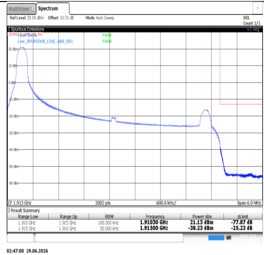
Band25-5MHz-QPSK-26665-25RB#0-PASS
