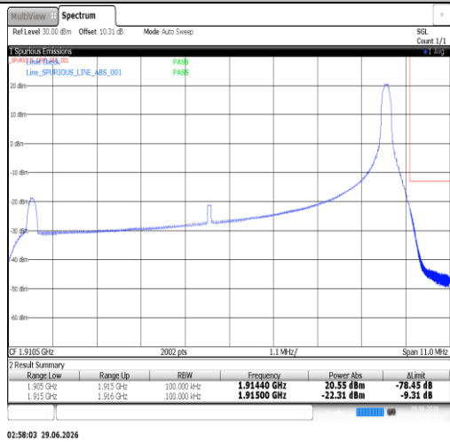
Band25-15MHz-QPSK-26115-1RB#0-PASS
