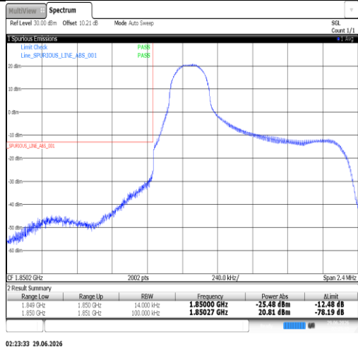
Band25-1.4MHz-16QAM-26047-6RB#0-PASS
