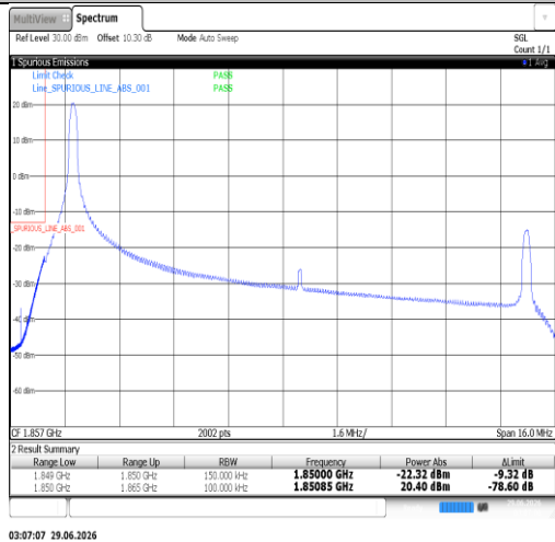
Band25-15MHz-QPSK-26115-75RB#0-PASS
