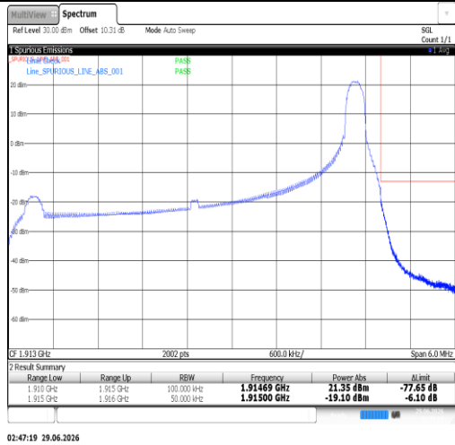
Band25-5MHz-16QAM-26065-1RB#0-PASS
