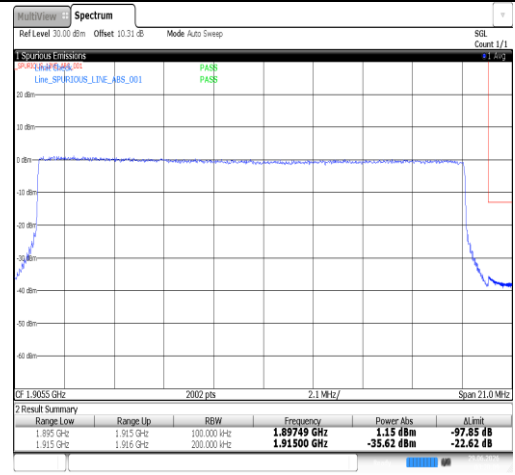
Band25-20MHz-16QAM-26590-100RB#0-PASS
