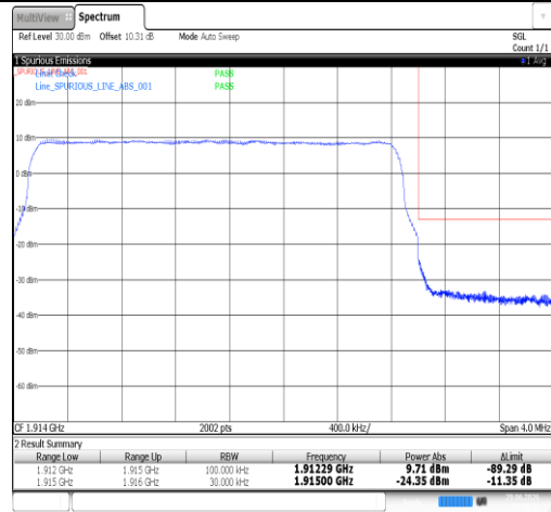
Band25-3MHz-QPSK-26675-15RB#0-PASS
