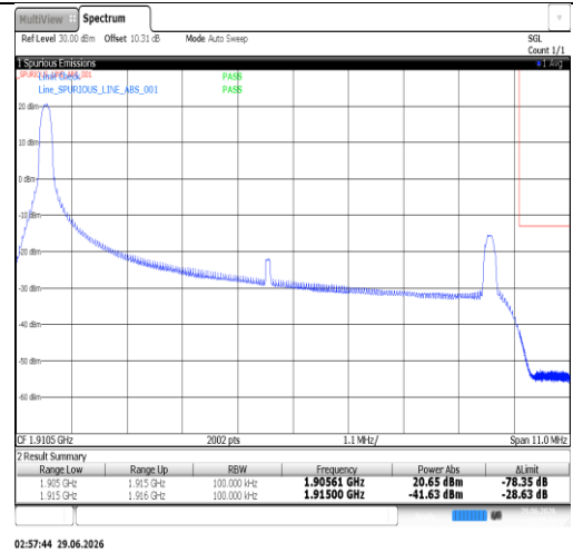
Band25-10MHz-16QAM-26640-50RB#0-PASS
