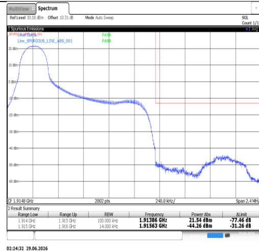
Band25-1.4MHz-QPSK-26683-6RB#0-PASS
