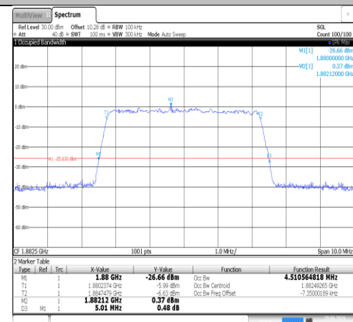
Band25-5MHz-16QAM-26365-25RB#0-PASS
