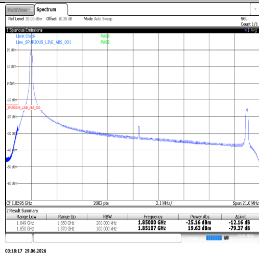
Band25-20MHz-16QAM-26140-100RB#0-PASS
