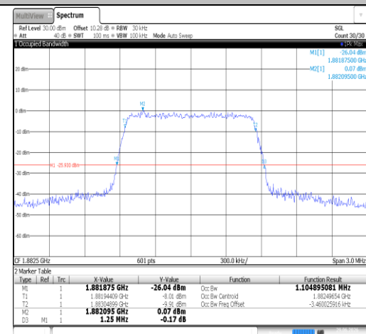
Band25-1.4MHz-16QAM-26365-6RB#0-PASS
