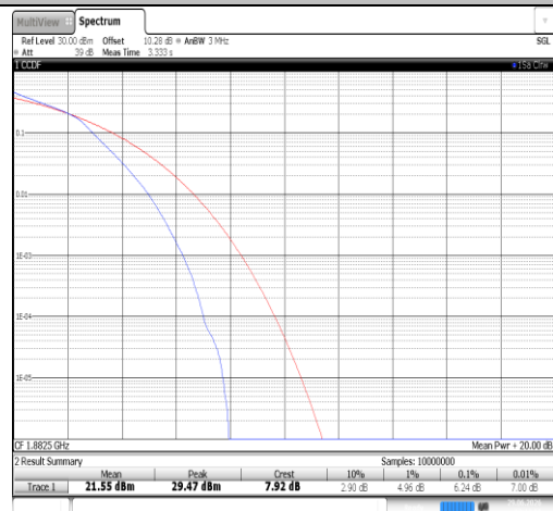
Band25-3MHz-16QAM-26365-15RB#0-PASS
