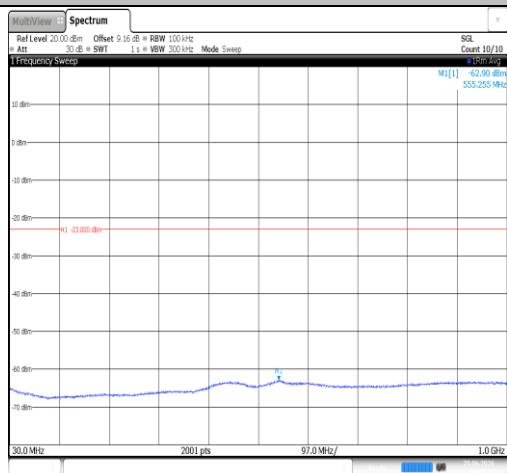
Band25-15MHz-QPSK-26115-1RB#0-30~1000-PASS
