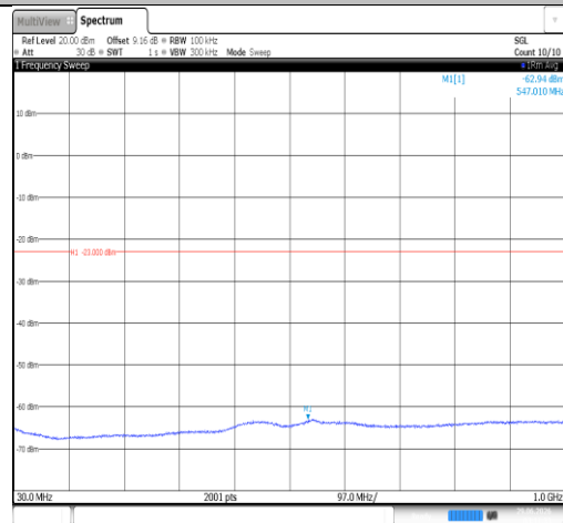
Band25-15MHz-QPSK-26365-1RB#0-30~1000-PASS
