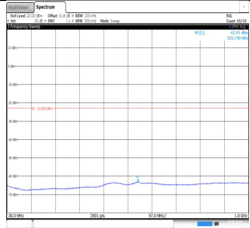
Band25-20MHz-16QAM-26140-1RB#0-30~1000-PASS
