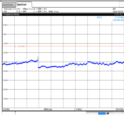
Band25-5MHz-QPSK-26665-1RB#0-3000~20000-PASS
