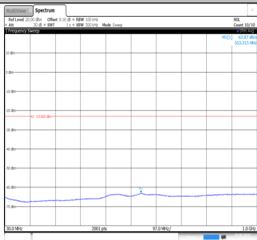
Band25-10MHz-QPSK-26090-1RB#0-30~1000-PASS
