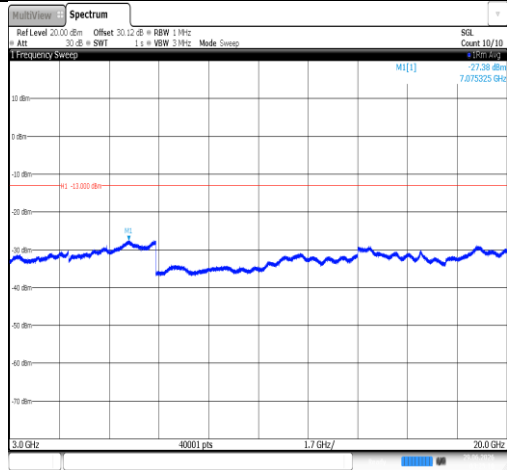
Band25-20MHz-QPSK-26590-1RB#0-3000~20000-PASS
