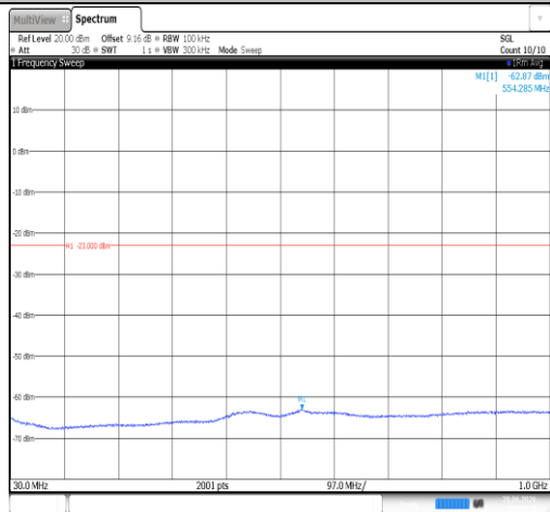
Band25-20MHz-QPSK-26140-1RB#0-30~1000-PASS
