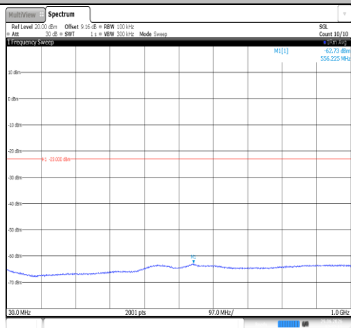
Band25-5MHz-QPSK-26665-1RB#0-30~1000-PASS
