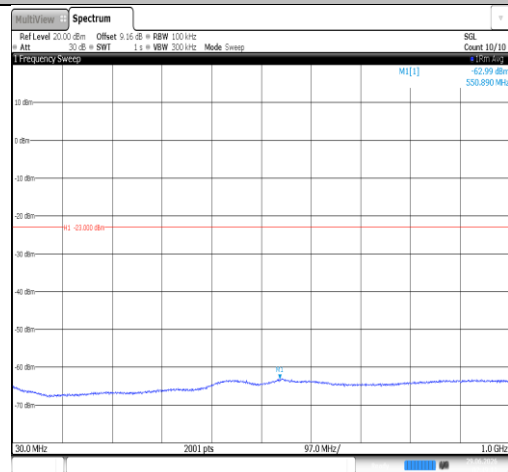
Band25-5MHz-16QAM-26065-1RB#0-30~1000-PASS
