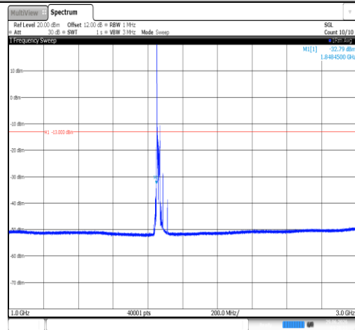
Band25-20MHz-QPSK-26140-1RB#0-1000~3000-PASS
