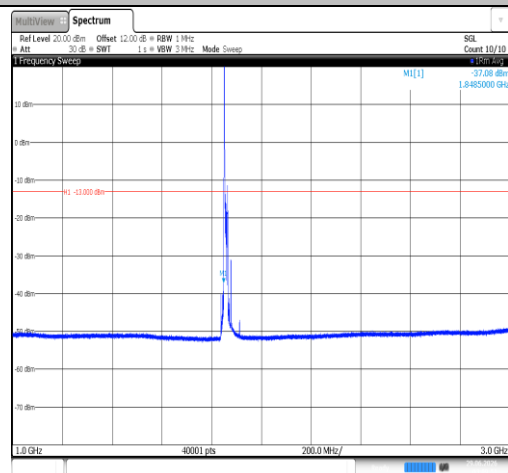
Band25-15MHz-QPSK-26115-1RB#0-1000~3000-PASS
