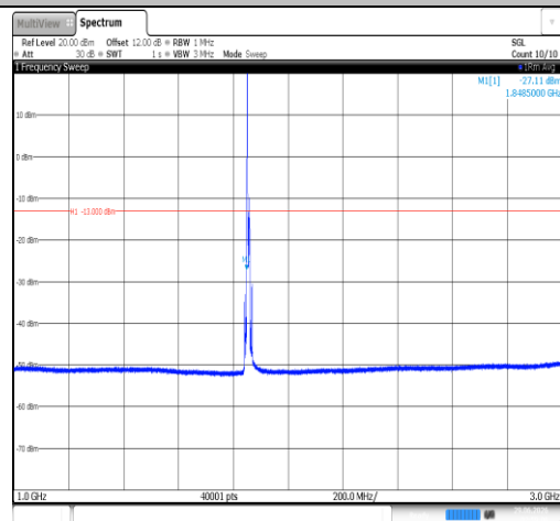
Band25-10MHz-QPSK-26090-1RB#0-1000~3000-PASS
