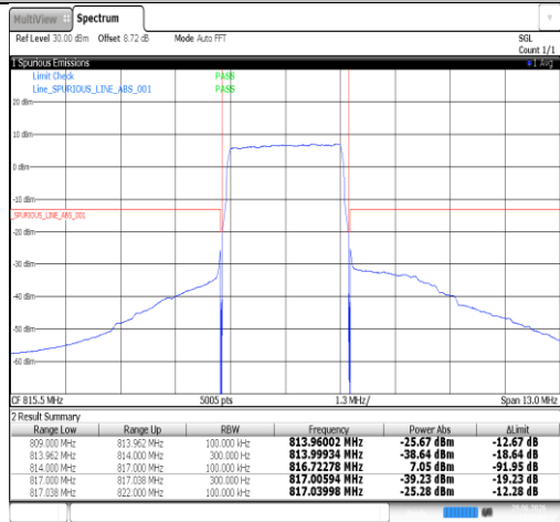
Band26(814-824)-3MHz-16QAM-26705-15RB#0-PASS
