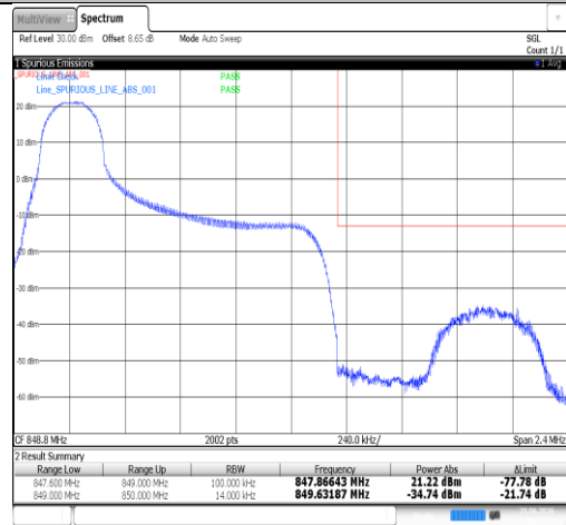
Band26(824-849)-1.4MHz-16QAM-27033-1RB#0-PASS
