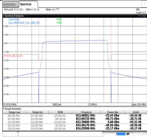
Band26(814-824)-10MHz-QPSK-26740-50RB#0-PASS
