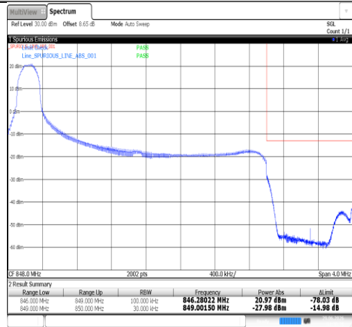
Band26(824-849)-3MHz-16QAM-27025-1RB#0-PASS
