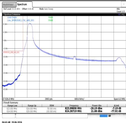
Band26(824-849)-5MHz-QPSK-26815-25RB#0-PASS
