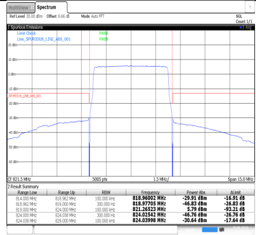
Band26(814-824)-10MHz-QPSK-26740-1RB#49-PASS
