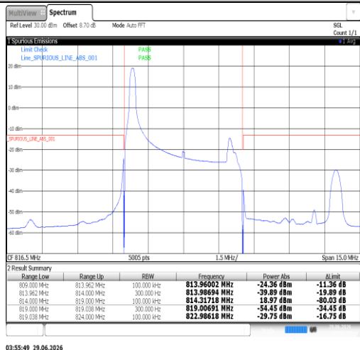
Band26(814-824)-5MHz-16QAM-26715-25RB#0-PASS
