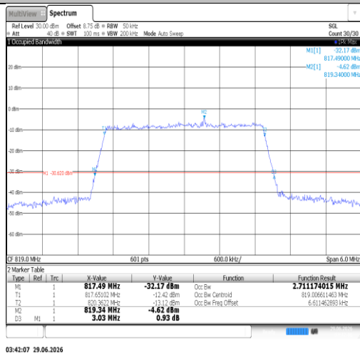
Band26(814-824)-5MHz-QPSK-26740-25RB#0-PASS
