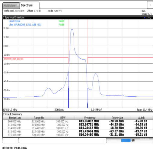
Band26(814-824)-1.4MHz-16QAM-26697-6RB#0-PASS
