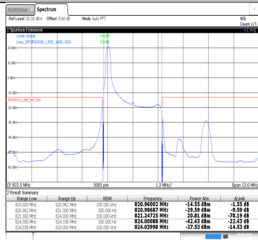
Band26(814-824)-3MHz-QPSK-26775-1RB#0-PASS
