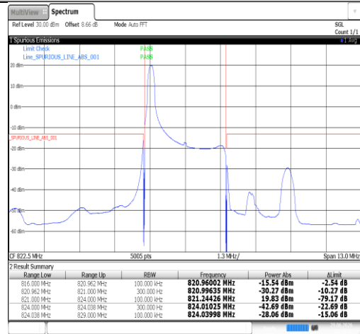
Band26(814-824)-3MHz-16QAM-26705-15RB#14-PASS
