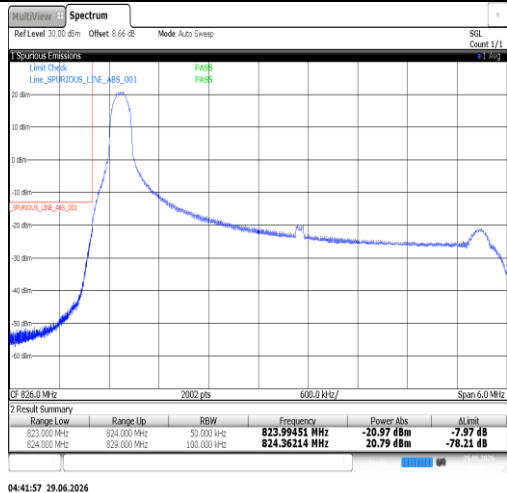
Band26(824-849)-5MHz-16QAM-26815-25RB#0-PASS
