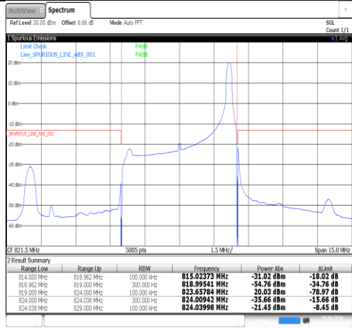
Band26(814-824)-10MHz-QPSK-26740-1RB#0-PASS
