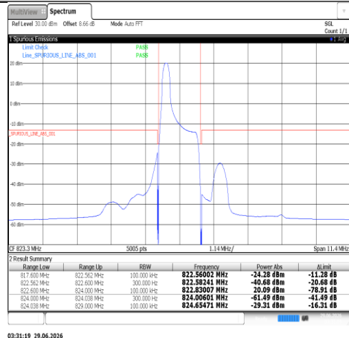
Band26(814-824)-1.4MHz-16QAM-26783-6RB#0-PASS
