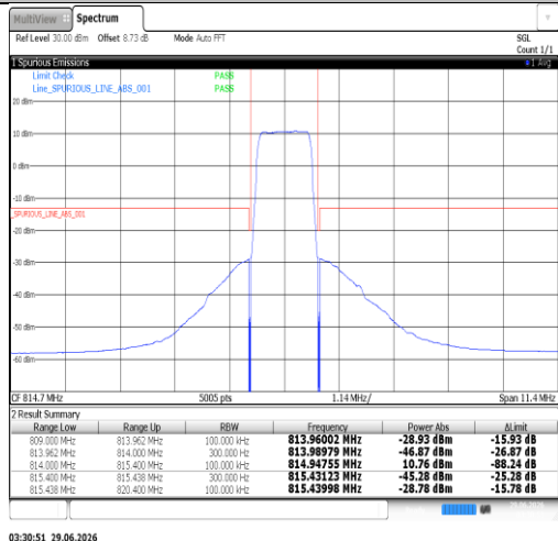
Band26(814-824)-1.4MHz-16QAM-26783-1RB#5-PASS
