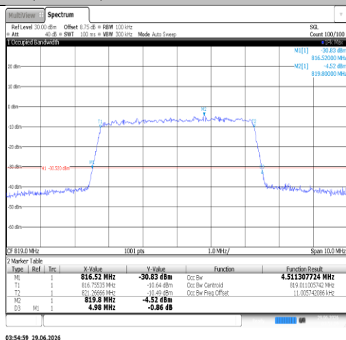
Band26(814-824)-10MHz-QPSK-26740-50RB#0-PASS
