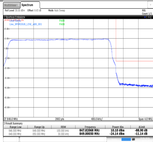
Band26(824-849)-3MHz-16QAM-26805-1RB#14-PASS
