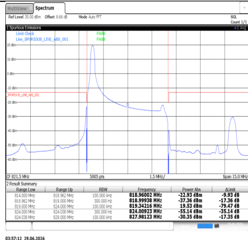
Band26(814-824)-5MHz-16QAM-26765-25RB#0-PASS
