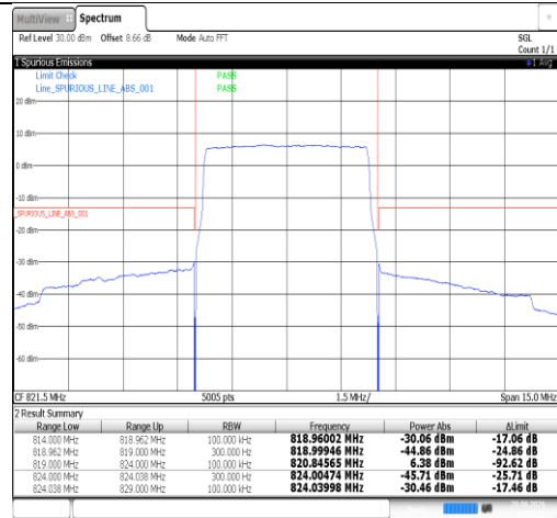
Band26(814-824)-5MHz-16QAM-26715-1RB#24-PASS
