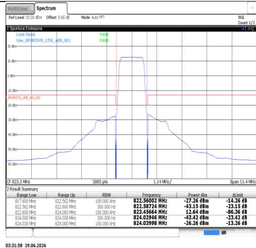
Band26(814-824)-1.4MHz-16QAM-26697-1RB#5-PASS
