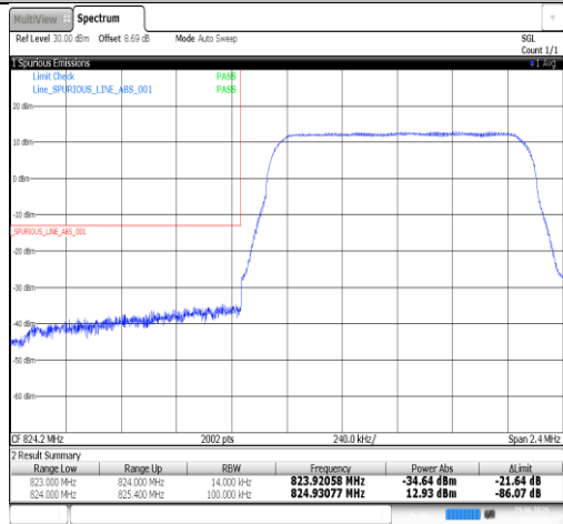
Band26(824-849)-1.4MHz-16QAM-26797-6RB#0-PASS
