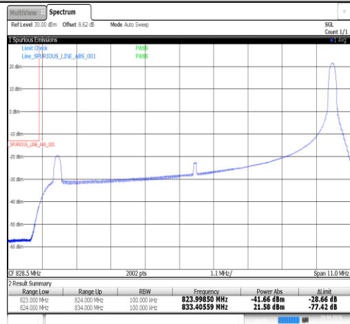
Band26(824-849)-10MHz-QPSK-26840-1RB#49-PASS
