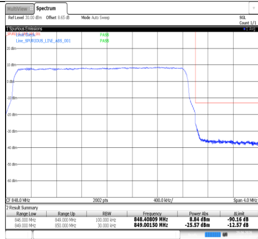
Band26(824-849)-5MHz-QPSK-26815-1RB#24-PASS
