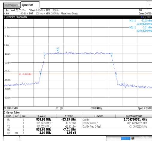
Band26(824-849)-3MHz-16QAM-26915-15RB#0-PASS
