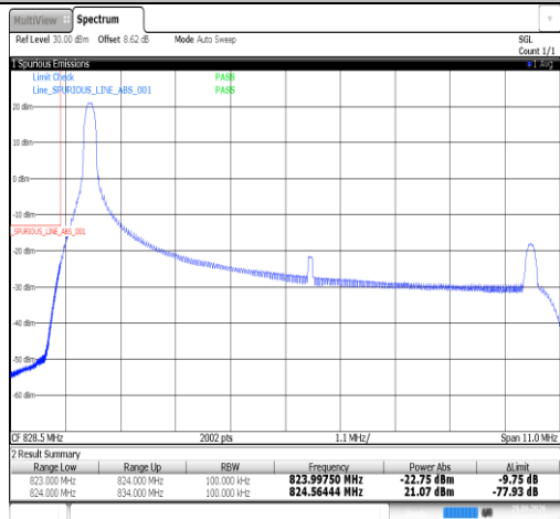
Band26(824-849)-10MHz-QPSK-26840-1RB#0-PASS
