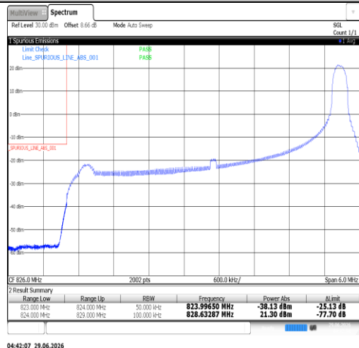
Band26(824-849)-5MHz-QPSK-27015-1RB#0-PASS
