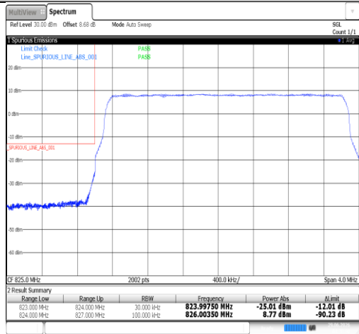
Band26(824-849)-3MHz-16QAM-26805-15RB#0-PASS
