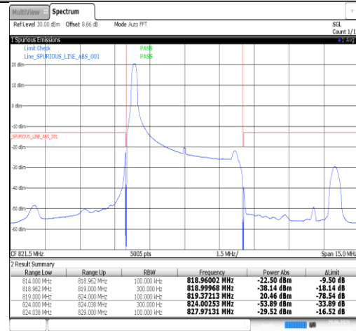
Band26(814-824)-5MHz-QPSK-26765-1RB#0-PASS
