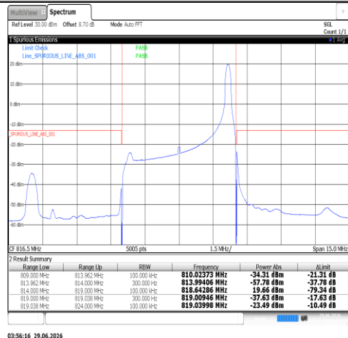
Band26(814-824)-5MHz-16QAM-26765-1RB#0-PASS
