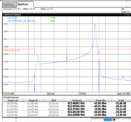
Band26(824-849)-1.4MHz-QPSK-26797-1RB#0-PASS
