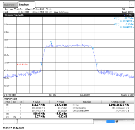
Band26(814-824)-3MHz-16QAM-26740-15RB#0-PASS
