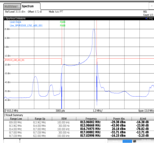
Band26(814-824)-3MHz-QPSK-26705-1RB#14-PASS
