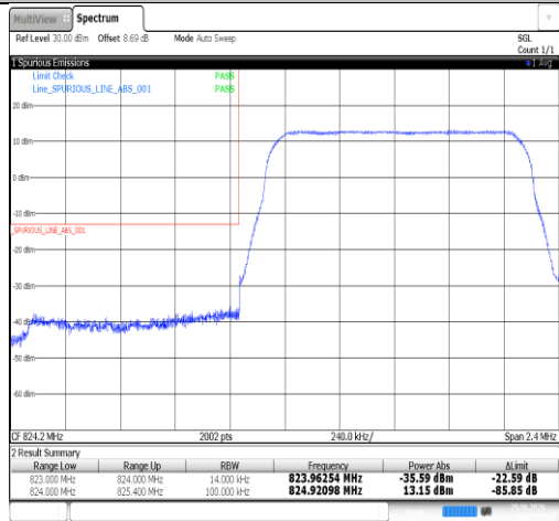
Band26(824-849)-1.4MHz-QPSK-26797-6RB#0-PASS
