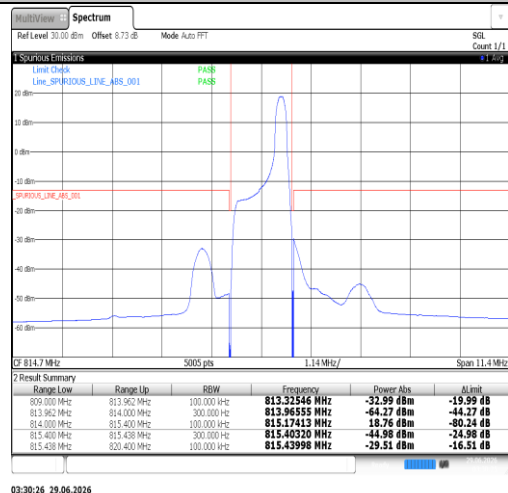
Band26(814-824)-1.4MHz-16QAM-26783-1RB#0-PASS
