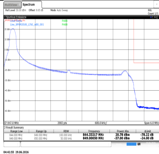
Band26(824-849)-5MHz-16QAM-27015-25RB#0-PASS
