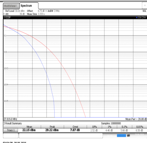
Band26(814-824)-10MHz-QPSK-26740-50RB#0-PASS
