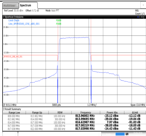
Band26(814-824)-3MHz-QPSK-26705-15RB#0-PASS
