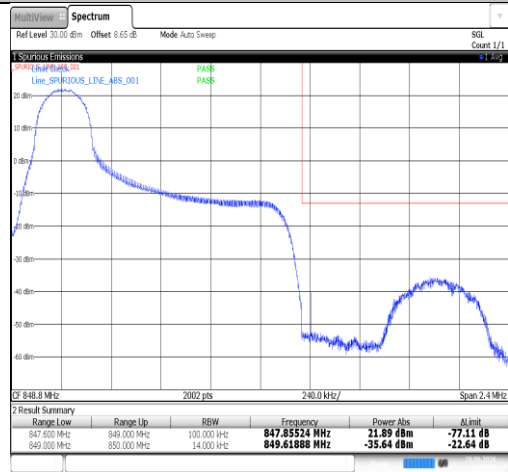
Band26(824-849)-1.4MHz-QPSK-27033-1RB#0-PASS
