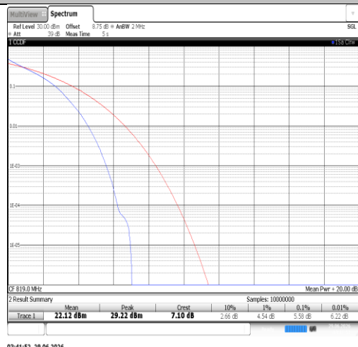
Band26(814-824)-5MHz-QPSK-26740-25RB#0-PASS
