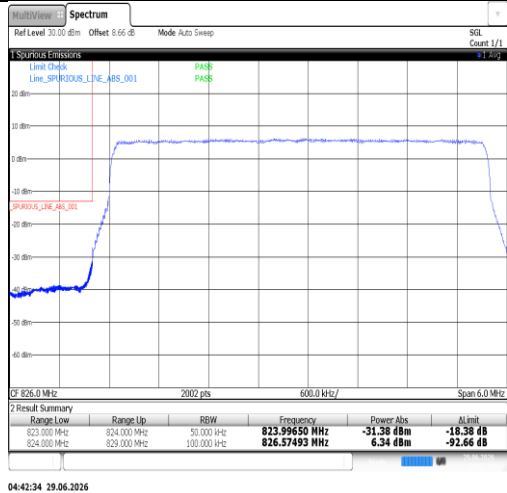
Band26(824-849)-5MHz-16QAM-27015-1RB#24-PASS
