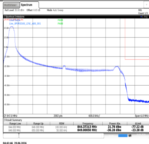
Band26(824-849)-5MHz-QPSK-27015-25RB#0-PASS
