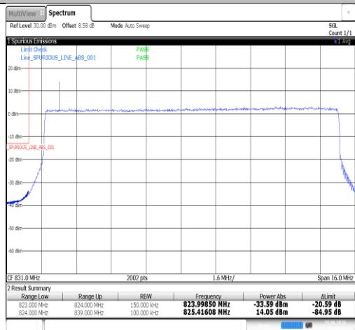
Band26(824-849)-15MHz-QPSK-26865-75RB#0-PASS
