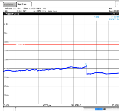
Band26(824-849)-3MHz-16QAM-27025-1RB#0-3000~10000-PASS
