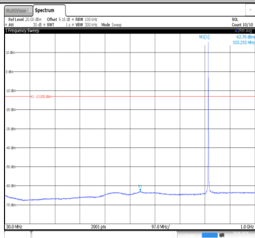
Band26(814-824)-1.4MHz-16QAM-26740-1RB#0-30~1000- PASS
