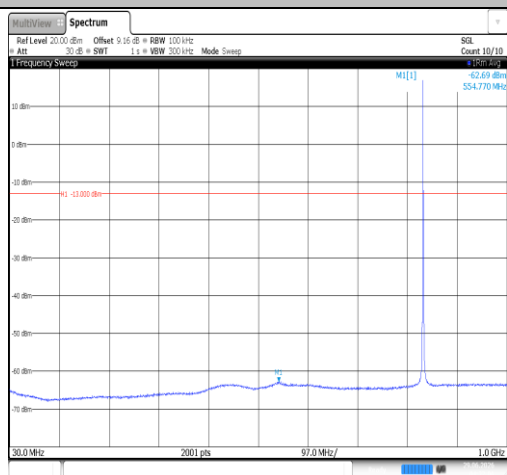
Band26(824-849)-1.4MHz-16QAM-26915-1RB#0-30~1000- PASS
