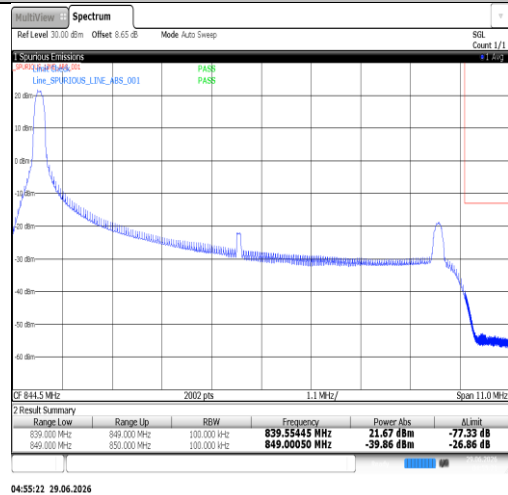
Band26(824-849)-10MHz-16QAM-26990-1RB#49-PASS
