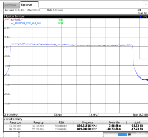
Band26(824-849)-15MHz-16QAM-26865-1RB#74-PASS
