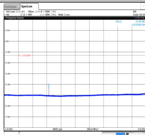
Band26(814-824)-10MHz-QPSK-26740-1RB#0- 1000~3000-PASS
