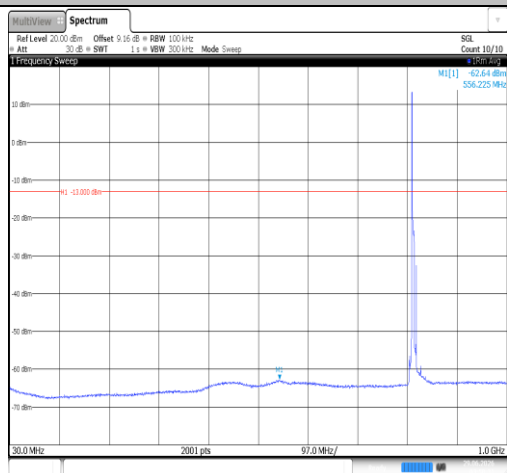
Band26(814-824)-5MHz-QPSK-26715-1RB#0-30~1000-PASS
