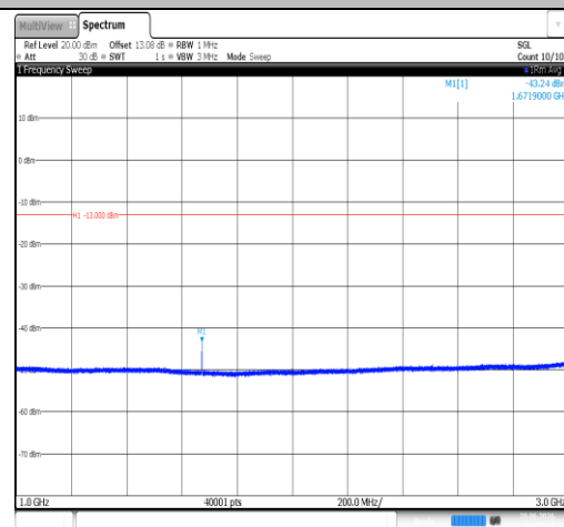
Band26(824-849)-1.4MHz-16QAM-26915-1RB#0- 1000~3000-PASS
