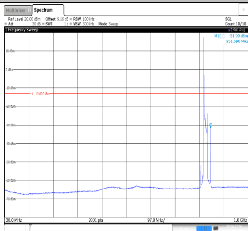
Band26(824-849)-15MHz-QPSK-26865-1RB#0-30~1000- PASS
