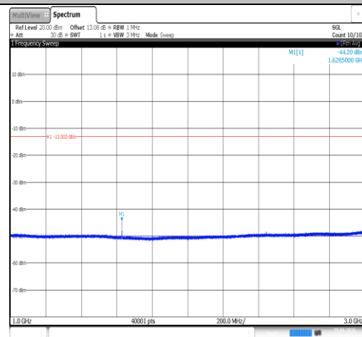
Band26(814-824)-3MHz-QPSK-26705-1RB#0-1000~3000-PASS
