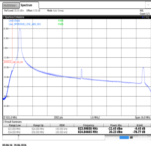
Band26(824-849)-15MHz-16QAM-26865-75RB#0-PASS
