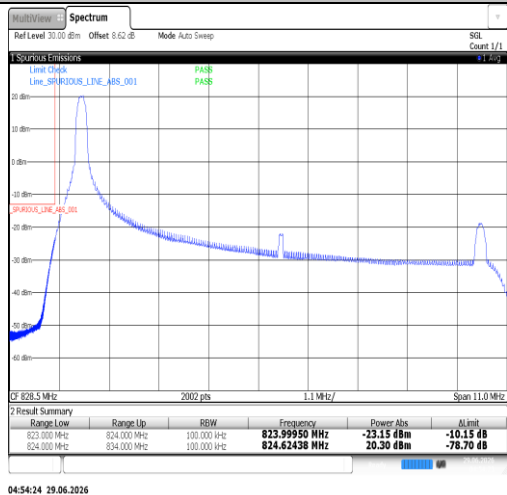
Band26(824-849)-10MHz-16QAM-26840-50RB#0-PASS
