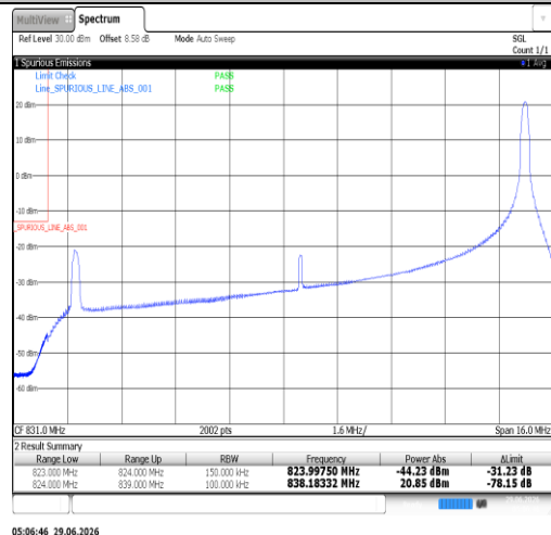
Band26(824-849)-15MHz-16QAM-26965-1RB#0-PASS
