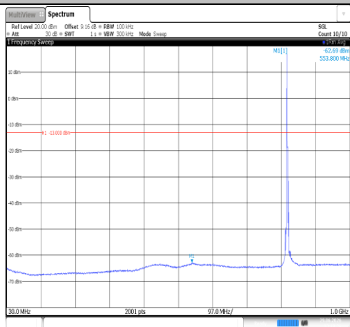
Band26(814-824)-3MHz-QPSK-26775-1RB#0-30~1000-PASS
