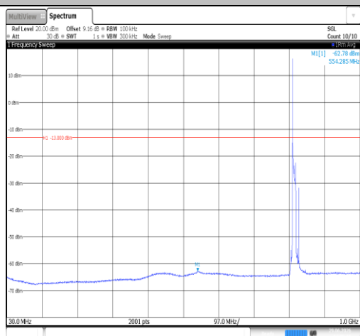
Band26(814-824)-10MHz-QPSK-26740-1RB#0-30~1000- PASS
