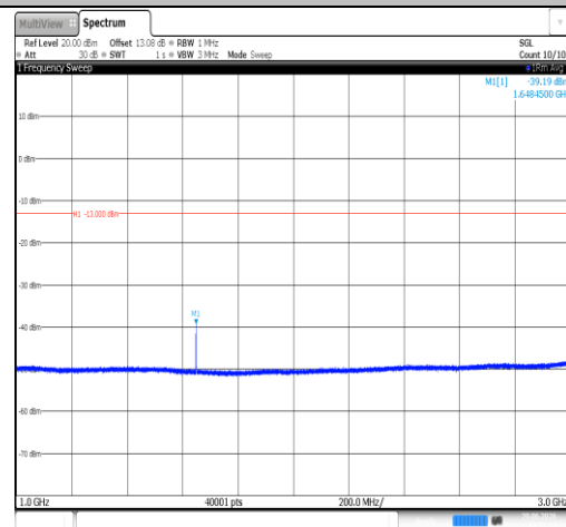
Band26(824-849)-3MHz-QPSK-26805-1RB#0-1000~3000- PASS
