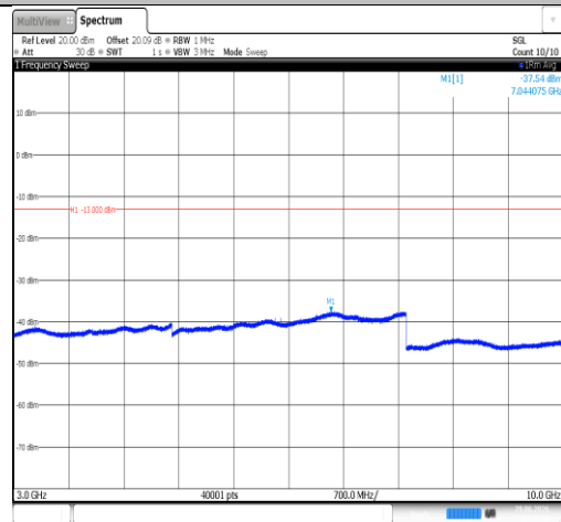
Band26(814-824)-3MHz-QPSK-26740-1RB#0-3000~10000-PASS
