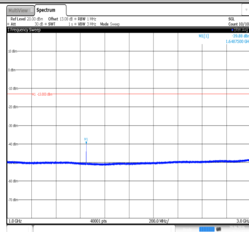
Band26(824-849)-5MHz-QPSK-26815-1RB#0-1000~3000-PASS
