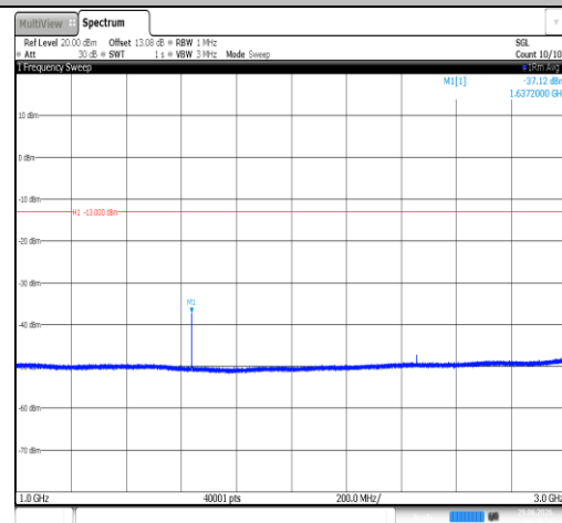
Band26(814-824)-1.4MHz-16QAM-26740-1RB#0- 1000~3000-PASS
