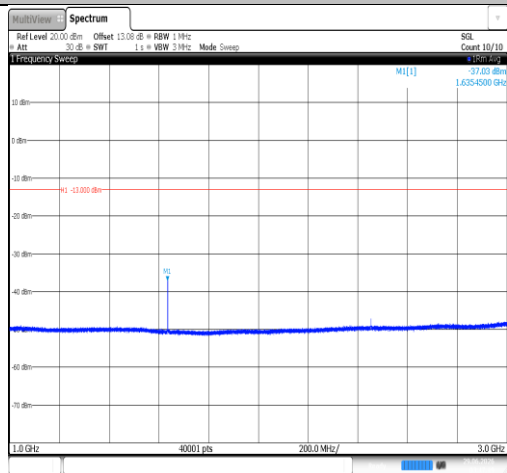
Band26(814-824)-3MHz-QPSK-26740-1RB#0-1000~3000-PASS
