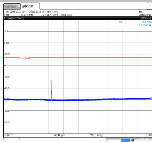
Band26(814-824)-3MHz-QPSK-26775-1RB#0-1000~3000-PASS
