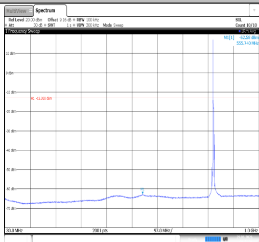
Band26(824-849)-3MHz-QPSK-26805-1RB#0-30~1000- PASS
