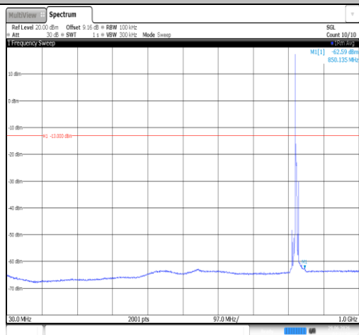
Band26(824-849)-5MHz-QPSK-26815-1RB#0-30~1000-PASS
