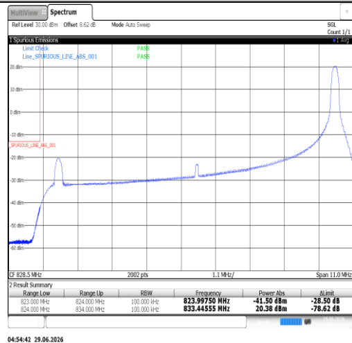
Band26(824-849)-10MHz-16QAM-26840-50RB#49-PASS
