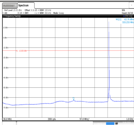
Band26(814-824)-3MHz-QPSK-26705-1RB#0-30~1000-PASS
