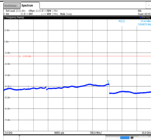
Band26(824-849)-10MHz-QPSK-26915-1RB#0-3000~10000-PASS
