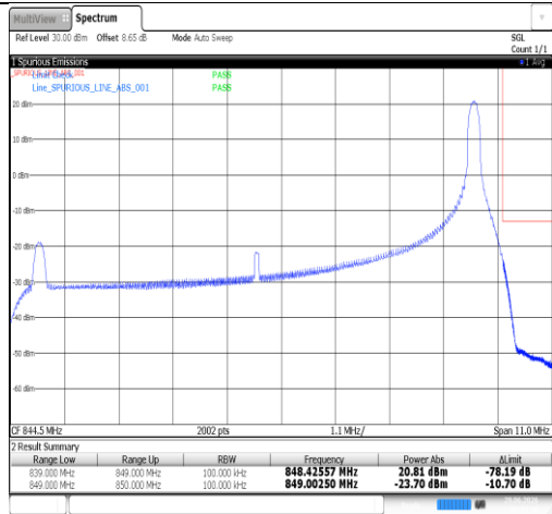
Band26(824-849)-15MHz-QPSK-26865-1RB#0-PASS
