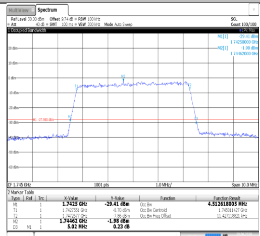
Band66-5MHz-16QAM-132322-25RB#0-PASS
