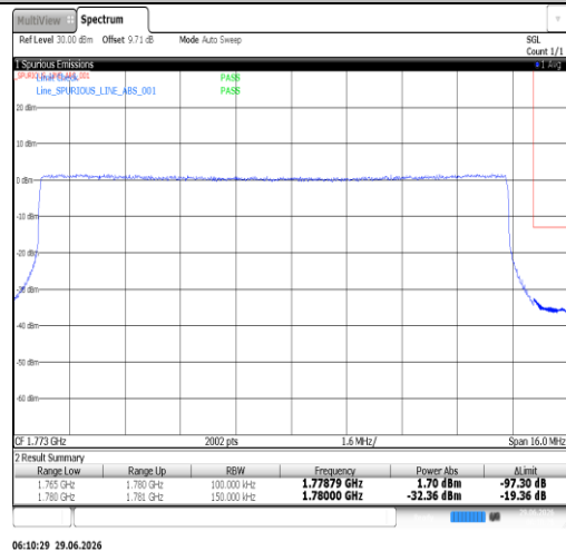
Band66-15MHz-16QAM-132047-1RB#74-PASS
