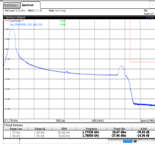
Band66-5MHz-QPSK-132647-25RB#0-PASS
