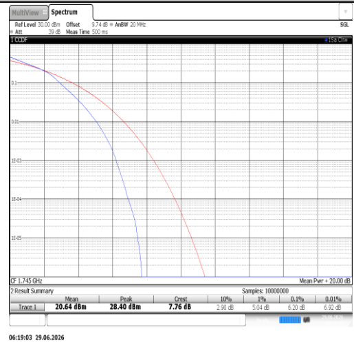
Band66-20MHz-16QAM-132322-100RB#0-PASS
