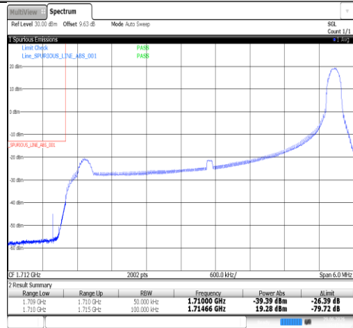
Band66-5MHz-16QAM-132647-1RB#0-PASS
