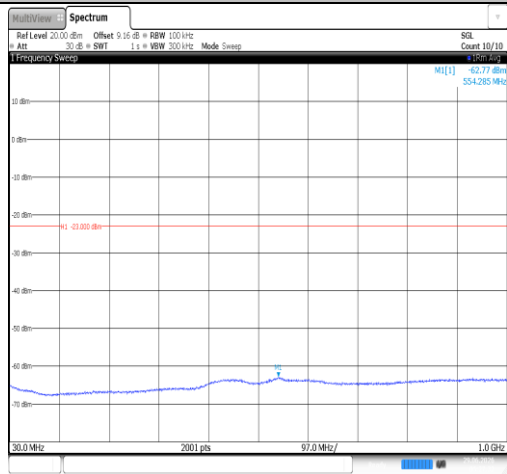
Band66-1.4MHz-16QAM-131979-1RB#0-30~1000-PASS
