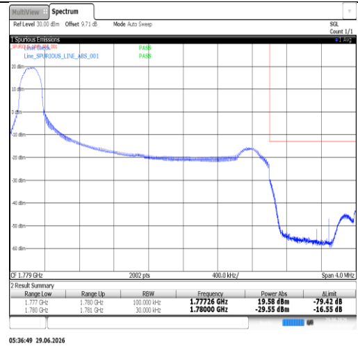
Band66-3MHz-16QAM-132657-15RB#0-PASS
