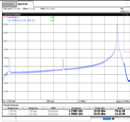
Band66-20MHz-16QAM-132572-1RB#99-PASS
