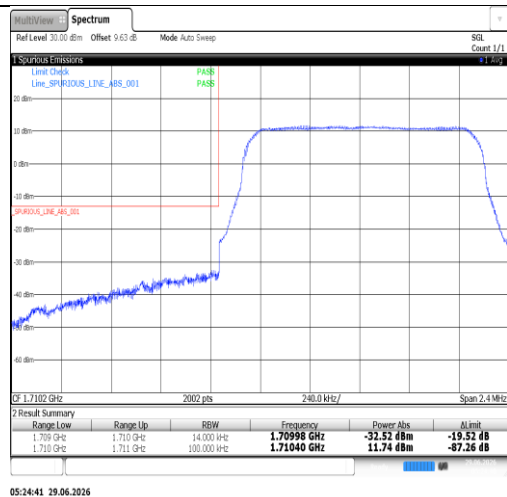
Band66-1.4MHz-16QAM-132665-1RB#5-PASS
