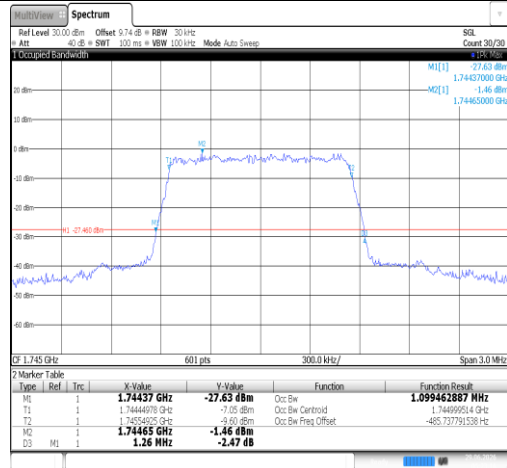
Band66-1.4MHz-QPSK-132322-6RB#0-PASS
