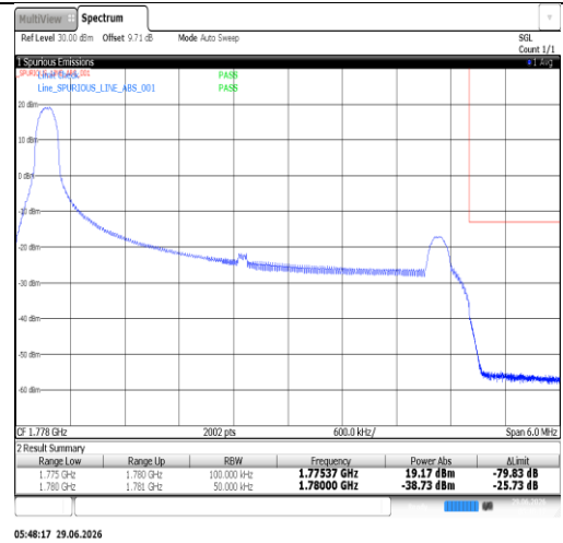
Band66-5MHz-16QAM-132647-25RB#0-PASS
