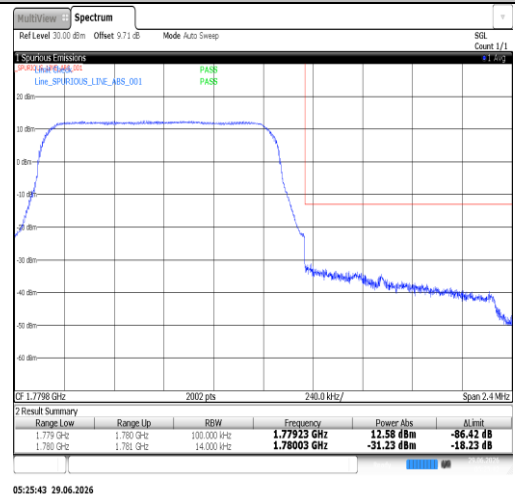
Band66-1.4MHz-16QAM-131979-1RB#5-PASS
