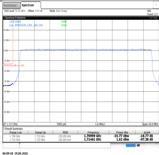
Band66-15MHz-QPSK-132597-1RB#74-PASS
