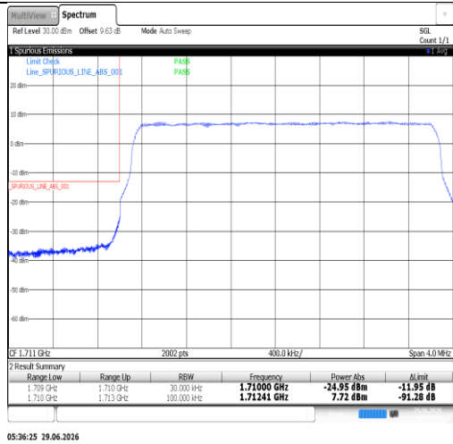
Band66-3MHz-16QAM-132657-1RB#14-PASS
