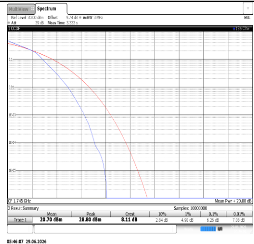
Band66-5MHz-16QAM-132322-25RB#0-PASS
