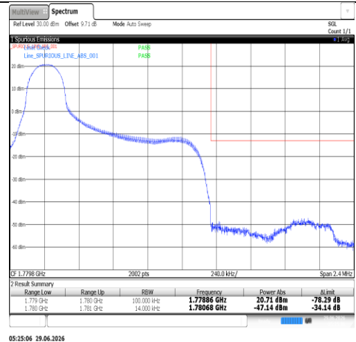
Band66-1.4MHz-QPSK-132665-6RB#0-PASS
