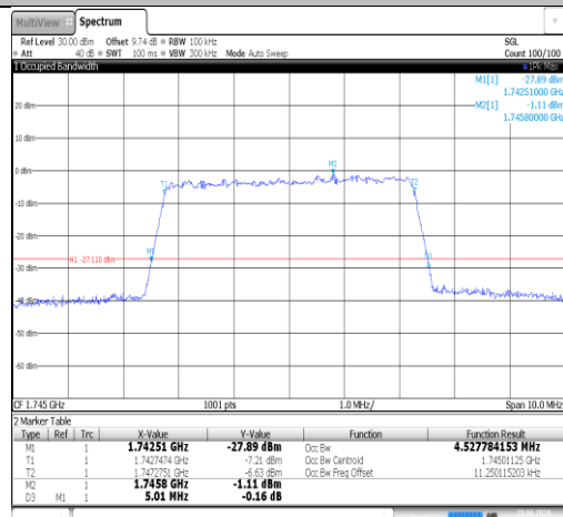
Band66-5MHz-QPSK-132322-25RB#0-PASS
