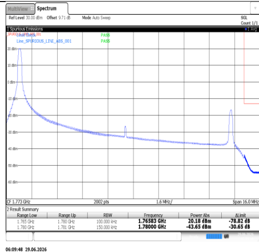
Band66-15MHz-QPSK-132597-75RB#0-PASS
