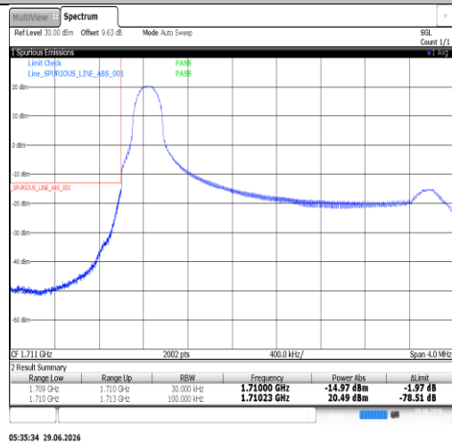
Band66-3MHz-QPSK-131987-15RB#0-PASS
