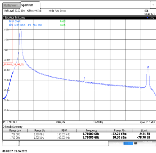
Band66-15MHz-QPSK-132047-75RB#0-PASS
