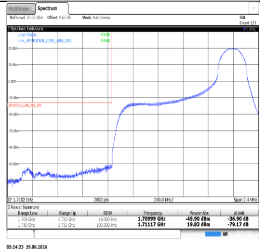
Band66-1.4MHz-16QAM-132665-1RB#0-PASS
