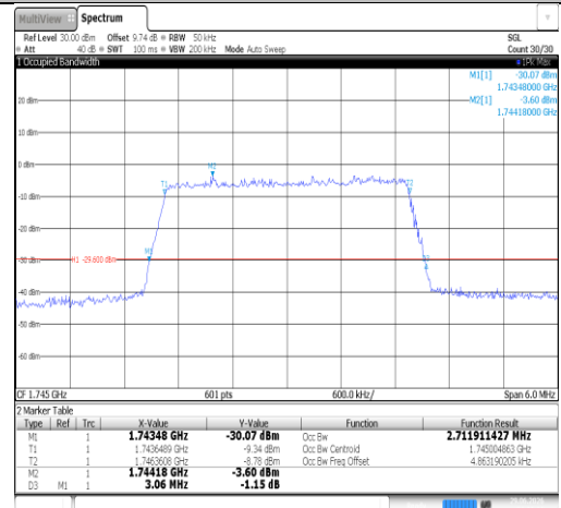
Band66-3MHz-16QAM-132322-15RB#0-PASS
