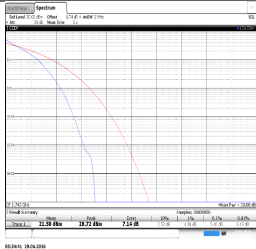
Band66-3MHz-QPSK-132322-15RB#0-PASS
