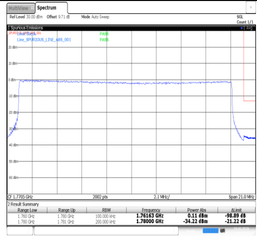
Band66-20MHz-16QAM-132572-100RB#0-PASS
