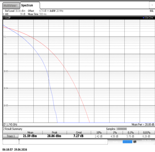
Band66-20MHz-QPSK-132322-100RB#0-PASS
