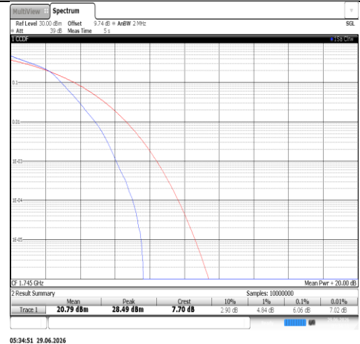
Band66-3MHz-16QAM-132322-15RB#0-PASS
