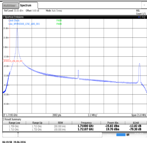
Band66-20MHz-16QAM-132072-100RB#0-PASS
