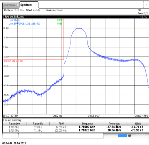
Band66-1.4MHz-16QAM-131979-6RB#0-PASS
