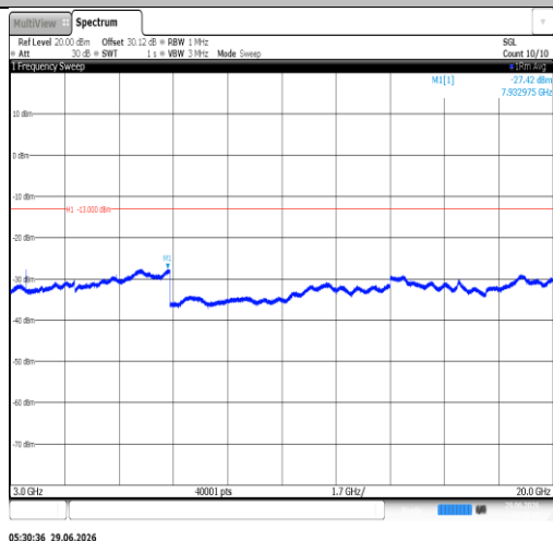
Band66-1.4MHz-16QAM-132322-1RB#0-3000~20000-PASS
