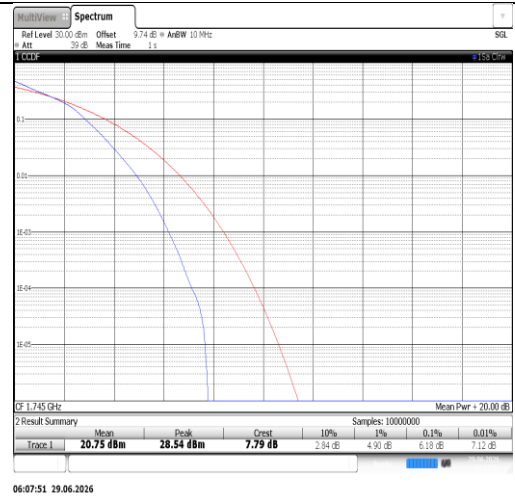
Band66-15MHz-16QAM-132322-75RB#0-PASS
