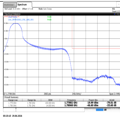
Band66-1.4MHz-16QAM-132665-6RB#0-PASS
