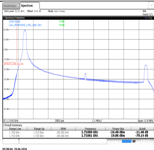
Band66-10MHz-16QAM-132022-50RB#0-PASS
