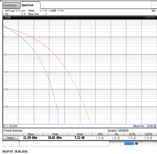
Band66-15MHz-QPSK-132322-75RB#0-PASS
