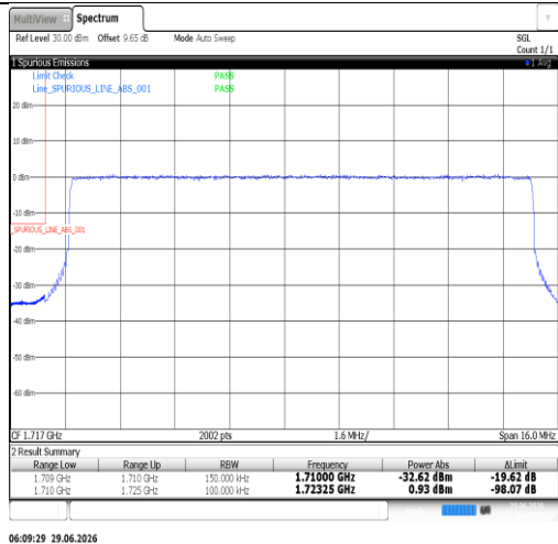
Band66-15MHz-16QAM-132597-1RB#74-PASS
