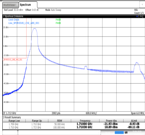
Band66-5MHz-16QAM-131997-25RB#0-PASS
