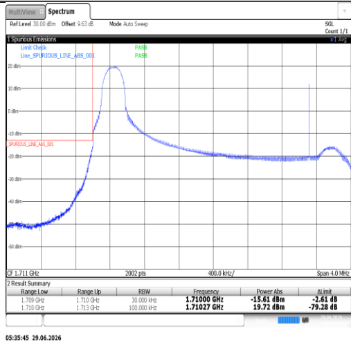
Band66-3MHz-16QAM-131987-15RB#0-PASS
