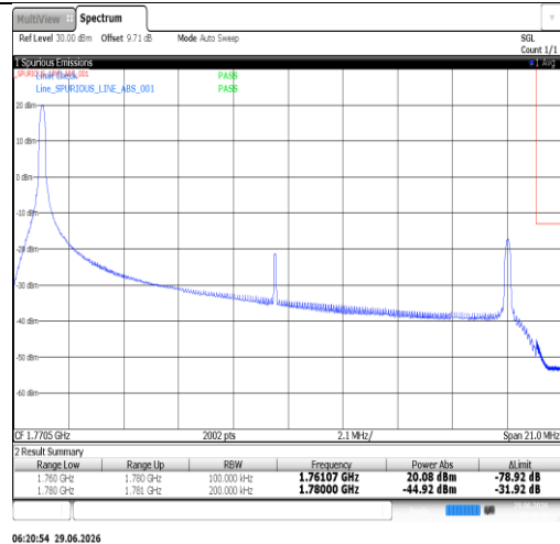
Band66-20MHz-QPSK-132572-100RB#0-PASS
