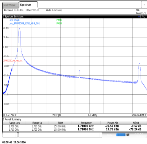
Band66-15MHz-16QAM-132047-75RB#0-PASS
