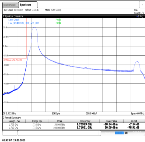
Band66-5MHz-QPSK-131997-25RB#0-PASS
