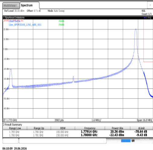
Band66-15MHz-16QAM-132047-1RB#0-PASS
