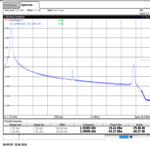
Band66-15MHz-16QAM-132597-75RB#0-PASS
