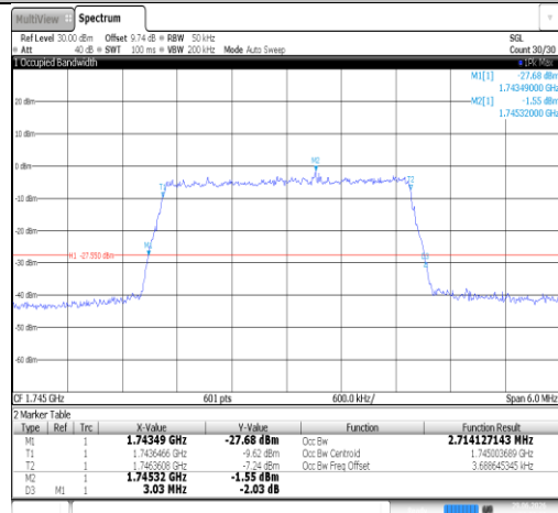
Band66-3MHz-QPSK-132322-15RB#0-PASS
