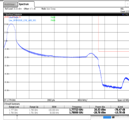
Band66-3MHz-QPSK-132657-15RB#0-PASS
