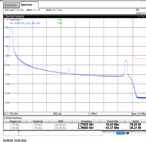
Band66-10MHz-QPSK-132622-50RB#0-PASS
