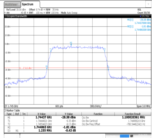
Band66-1.4MHz-16QAM-132322-6RB#0-PASS
