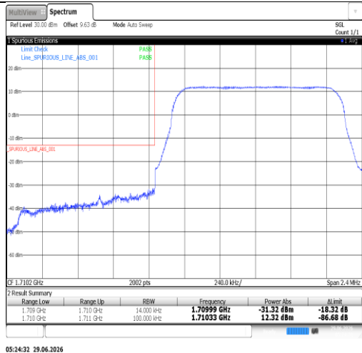
Band66-1.4MHz-QPSK-132665-1RB#5-PASS
