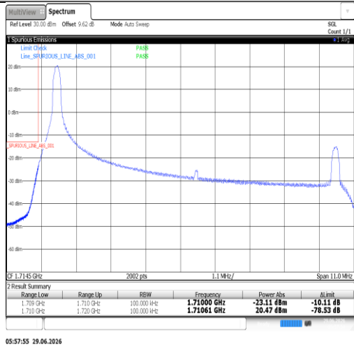
Band66-10MHz-QPSK-132022-50RB#0-PASS
