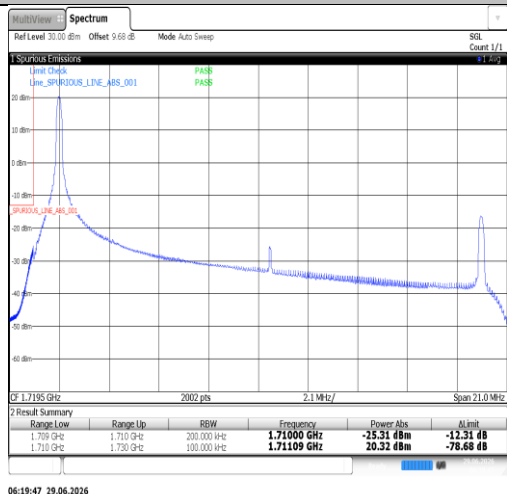
Band66-20MHz-QPSK-132072-100RB#0-PASS
