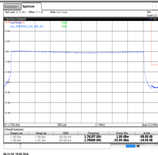
Band66-20MHz-16QAM-132072-1RB#99-PASS
