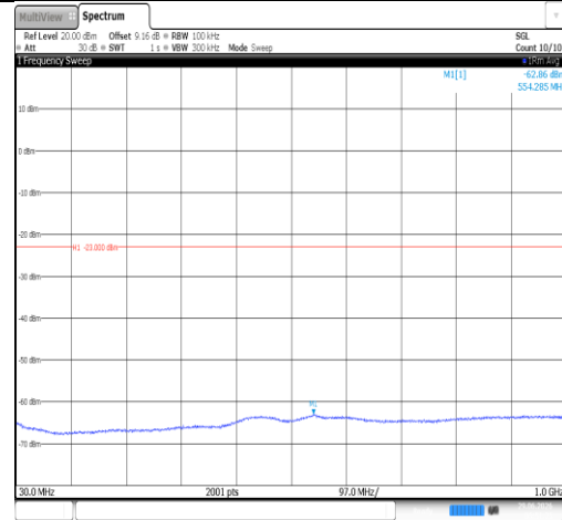
Band66-5MHz-QPSK-132322-1RB#0-30~1000-PASS
