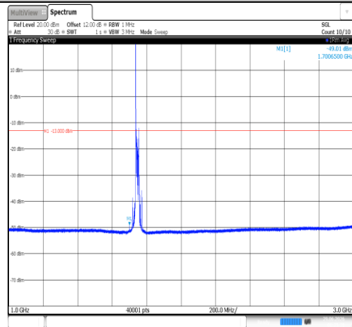
Band66-20MHz-16QAM-132322-1RB#0-1000~3000-PASS
