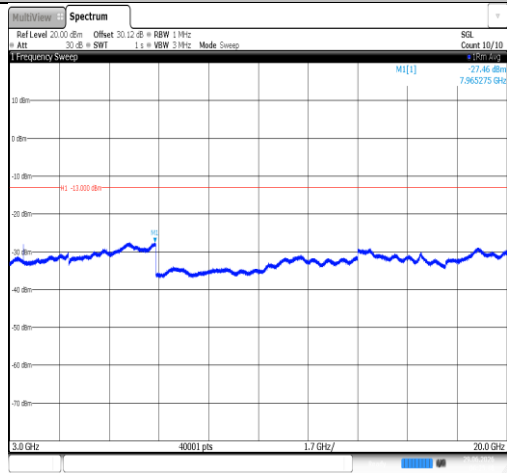
Band66-20MHz-16QAM-132322-1RB#0-3000~20000-PASS
