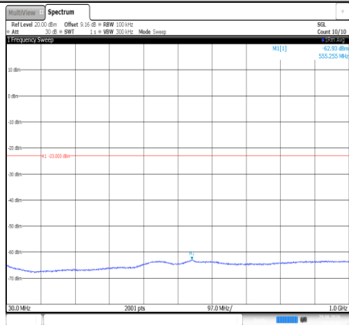
Band66-20MHz-16QAM-132322-1RB#0-30~1000-PASS
