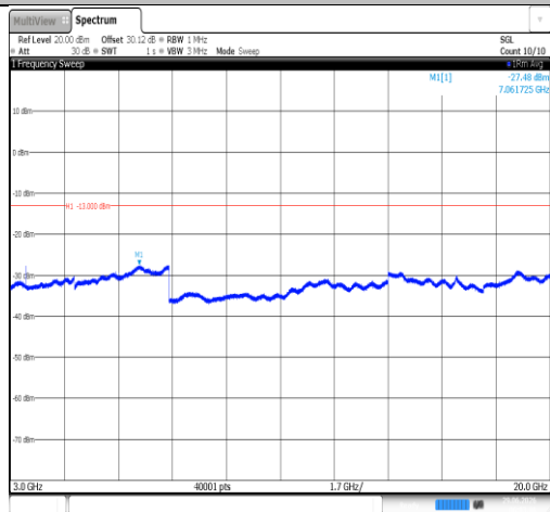
Band66-10MHz-16QAM-132322-1RB#0-3000~20000-PASS
