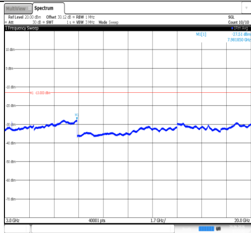
Band66-5MHz-16QAM-132322-1RB#0-3000~20000-PASS
