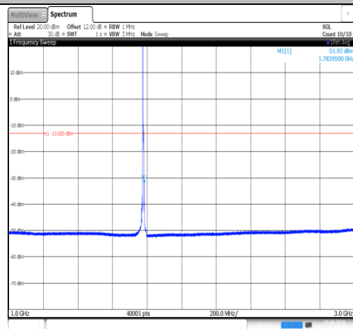
Band66-5MHz-QPSK-132647-1RB#0-1000~3000-PASS
