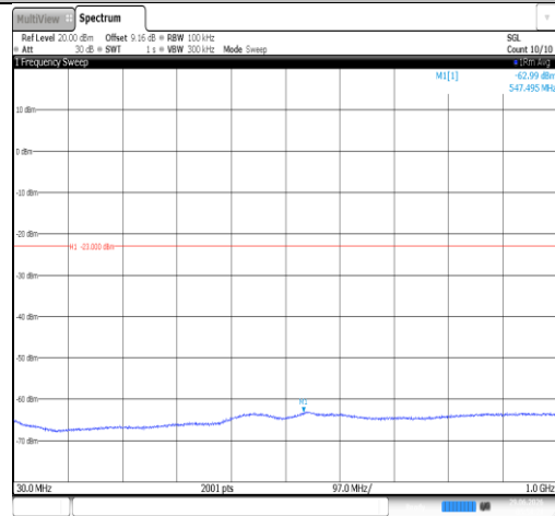
Band66-5MHz-16QAM-132647-1RB#0-30~1000-PASS
