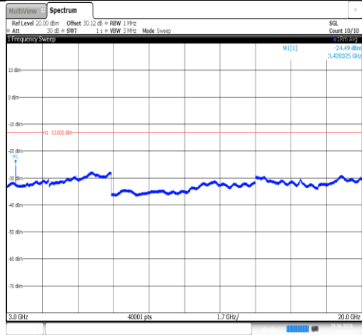
Band66-5MHz-QPSK-131997-1RB#0-3000~20000-PASS
