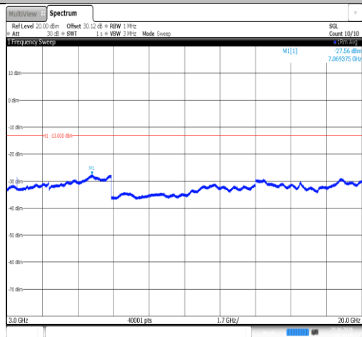
Band66-15MHz-16QAM-132322-1RB#0-3000~20000-PASS
