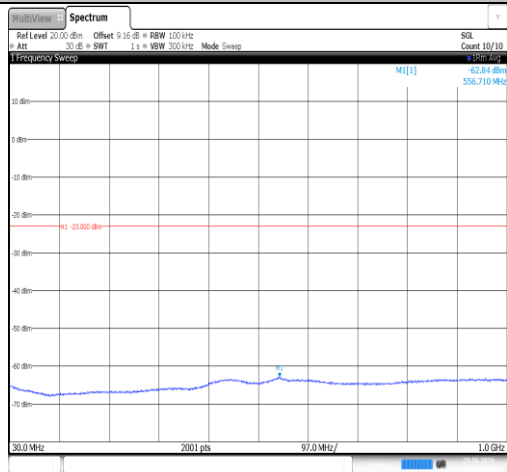
Band66-5MHz-16QAM-132322-1RB#0-30~1000-PASS
