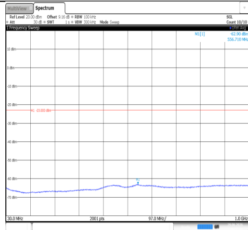
Band66-15MHz-16QAM-132047-1RB#0-30~1000-PASS
