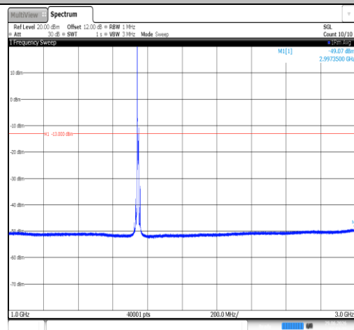
Band66-10MHz-16QAM-132322-1RB#0-1000~3000-PASS
