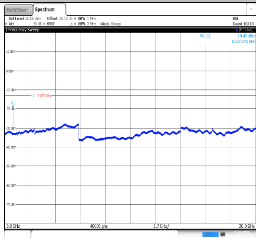
Band66-5MHz-QPSK-132647-1RB#0-3000~20000-PASS
