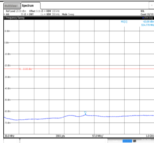
Band66-5MHz-16QAM-131997-1RB#0-30~1000-PASS
