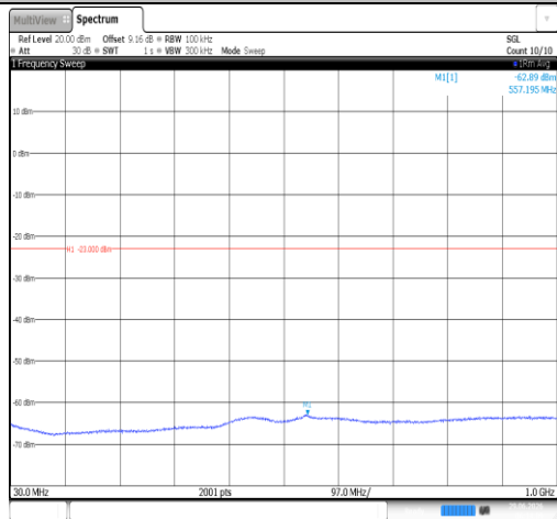
Band66-15MHz-16QAM-132322-1RB#0-30~1000-PASS
