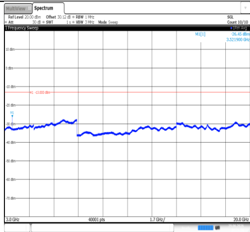
Band66-20MHz-QPSK-132572-1RB#0-3000~20000-PASS
