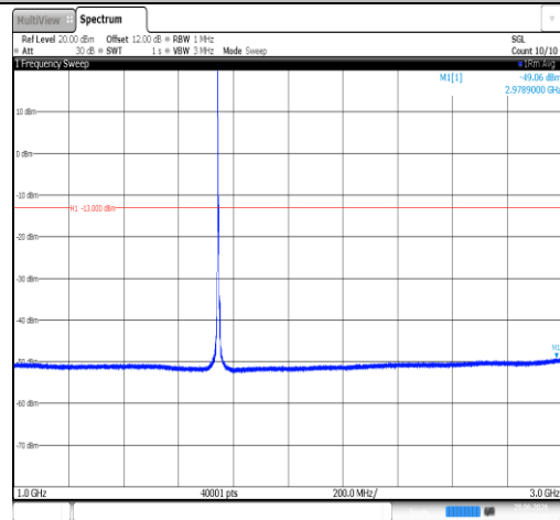
Band66-5MHz-16QAM-132322-1RB#0-1000~3000-PASS
