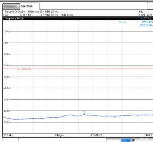
Band66-10MHz-16QAM-132322-1RB#0-30~1000-PASS
