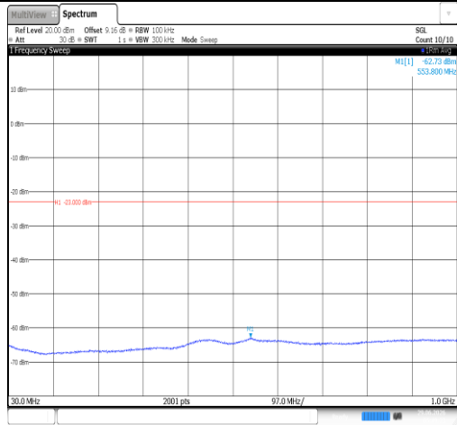
Band66-5MHz-QPSK-131997-1RB#0-30~1000-PASS
