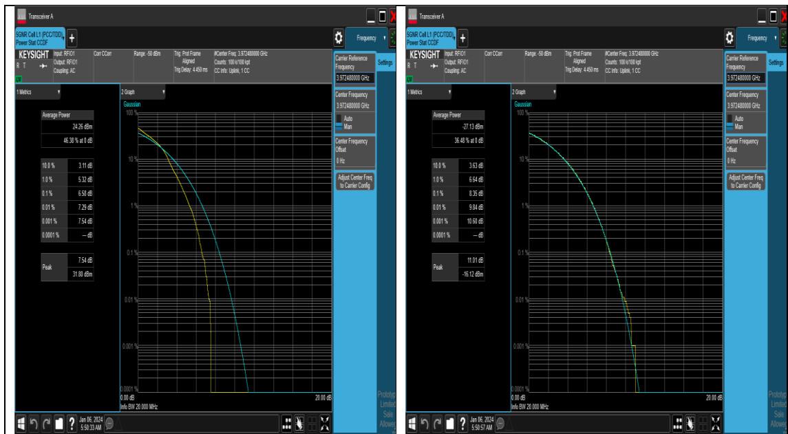
NTNV_N77-3700-3980_PC2_30_15_H_TID3_#1
