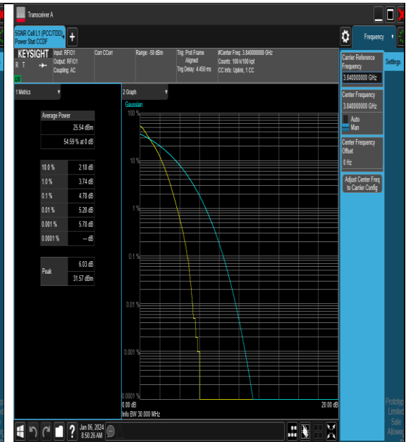
NTNV_N77-3700-3980_PC2_30_30_M_TID1_#1
