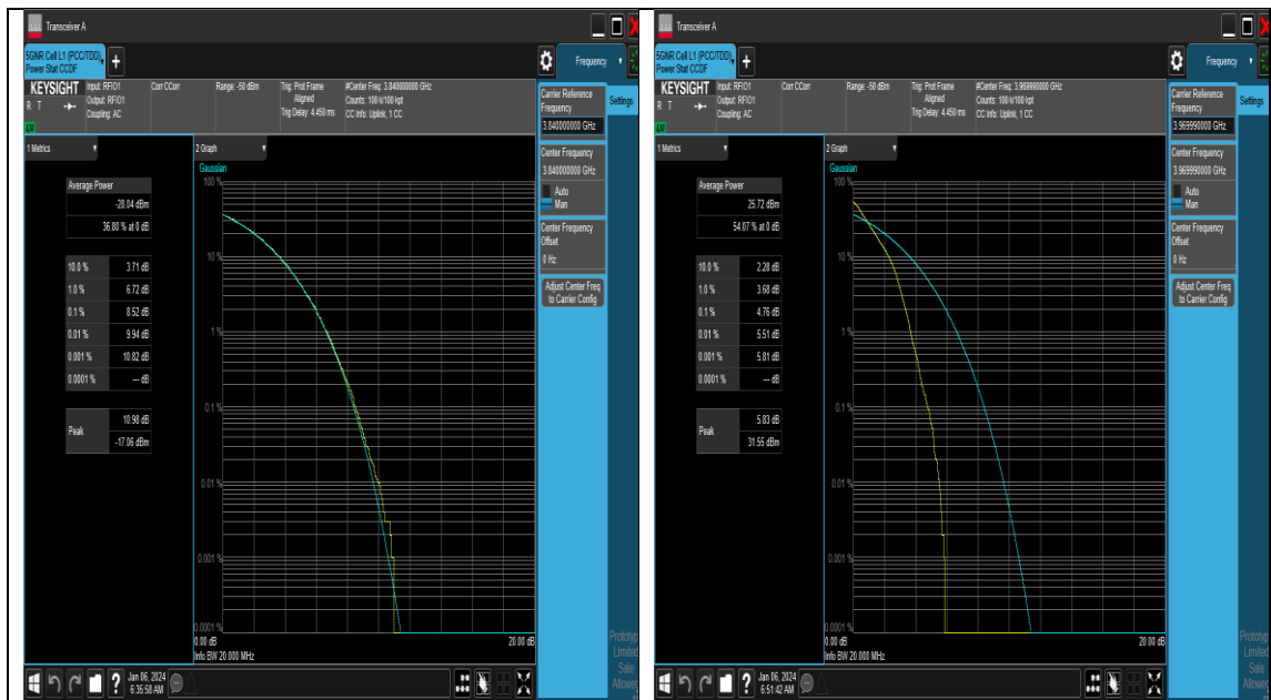
NTNV_N77-3700-3980_PC2_30_20_M_TID4_#1
