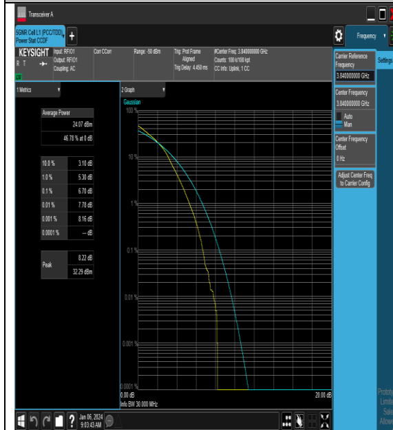
NTNV_N77-3700-3980_PC2_30_30_M_TID3_#1
