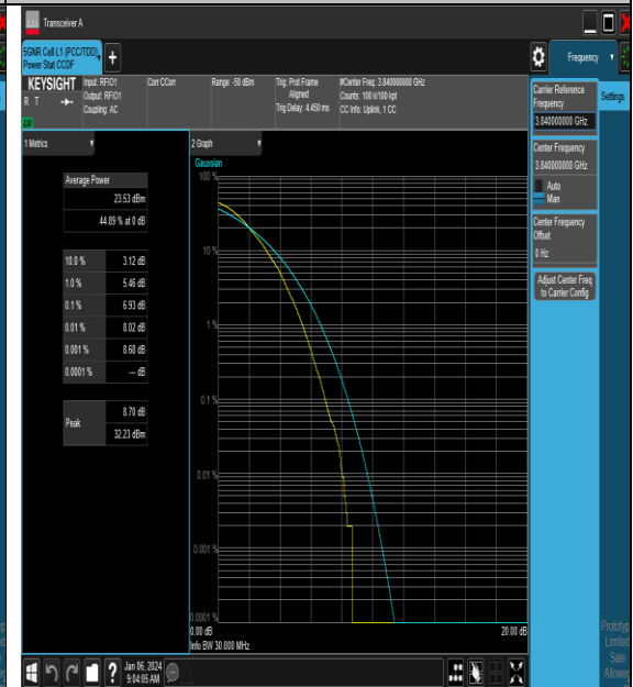
NTNV_N77-3700-3980_PC2_30_30_M_TID4_#1
