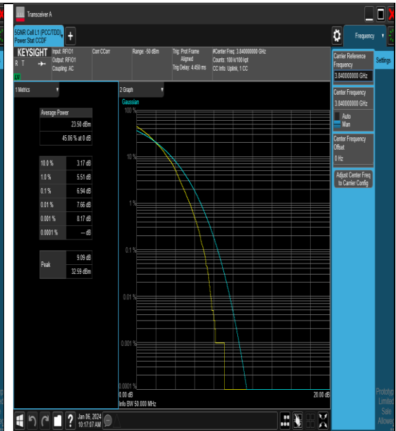
NTNV_N77-3700-3980_PC2_30_40_M_TID4_#1
