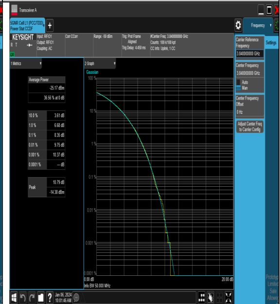
NTNV_N77-3700-3980_PC2_30_40_M_TID1_#1
