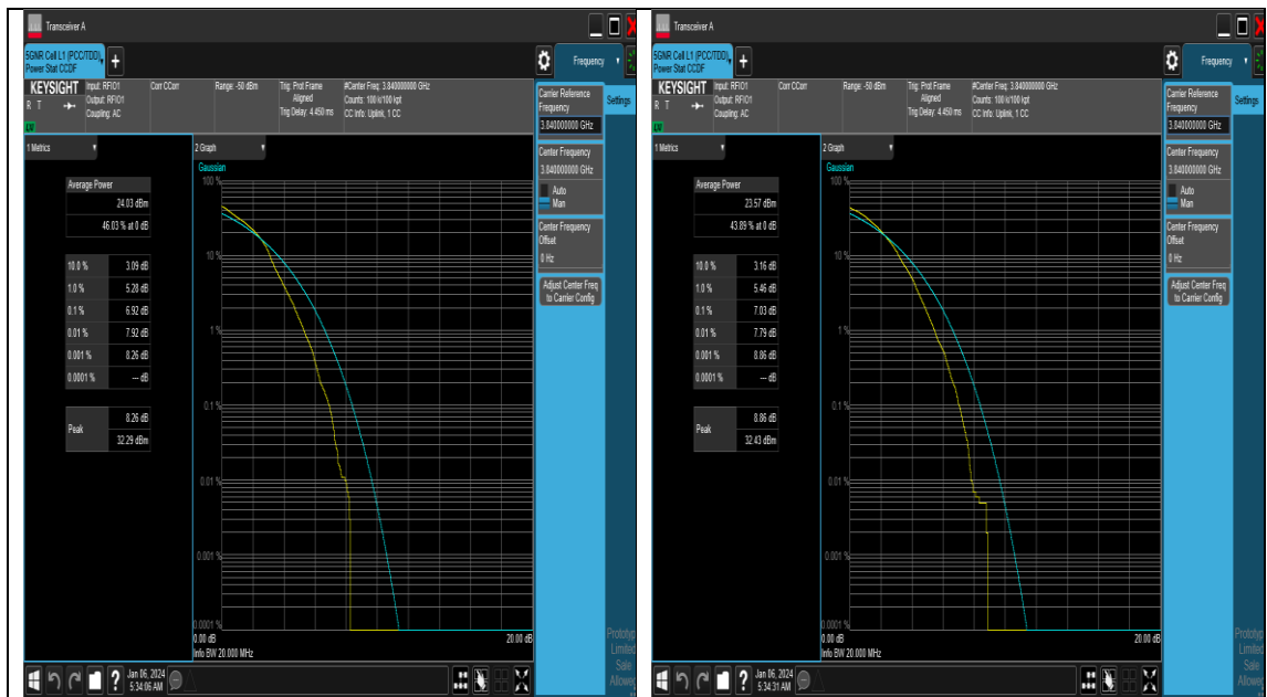
NTNV_N77-3700-3980_PC2_30_15_M_TID3_#1
