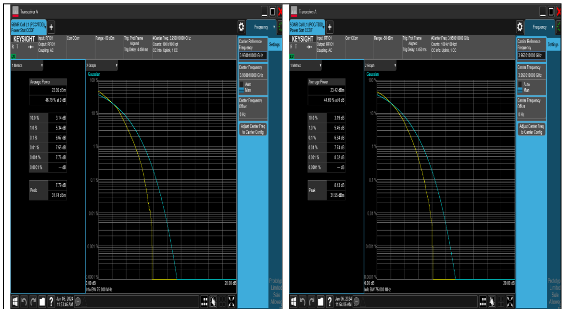
NTNV_N77-3700-3980_PC2_30_60_H_TID3_#1
