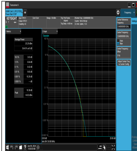
NTNV_N77-3700-3980_PC2_30_30_M_TID5_#1
