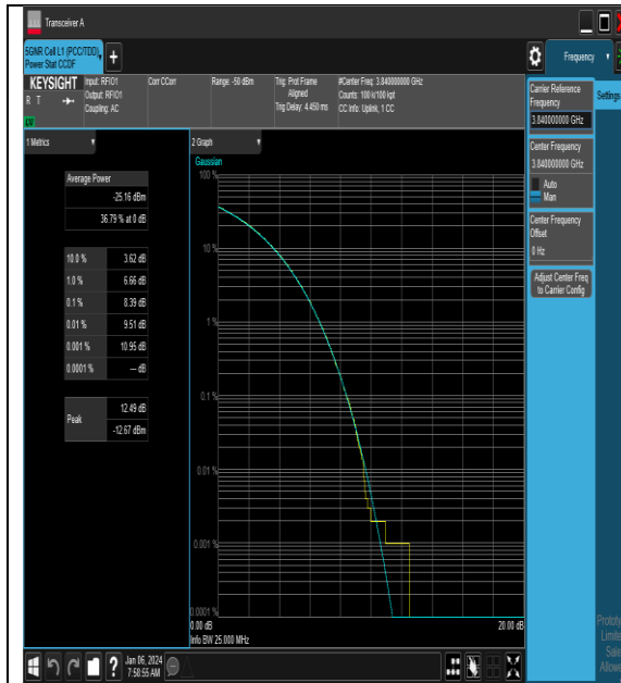
NTNV_N77-3700-3980_PC2_30_25_M_TID5_#1
