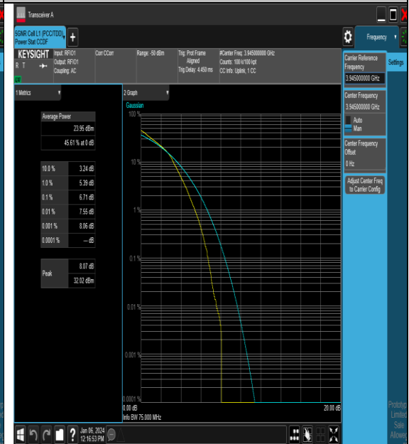
NTNV_N77-3700-3980_PC2_30_70_H_TID3_#1
