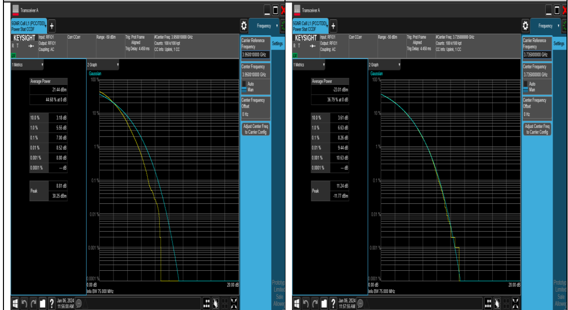
NTNV_N77-3700-3980_PC2_30_60_H_TID5_#1
