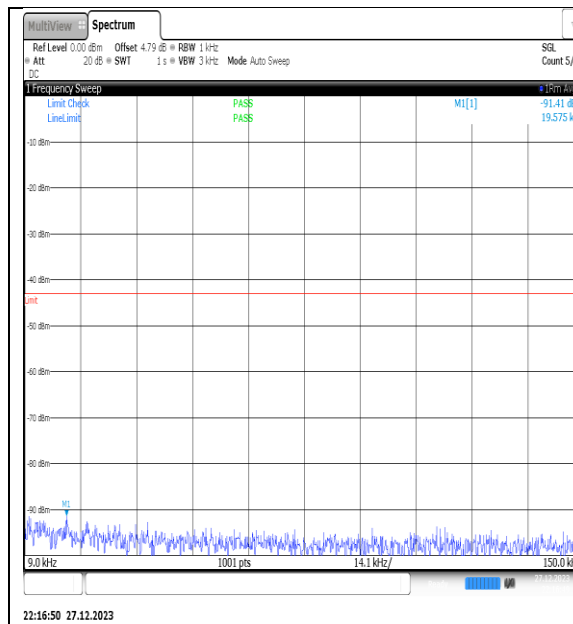
NTNV_N77-3450- 3550_PC2_30_50_H_TID14_NS_01_0.009_0.15_ #1
