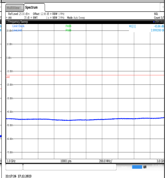
NTNV_N77-3450- 3550_PC2_30_50_H_TID14_NS_01_1000_3000_ #1
