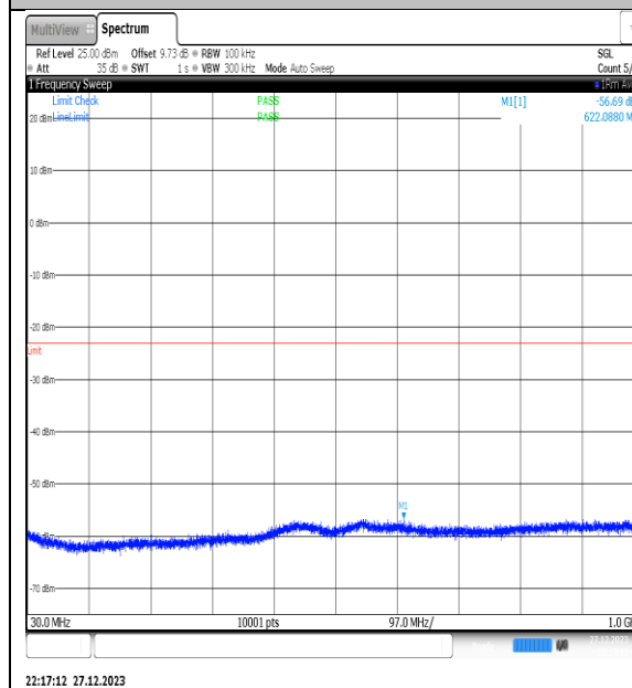
NTNV_N77-3450- 3550_PC2_30_50_H_TID14_NS_01_30_1000_#1
