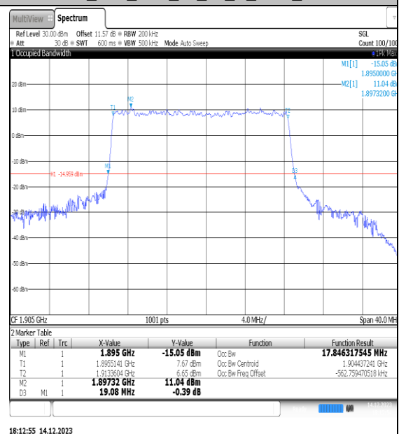
NTNV_N25_PC3_15_20_H_TID4_Ant1#1
