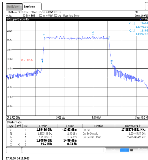
NTNV_N25_PC3_15_20_H_TID1_Ant1#1
