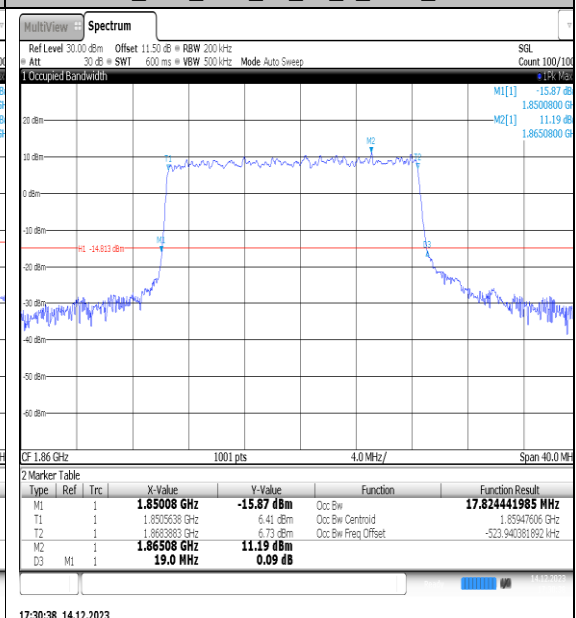
NTNV_N25_PC3_15_20_L_TID4_Ant1#1
