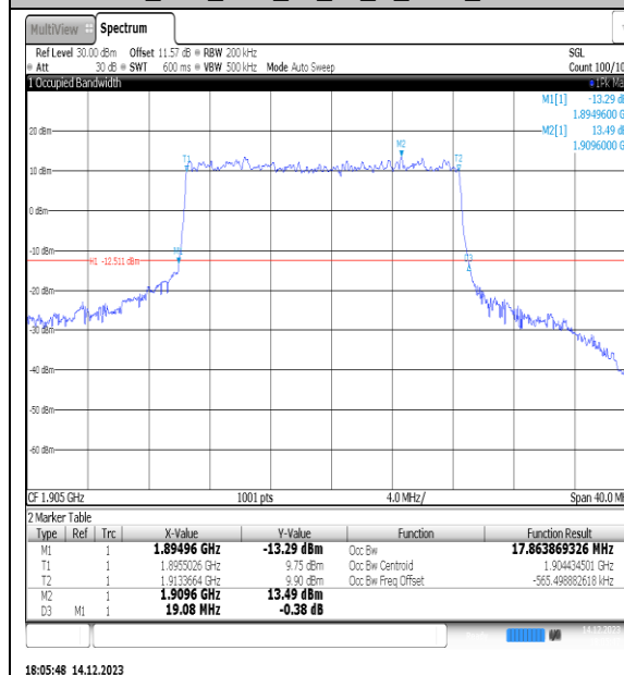
NTNV_N25_PC3_15_20_H_TID3_Ant1#1
