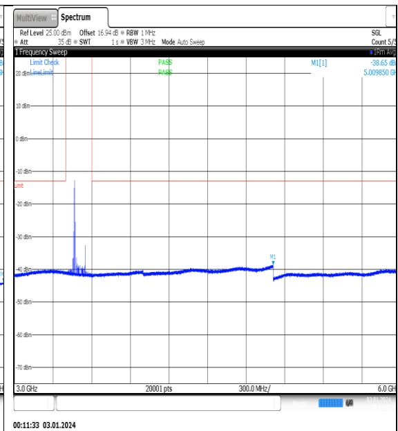
NTNV_N77-3450- 3550_PC2_30_90_H_TID8_NS_01_3000_6000_# 1
