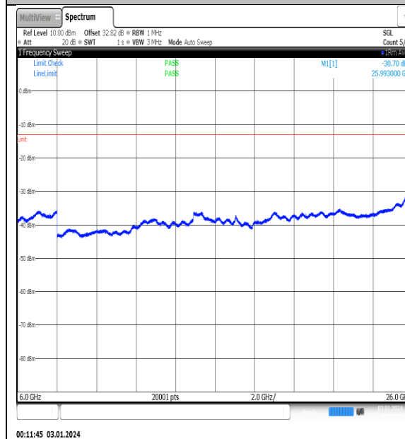
NTNV_N77-3450- 3550_PC2_30_90_H_TID8_NS_01_6000_26000_ #1
