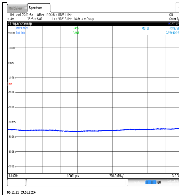
NTNV_N77-3450- 3550_PC2_30_90_H_TID8_NS_01_1000_3000_# 1
