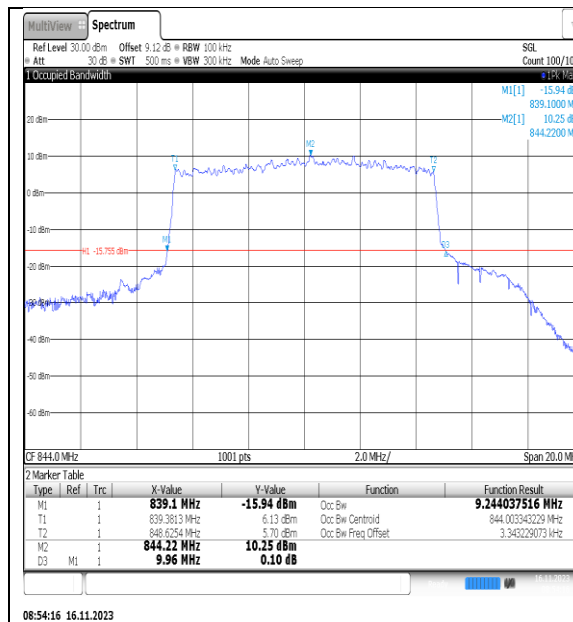
NTNV_N5_PC3_15_10_H_TID8_Ant1#1
