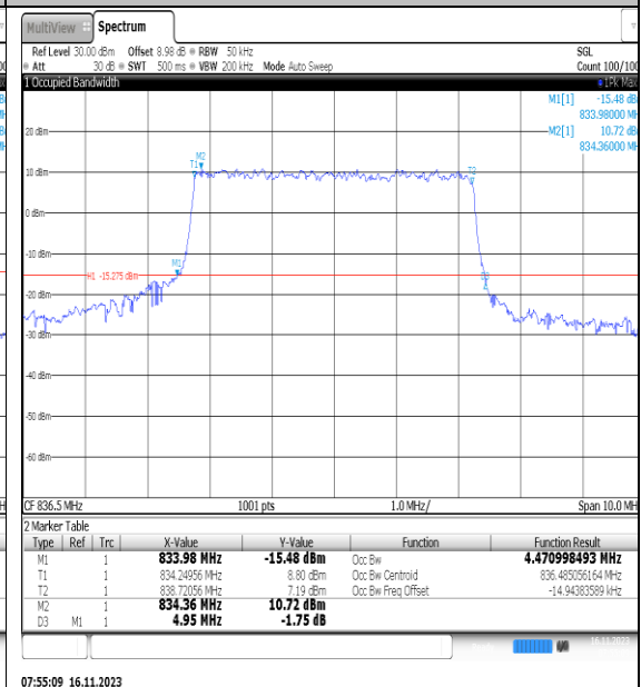
NTNV_N5_PC3_15_5_M_TID7_Ant1#1
