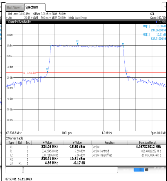
NTNV_N5_PC3_15_5_M_TID5_Ant1#1
