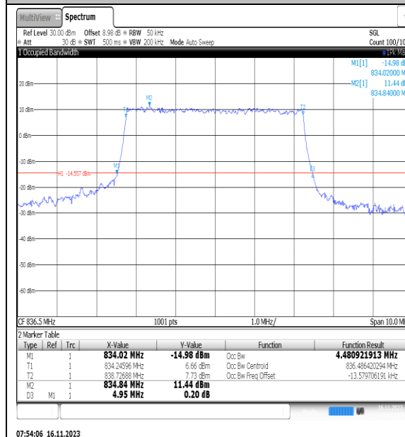
NTNV_N5_PC3_15_5_M_TID6_Ant1#1
