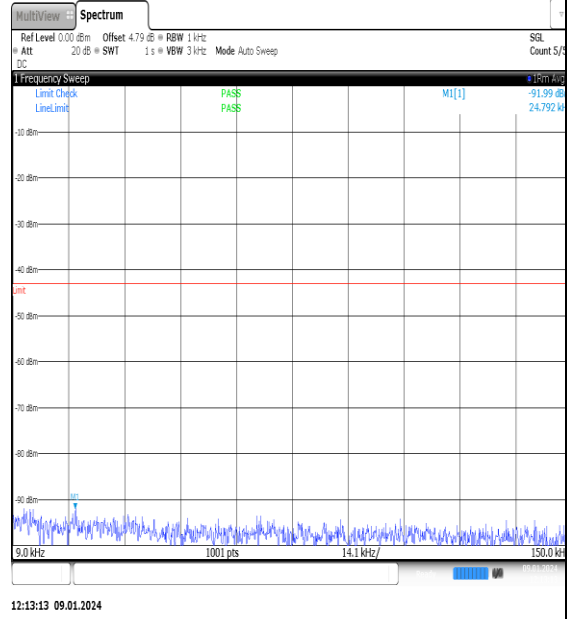
NTNV_N77-3700- 3980_PC2_30_70_L_TID14_NS_01_0.009_0.15_ _#1
