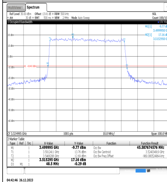
NTNV_N77-3450- 3550_PC2_30_50_H_TID3_Ant1#1
