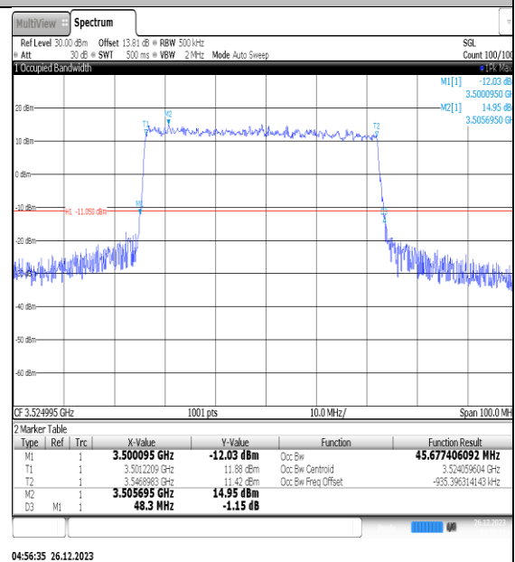
NTNV_N77-3450- 3550_PC2_30_50_H_TID4_Ant1#1
