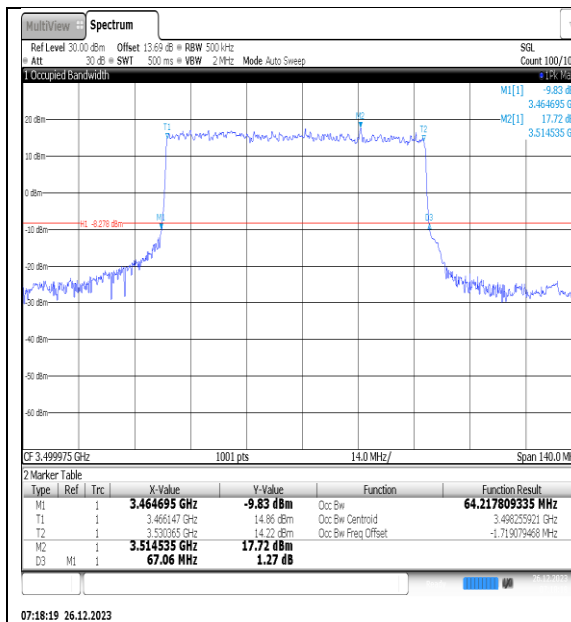
NTNV_N77-3450- 3550_PC2_30_70_M_TID1_Ant1#1
