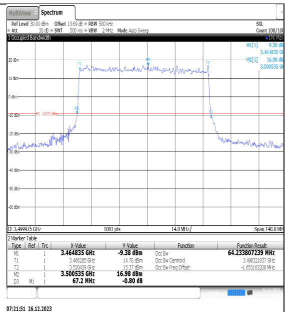
NTNV_N77-3450- 3550_PC2_30_70_M_TID2_Ant1#1
