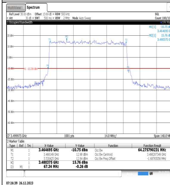
NTNV_N77-3450- 3550_PC2_30_70_M_TID3_Ant1#1
