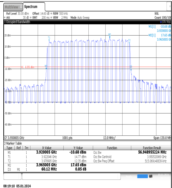
NTNV_N77-3700- 3980_PC2_30_60_H_TID2_Ant1#1
