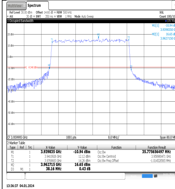
NTNV_N77-3700- 3980_PC2_30_40_H_TID4_Ant1#1
