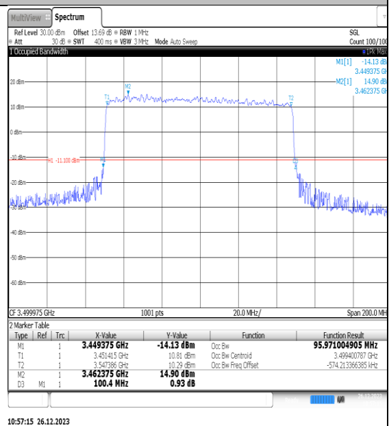
NTNV_N77-3450- 3550_PC2_30_100_M_TID4_Ant1#1
