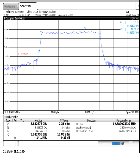
NTNV_N77-3700- 3980_PC2_30_15_M_TID2_Ant1#1
