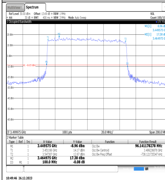
NTNV_N77-3450- 3550_PC2_30_100_M_TID3_Ant1#1
