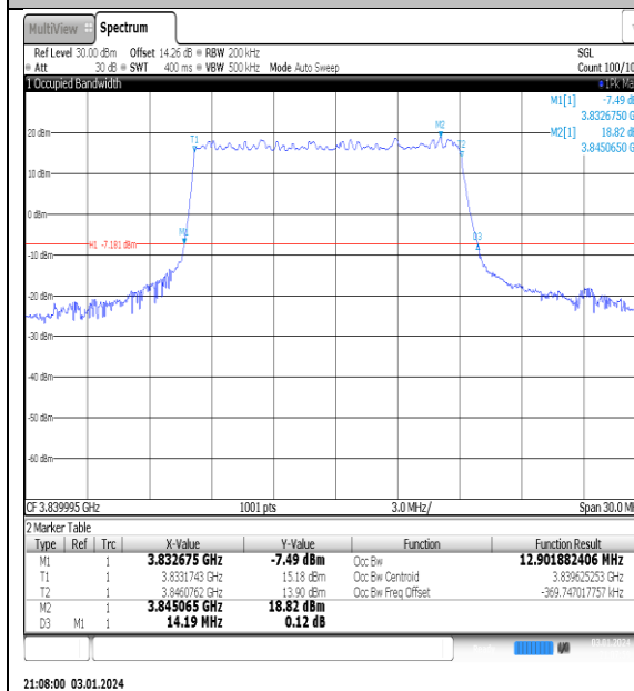
NTNV_N77-3700- 3980_PC2_30_15_M_TID1_Ant1#1
