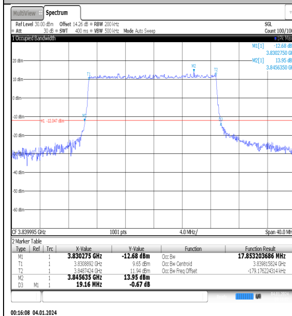
NTNV_N77-3700- 3980_PC2_30_20_M_TID4_Ant1#1
