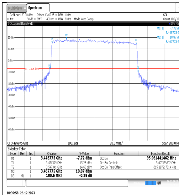
NTNV_N77-3450- 3550_PC2_30_100_M_TID1_Ant1#1
