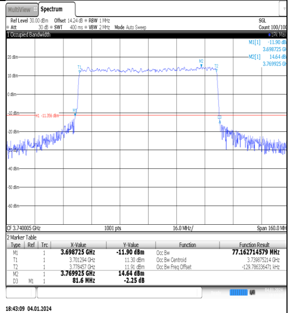
NTNV_N77-3700- 3980_PC2_30_80_L_TID4_Ant1#1
