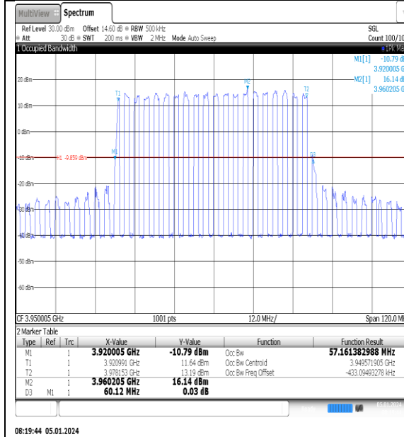
NTNV_N77-3700- 3980_PC2_30_60_H_TID3_Ant1#1
