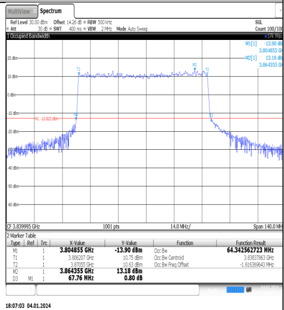
NTNV_N77-3700- 3980_PC2_30_70_M_TID4_Ant1#1
