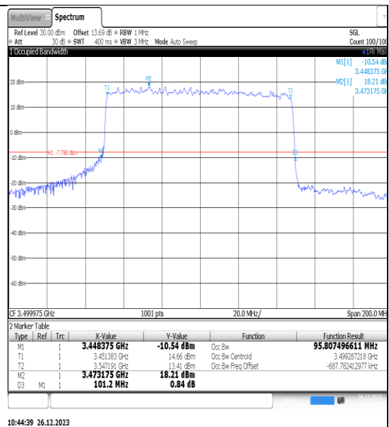
NTNV_N77-3450- 3550_PC2_30_100_M_TID2_Ant1#1
