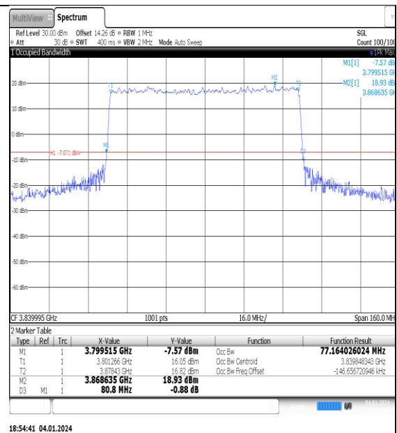
NTNV_N77-3700- 3980_PC2_30_80_M_TID2_Ant1#1
