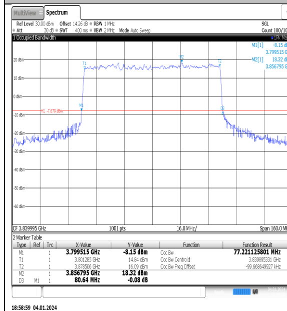
NTNV_N77-3700- 3980_PC2_30_80_M_TID3_Ant1#1
