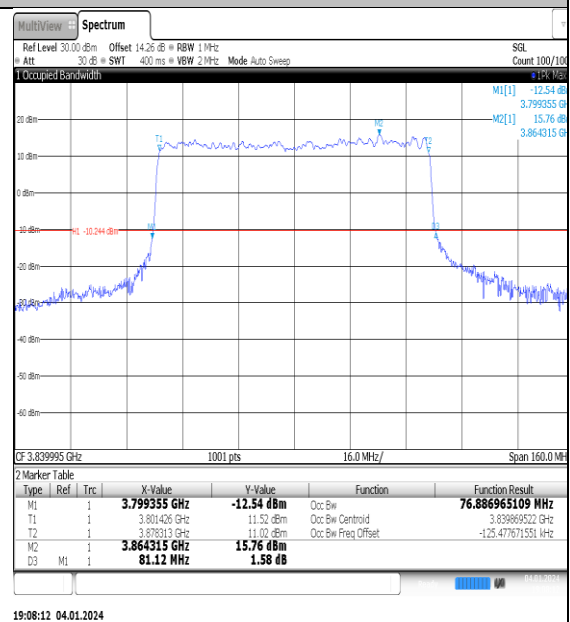
NTNV_N77-3700- 3980_PC2_30_80_M_TID4_Ant1#1
