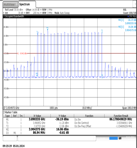
NTNV_N77-3700- 3980_PC2_30_90_H_TID4_Ant1#1
