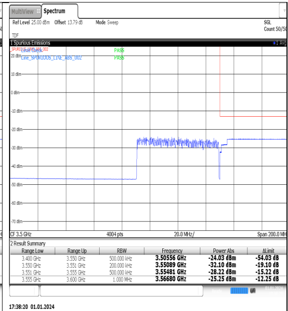
NTNV_N77-3450-3550_PC2_30_60_H_TID13_#1
