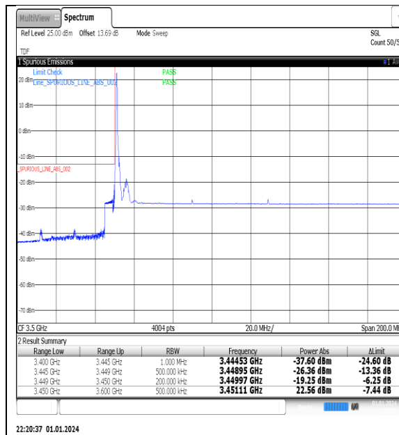
NTNV_N77-3450-3550_PC2_30_80_L_TID14_#1
