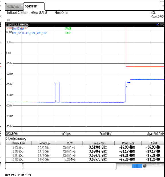
NTNV_N77-3450-3550_PC2_30_90_H_TID6_#1
