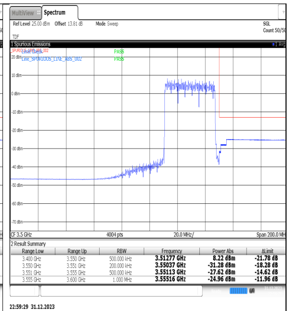
NTNV_N77-3450-3550_PC2_30_40_H_TID13_#1
