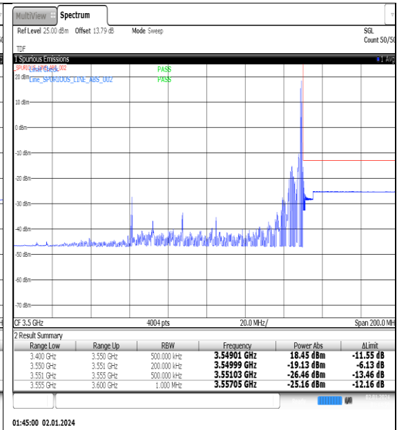
NTNV_N77-3450-3550_PC2_30_90_H_TID3_#1
