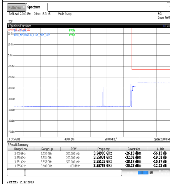
NTNV_N77-3450-3550_PC2_30_40_H_TID15_#1
