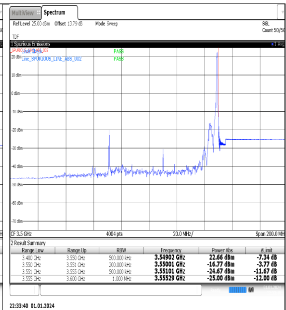
NTNV_N77-3450-3550_PC2_30_80_H_TID3_#1
