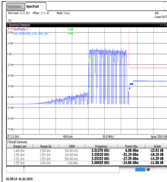
NTNV_N77-3450-3550_PC2_30_50_H_TID10_#1
