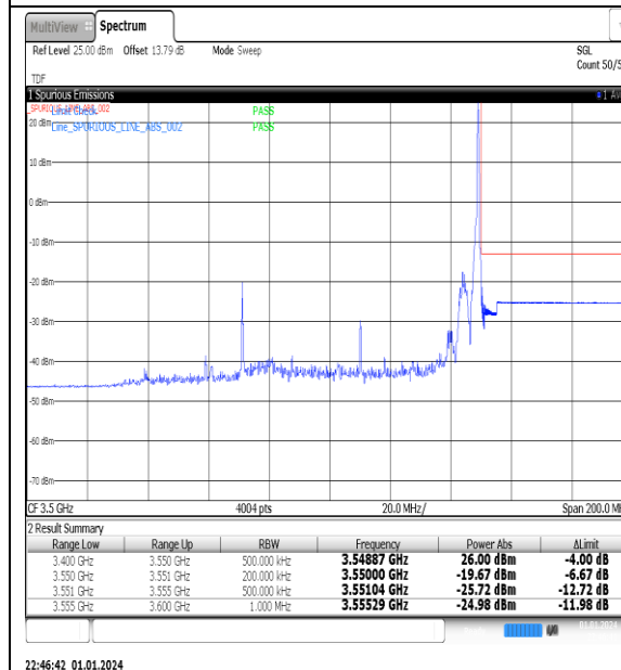
NTNV_N77-3450-3550_PC2_30_80_H_TID6_#1
