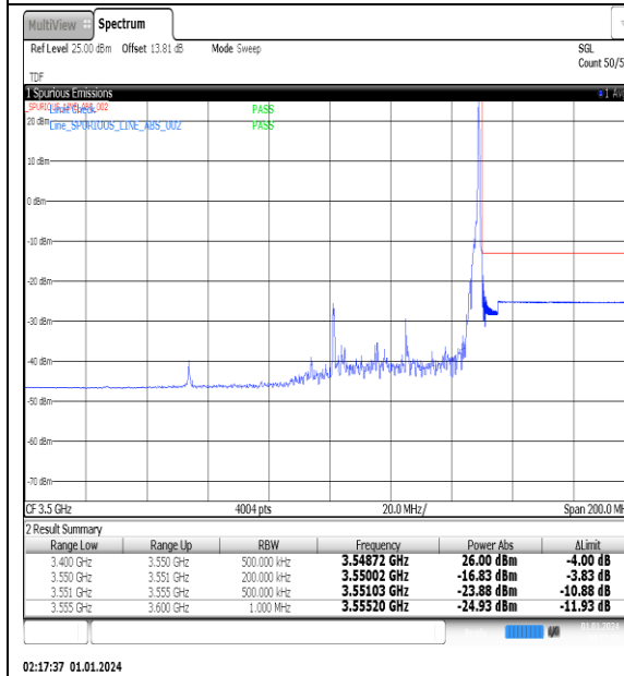
NTNV_N77-3450-3550_PC2_30_50_H_TID15_#1
