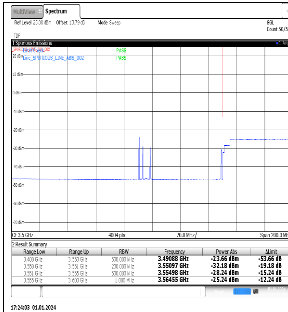
NTNV_N77-3450-3550_PC2_30_60_H_TID12_#1
