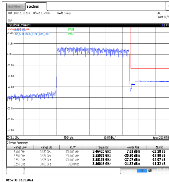
NTNV_N77-3450-3550_PC2_30_90_H_TID4_#1
