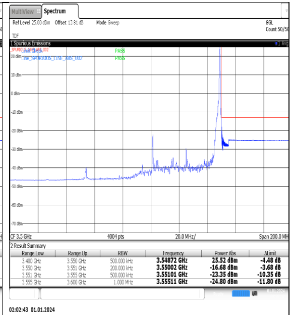
NTNV_N77-3450-3550_PC2_30_50_H_TID12_#1
