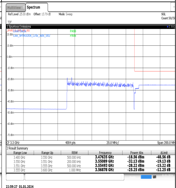
NTNV_N77-3450-3550_PC2_30_80_H_TID7_#1
