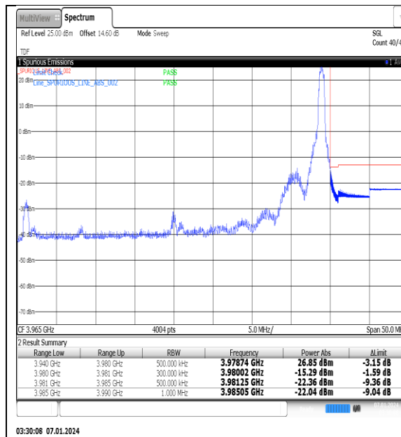
NTNV_N77-3700-3980_PC2_30_40_H_TID12_#1
