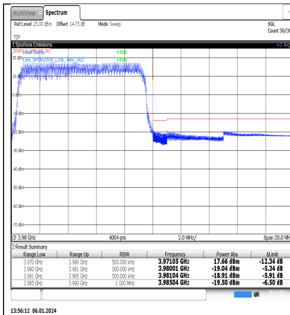
NTNV_N77-3700-3980_PC2_30_10_H_TID4_#1
