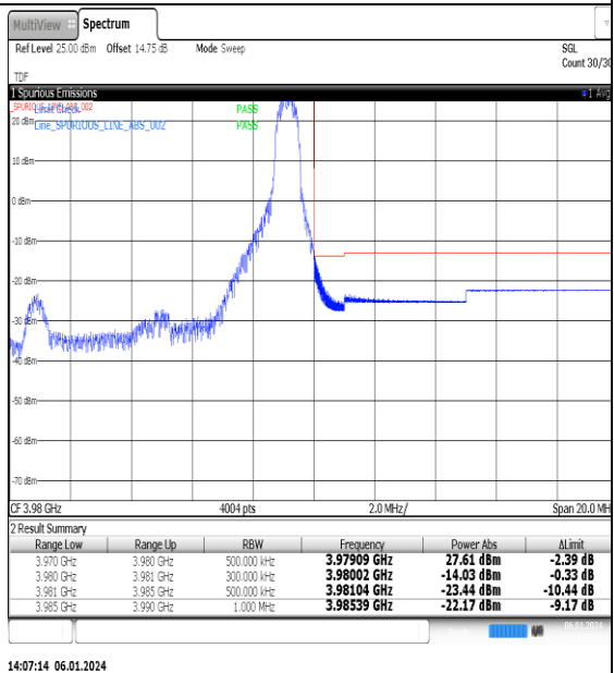
NTNV_N77-3700-3980_PC2_30_10_H_TID9_#1
