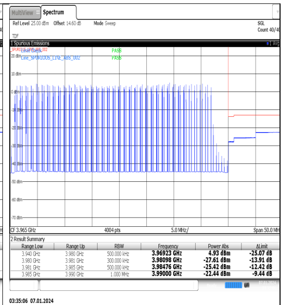
NTNV_N77-3700-3980_PC2_30_40_H_TID13_#1
