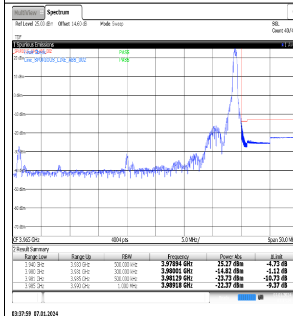
NTNV_N77-3700-3980_PC2_30_40_H_TID15_#1
