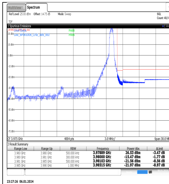
NTNV_N77-3700-3980_PC2_30_20_H_TID15_#1
