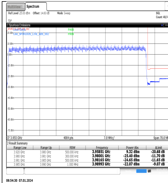
NTNV_N77-3700-3980_PC2_30_60_H_TID10_#1
