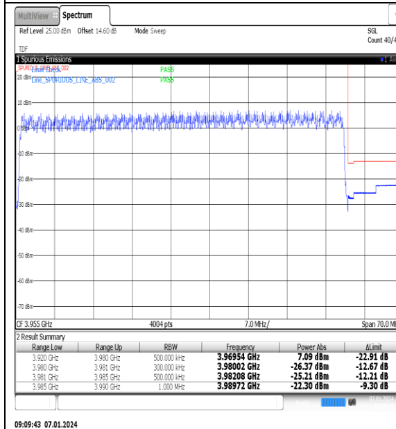
NTNV_N77-3700-3980_PC2_30_60_H_TID13_#1
