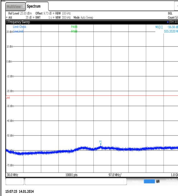
NTNV_N25_PC3_15_5_H_TID3_NS_01_30_1000 _#1
