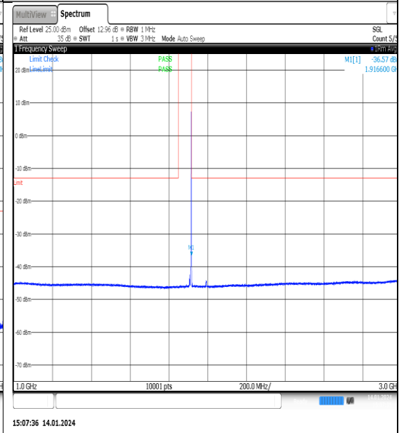
NTNV_N25_PC3_15_5_H_TID3_NS_01_1000_30 00_#1
