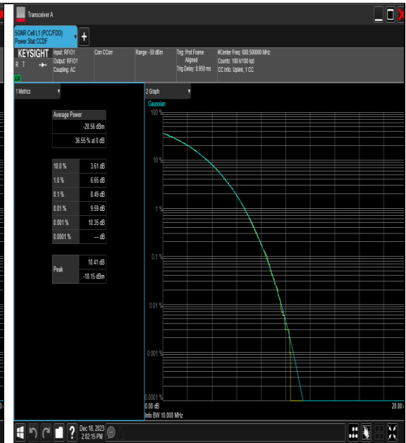
NTNV_N71_PC3_15_10_M_TID4_#1
