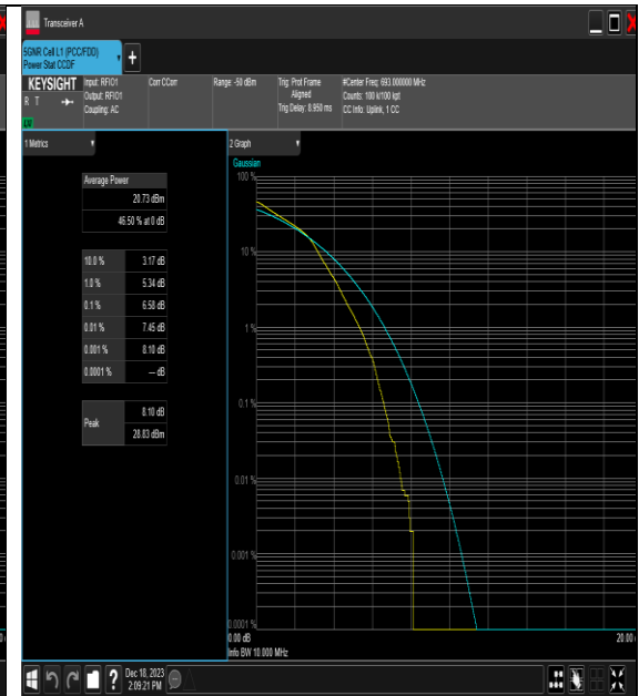
NTNV_N71_PC3_15_10_H_TID3_#1
