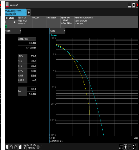
NTNV_N71_PC3_15_10_H_TID5_#1
