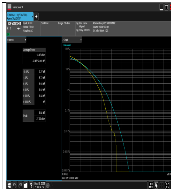
NTNV_N71_PC3_15_5_H_TID5_#1
