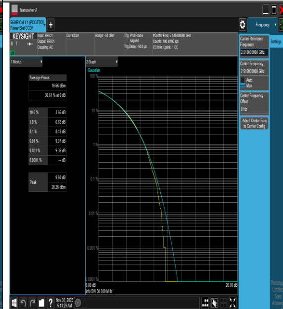
NTNV_N7_PC3_15_30_L_TID8_#1
