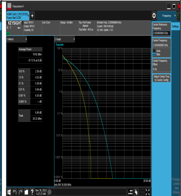
NTNV_N7_PC3_15_30_H_TID2_#1
