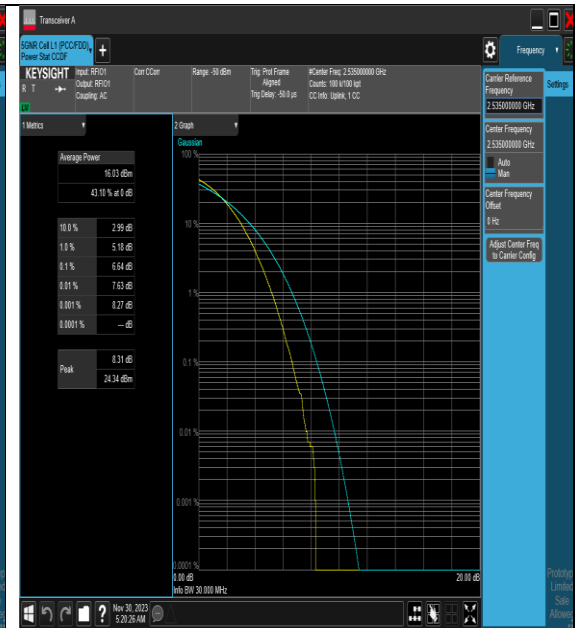
NTNV_N7_PC3_15_30_M_TID5_#1
