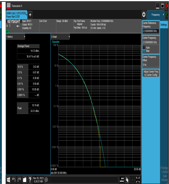
NTNV_N7_PC3_15_30_M_TID9_#1
