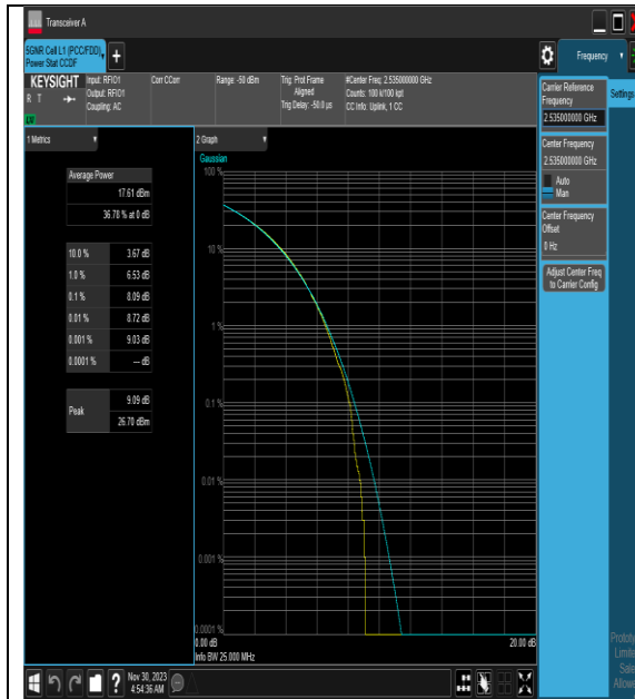
NTNV_N7_PC3_15_25_M_TID7_#1
