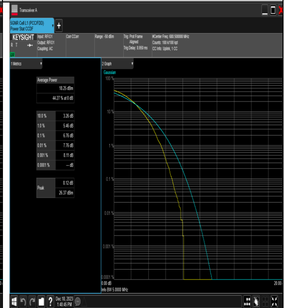
NTNV_N71_PC3_15_5_M_TID5_#1
