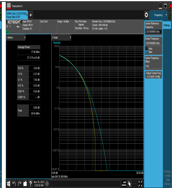
NTNV_N7_PC3_15_25_H_TID7_#1
