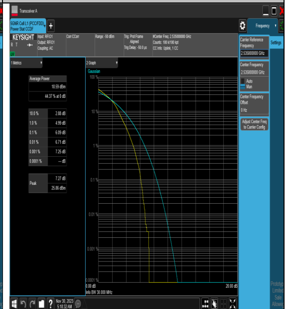
NTNV_N7_PC3_15_30_M_TID3_#1
