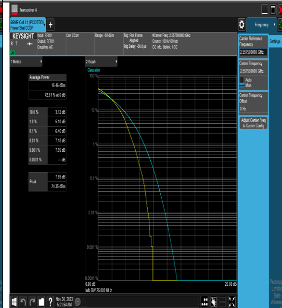
NTNV_N7_PC3_15_25_H_TID5_#1
