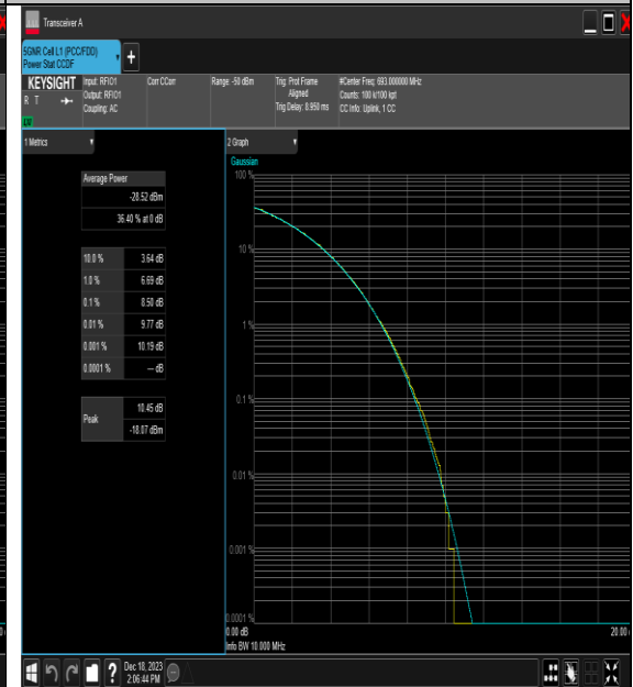
NTNV_N71_PC3_15_10_H_TID1_#1
