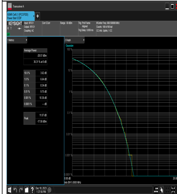
NTNV_N71_PC3_15_5_M_TID4_#1
