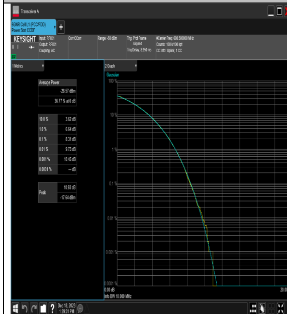
NTNV_N71_PC3_15_10_M_TID1_#1
