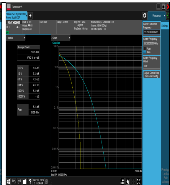
NTNV_N7_PC3_15_30_M_TID1_#1
