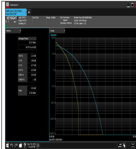
NTNV_N71_PC3_15_5_H_TID1_#1
