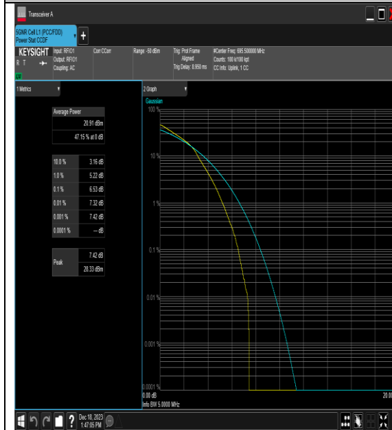
NTNV_N71_PC3_15_5_H_TID3_#1
