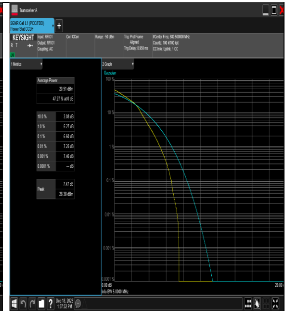
NTNV_N71_PC3_15_5_M_TID3_#1
