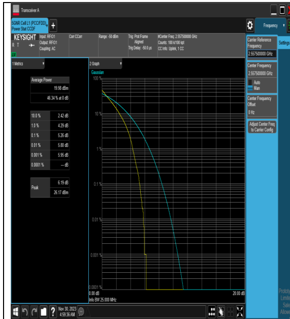
NTNV_N7_PC3_15_25_H_TID2_#1
