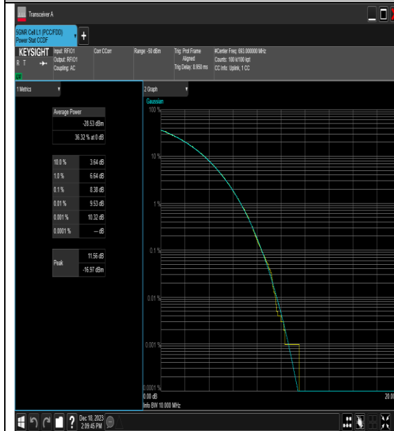
NTNV_N71_PC3_15_10_H_TID4_#1
