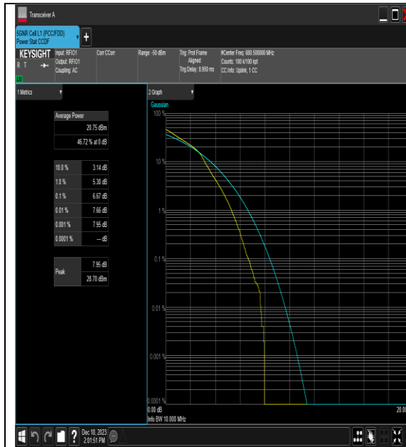
NTNV_N71_PC3_15_10_M_TID3_#1
