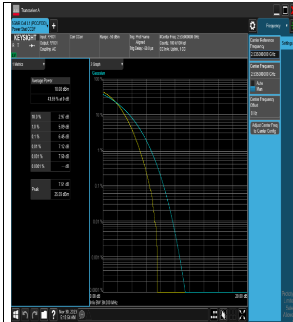
NTNV_N7_PC3_15_30_M_TID4_#1
