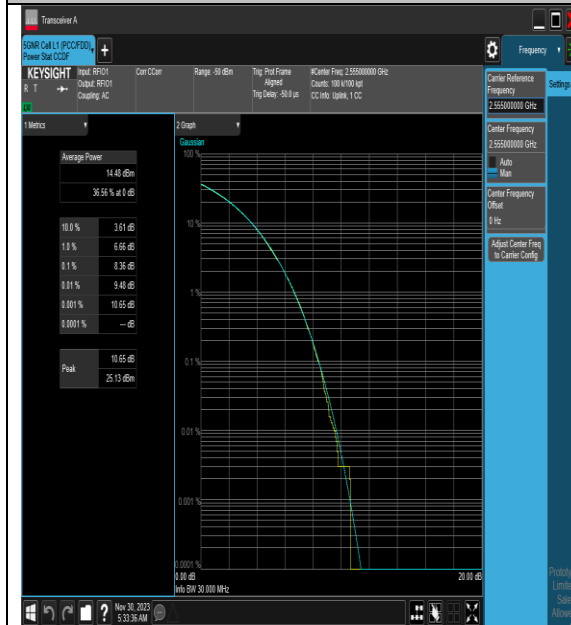
NTNV_N7_PC3_15_30_H_TID9_#1
