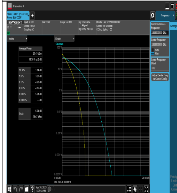
NTNV_N7_PC3_15_30_H_TID1_#1
