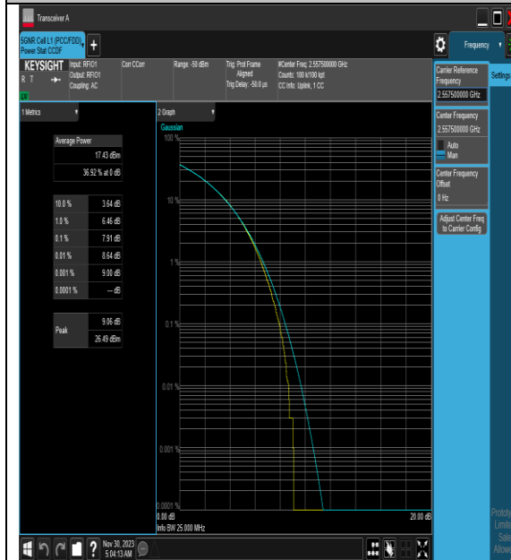
NTNV_N7_PC3_15_25_H_TID8_#1
