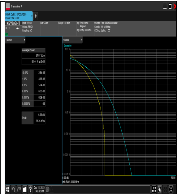
NTNV_N71_PC3_15_5_H_TID2_#1
