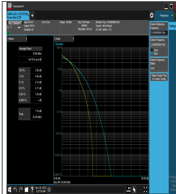
NTNV_N7_PC3_15_30_H_TID3_#1
