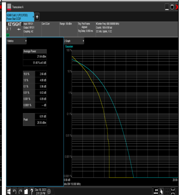
NTNV_N71_PC3_15_10_M_TID2_#1
