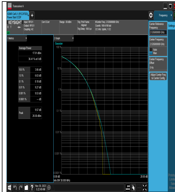
NTNV_N7_PC3_15_30_M_TID8_#1
