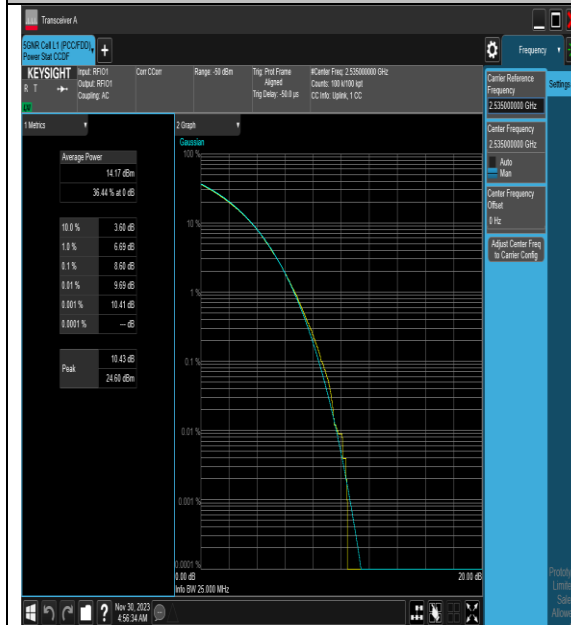
NTNV_N7_PC3_15_25_M_TID9_#1
