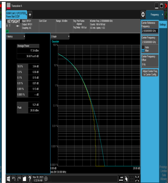
NTNV_N7_PC3_15_30_H_TID8_#1
