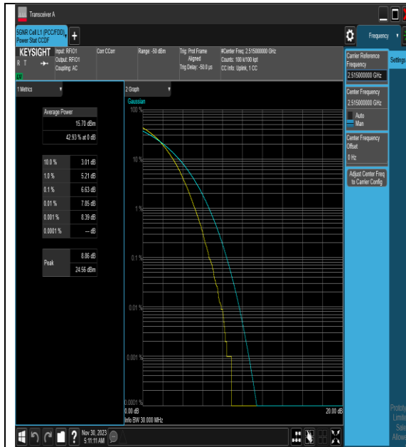
NTNV_N7_PC3_15_30_L_TID5_#1
