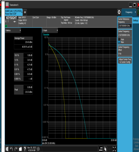
NTNV_N7_PC3_15_25_H_TID1_#1
