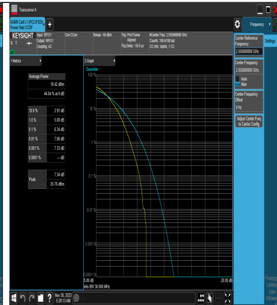
NTNV_N7_PC3_15_30_H_TID4_#1
