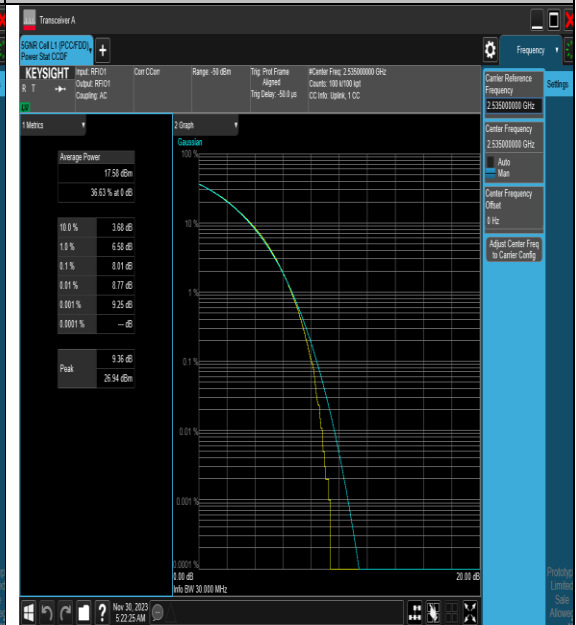
NTNV_N7_PC3_15_30_M_TID7_#1
