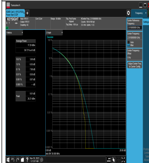
NTNV_N7_PC3_15_30_L_TID7_#1
