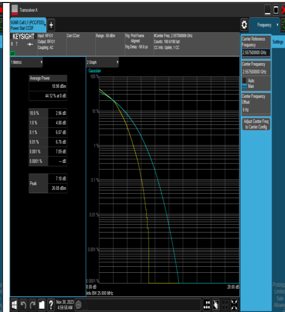
NTNV_N7_PC3_15_25_H_TID3_#1
