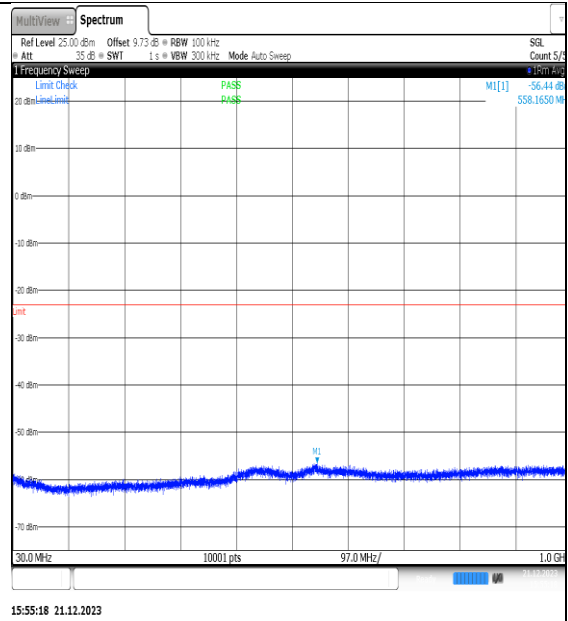
NTNV_N66_PC3_15_40_M_TID4_NS_01_30_10 00_#1
