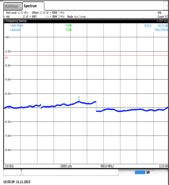
NTNV_N66_PC3_15_40_M_TID4_NS_01_3000_12000_#1
