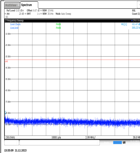
NTNV_N66_PC3_15_40_M_TID4_NS_01_0.15_3 0_#1
