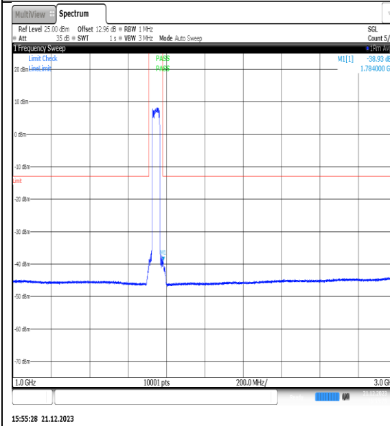
NTNV_N66_PC3_15_40_M_TID4_NS_01_1000_3000_#1
